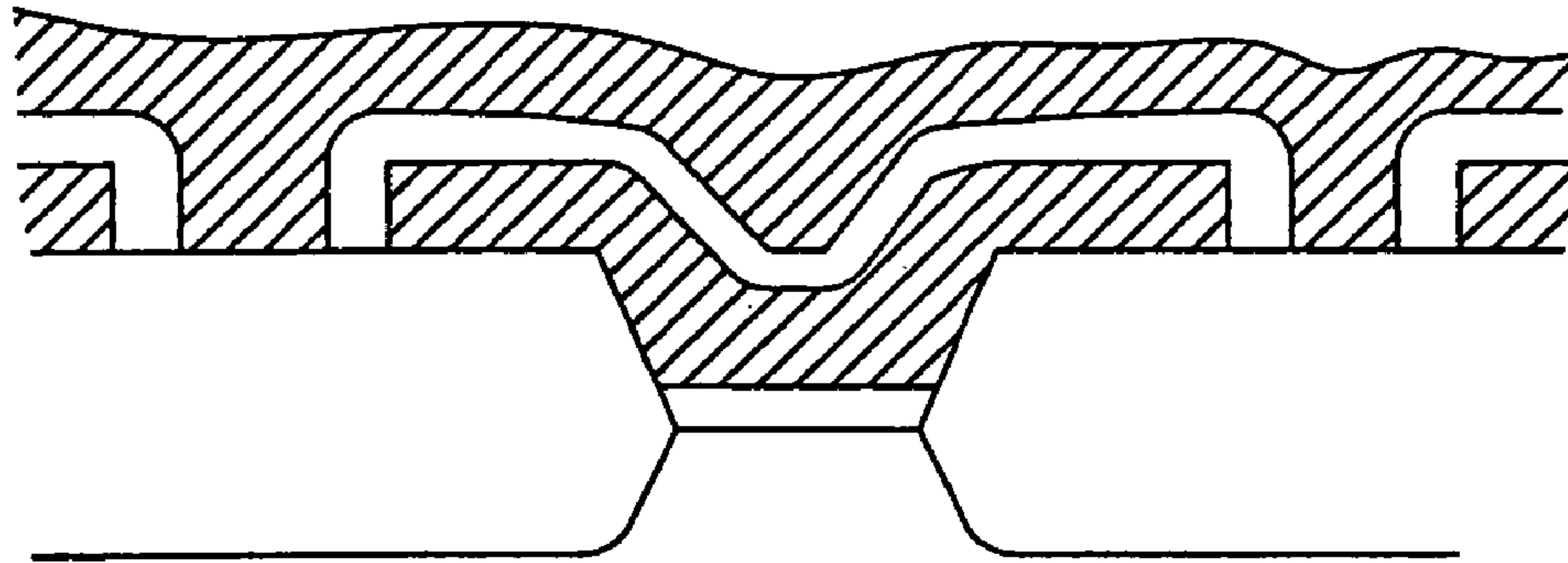
FIG. 4. (PRIOR ART)
