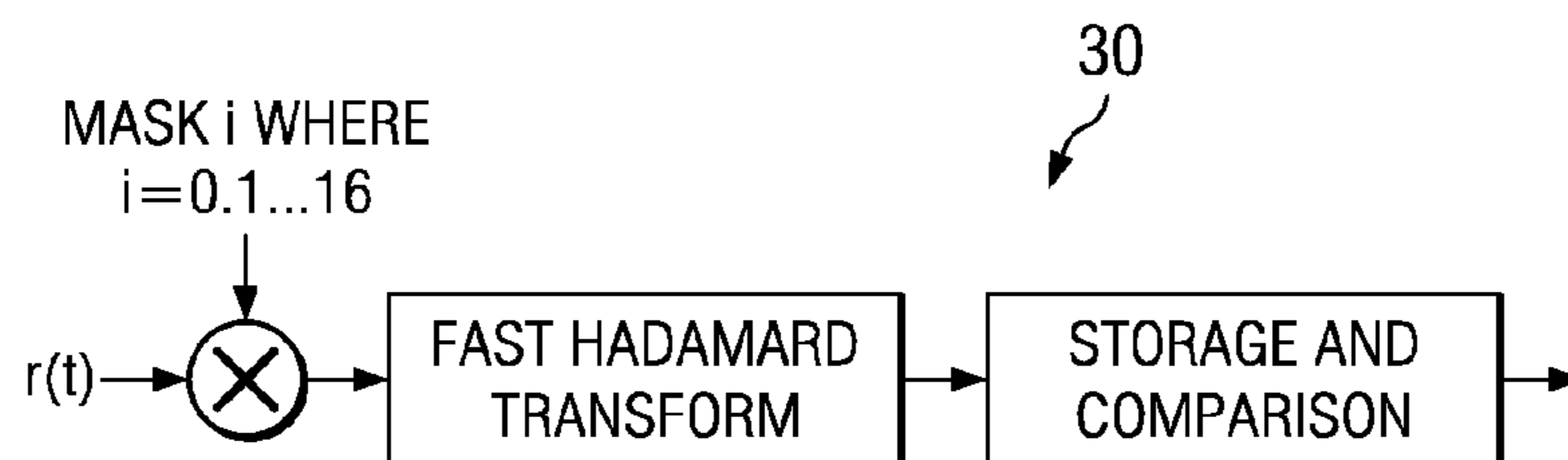
FIG. 3 (PRIOR ART)
