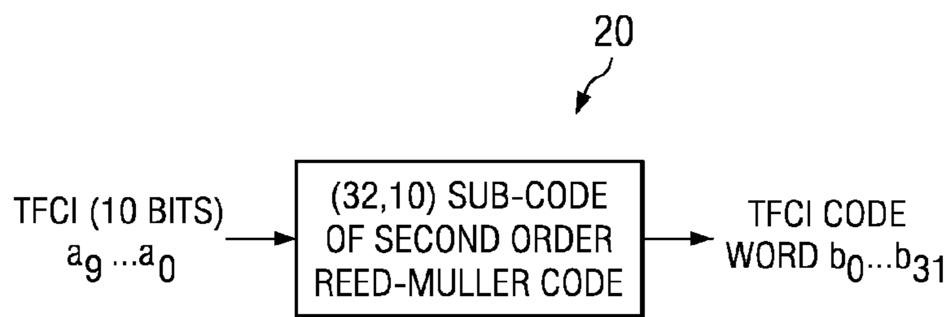
FIG. 2 (PRIOR ART)
