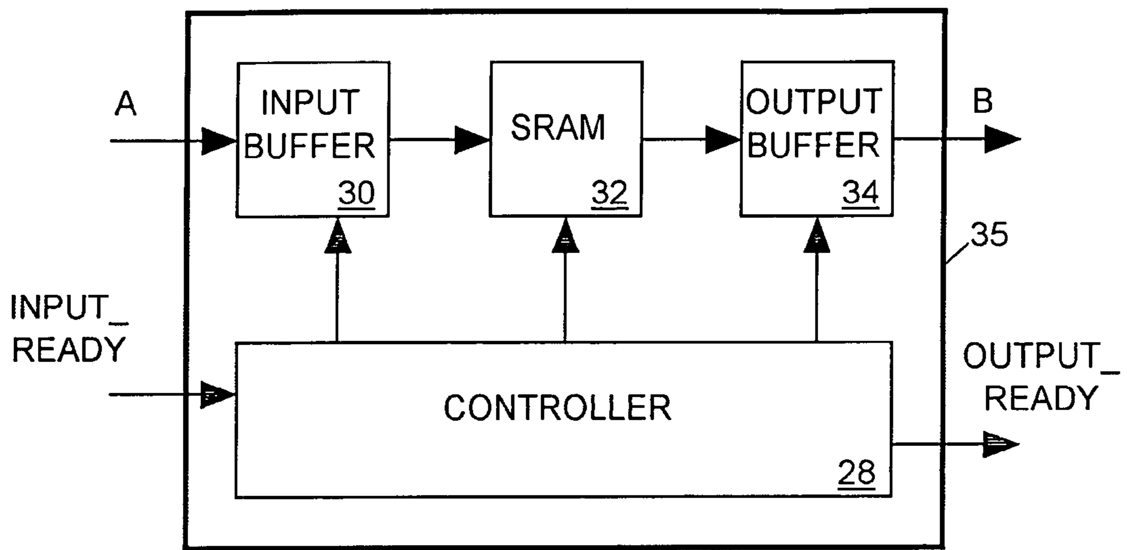
FIG. 3 (PRIOR ART)
