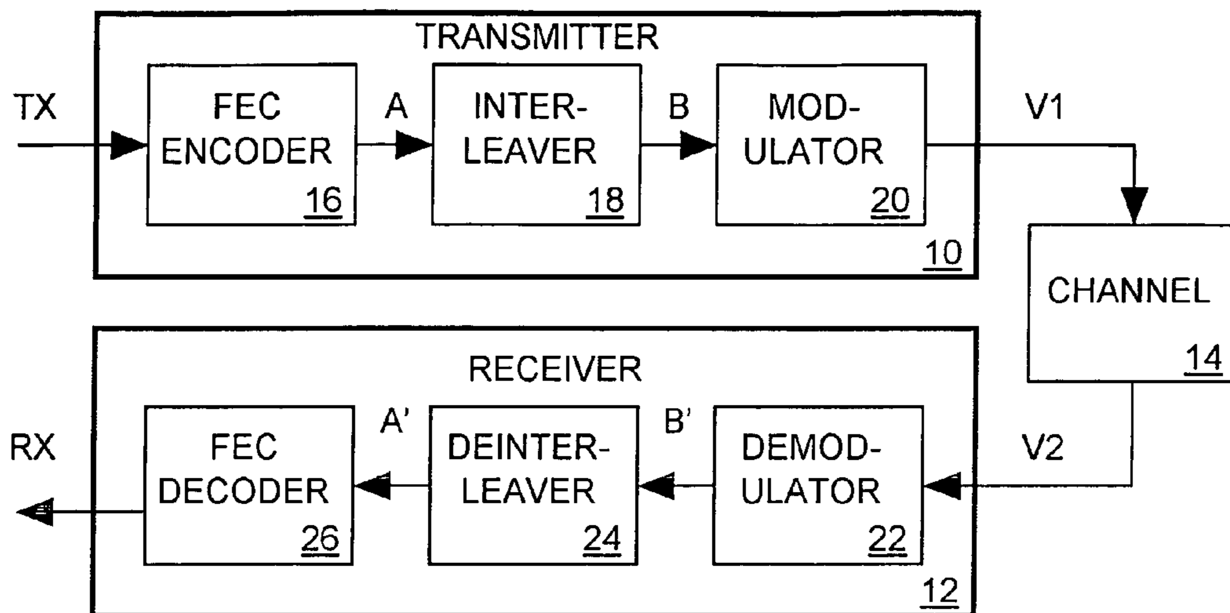
FIG. 1 (PRIOR ART)
