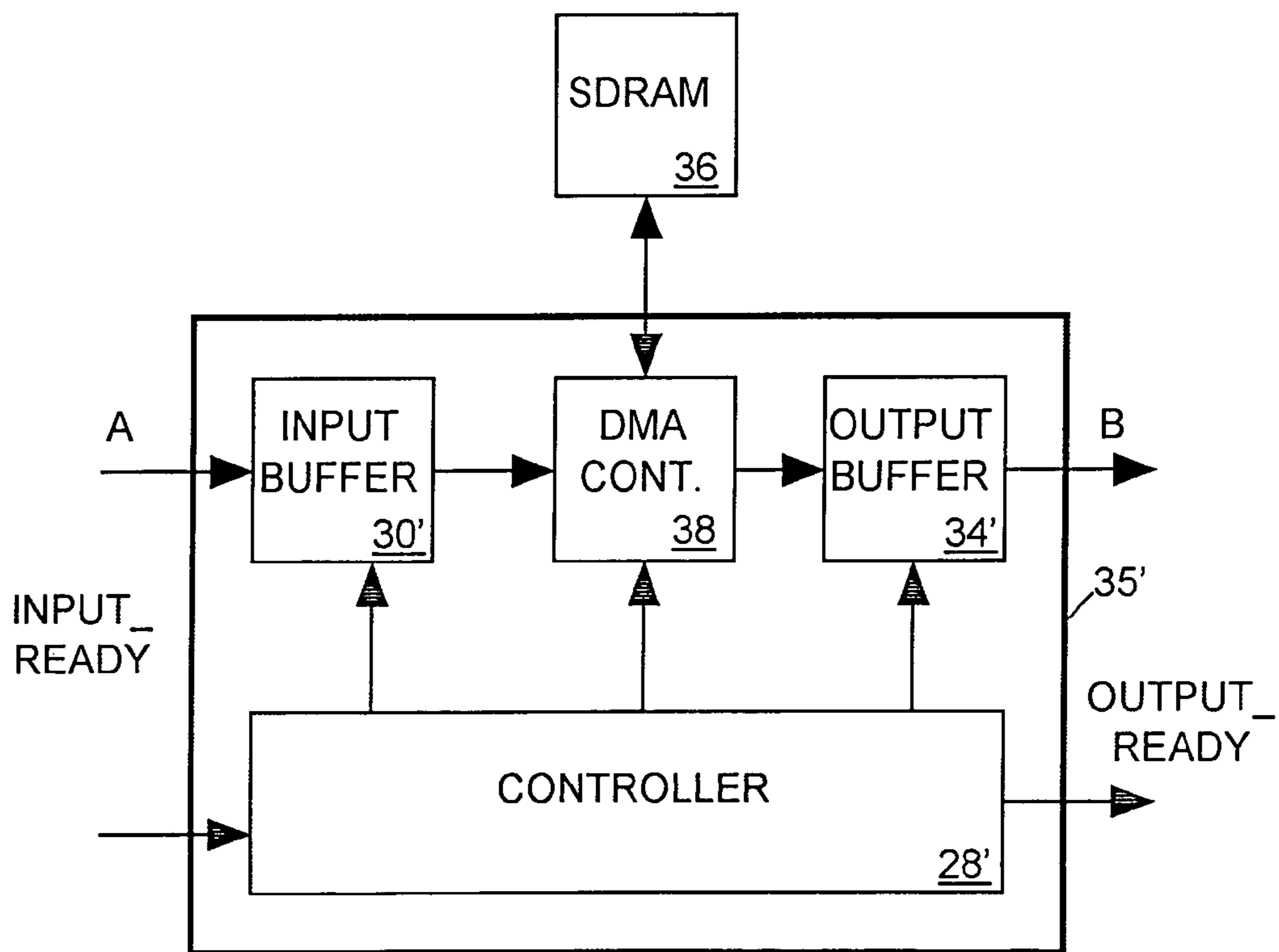
FIG. 4 (PRIOR ART)
