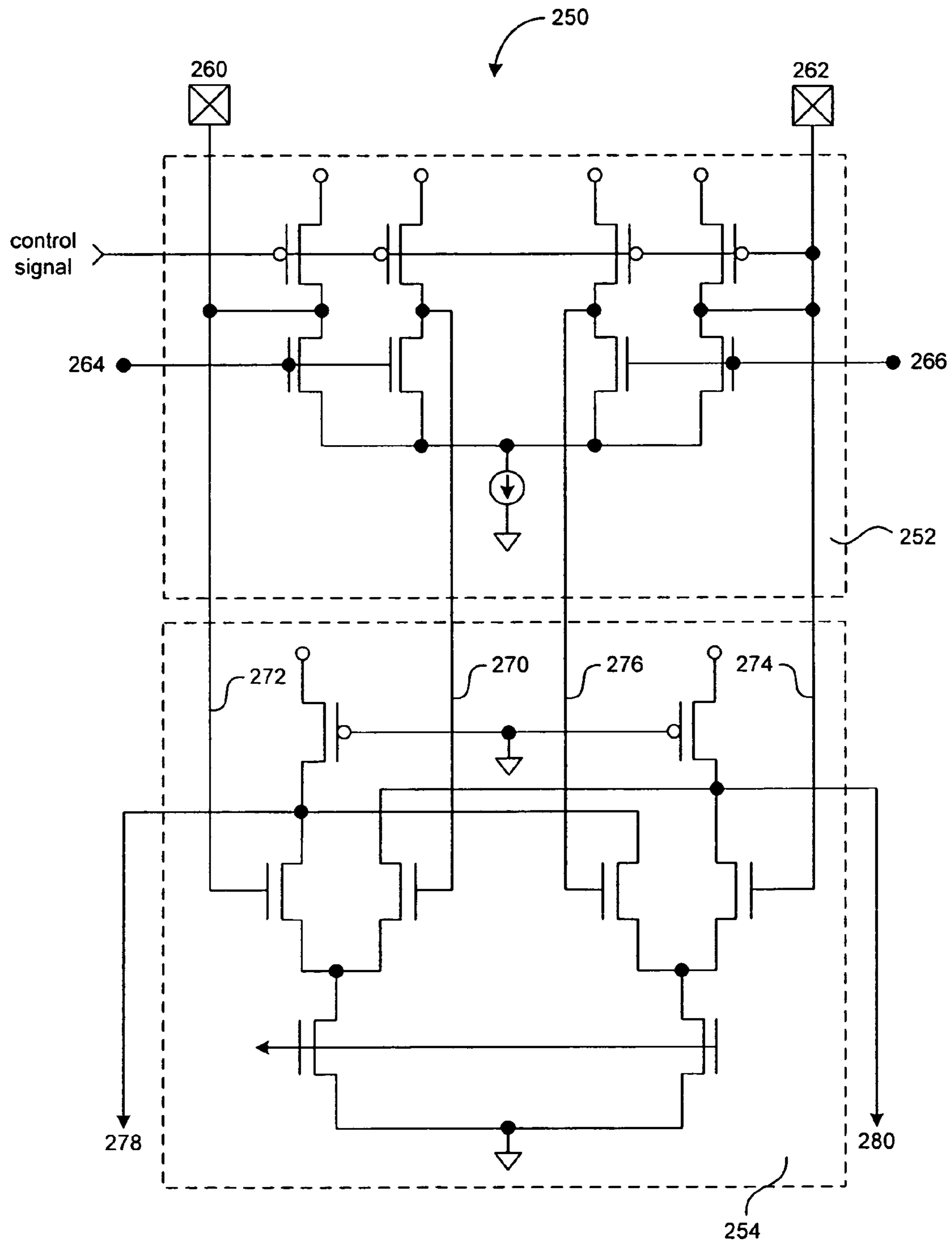
FIG. 2 (Prior Art)
