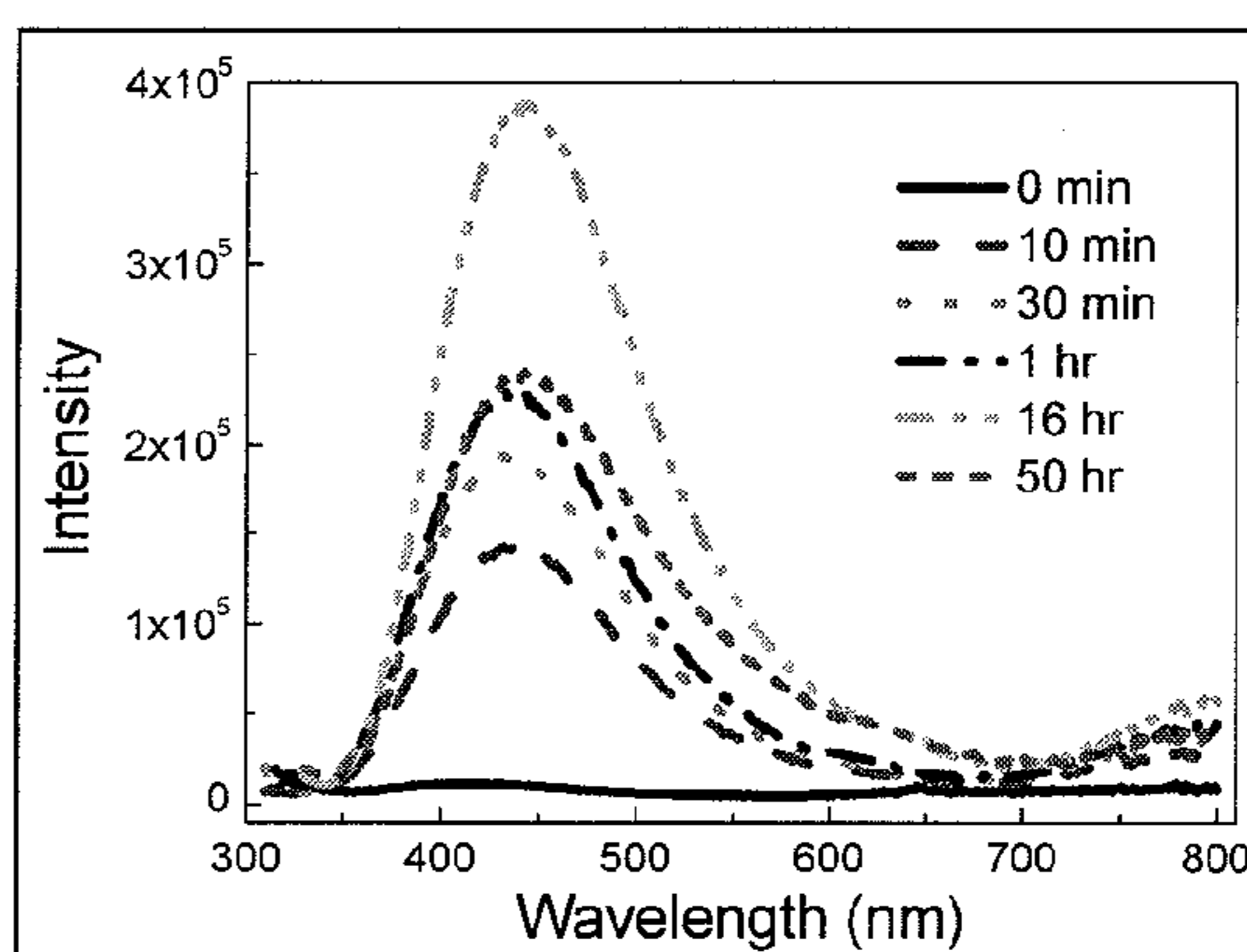
Fig.6. PL intensity of ZnS after reflux at different amount of time. Reflux at 100°C for 16 hrs gives the highest intensity.
