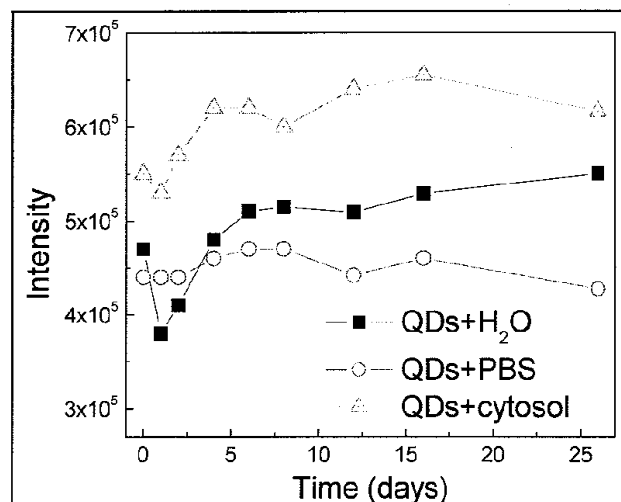
Fig.4. The PL intensity of aqueous CdS QDs as a function of time in water, PBS, and cytosol, respectively.
