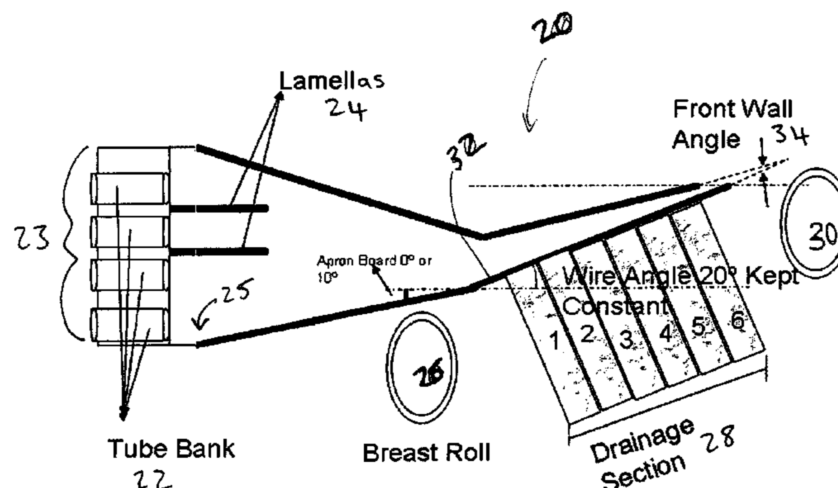
Hydroformer Schematic
