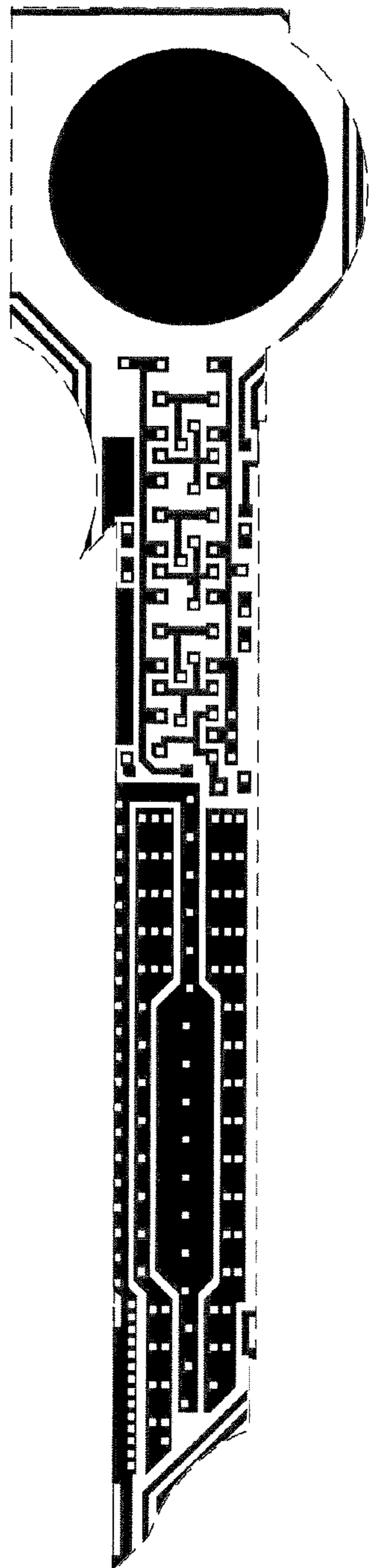
Metal 1 mask
