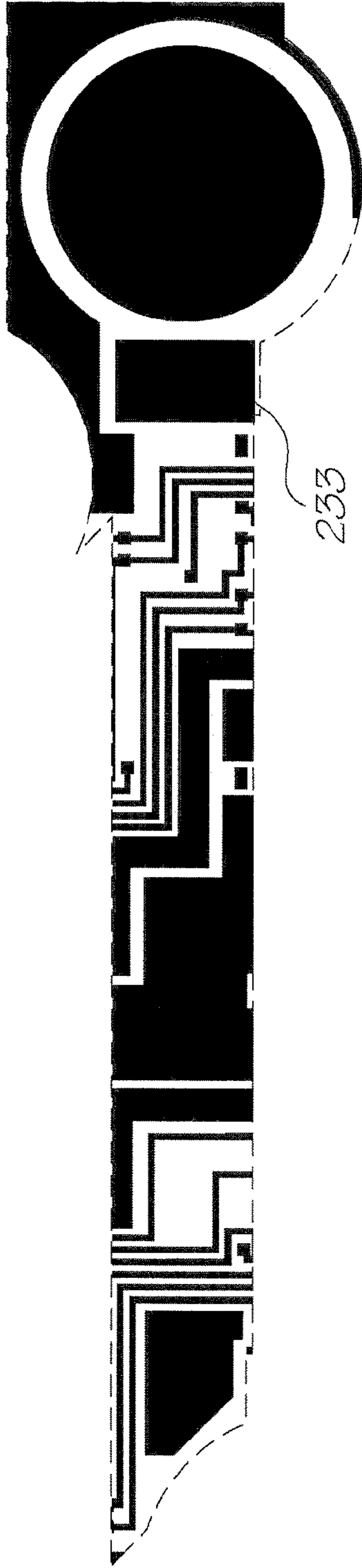
Metal 2 mask
