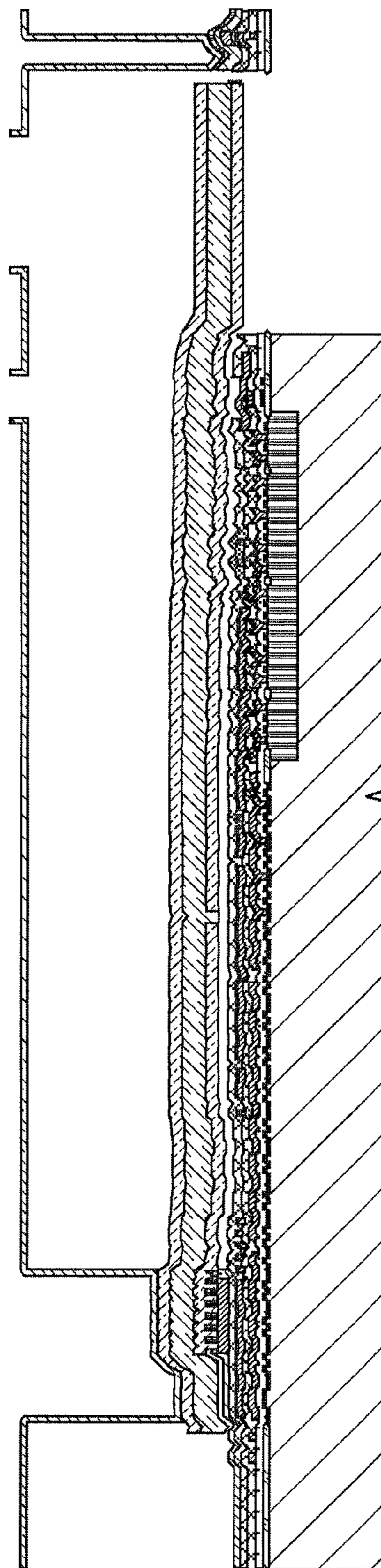
Detach from wafer blank, etch sacrificial material
