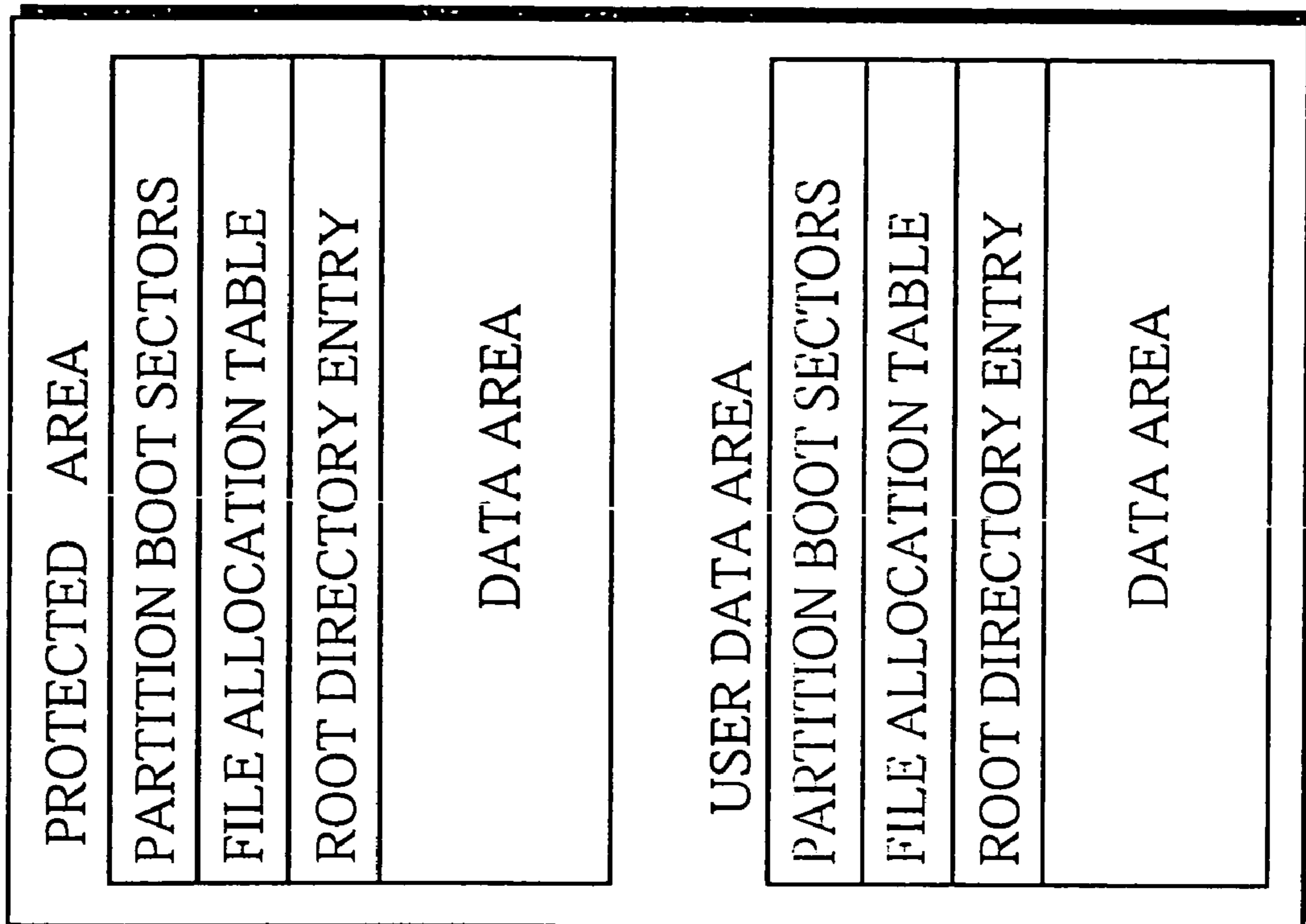
FIG. 4B FILE SYSTEM LAYER (ISO/IEC 9293)
