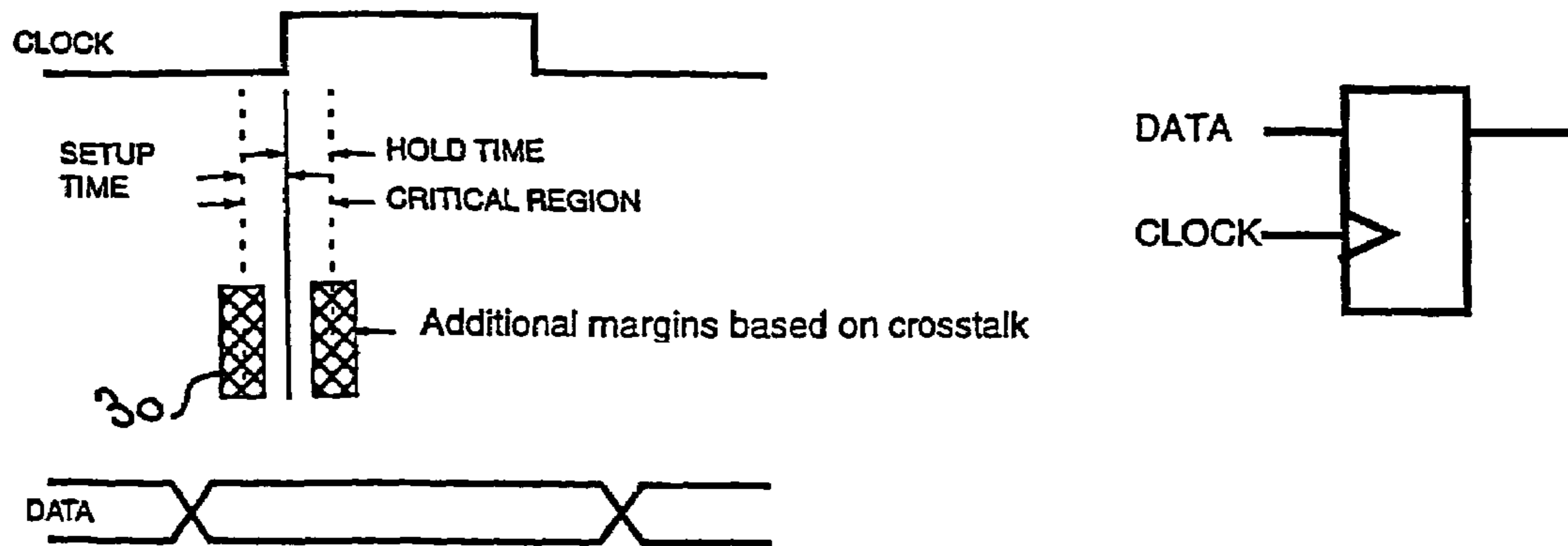
Figure 3,. Static Timing analysis with crosstalk back-annotation
