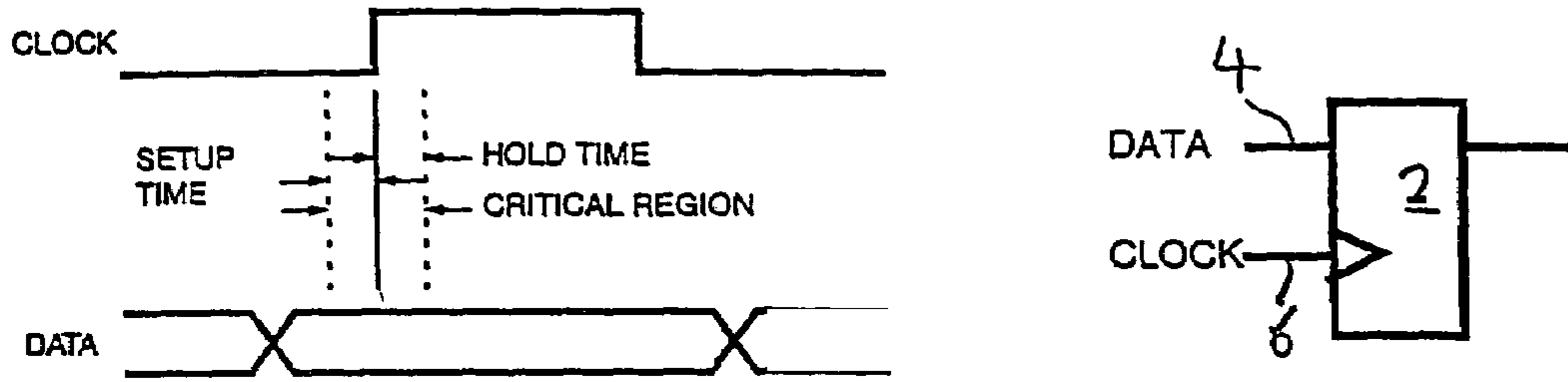
Figure 1. Traditional Static Timing analysis
