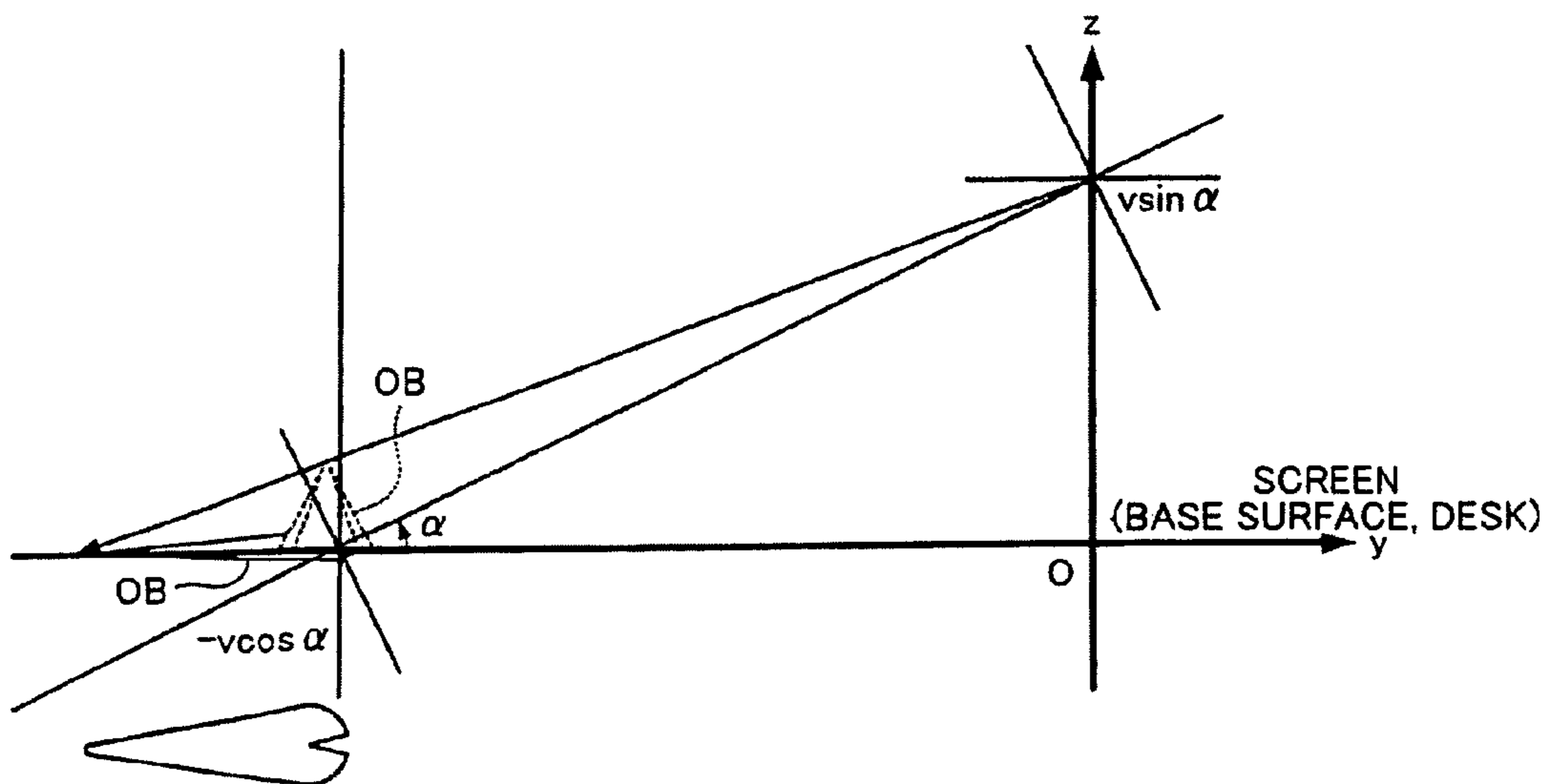
FIG. 27B PROJECTION P_z
