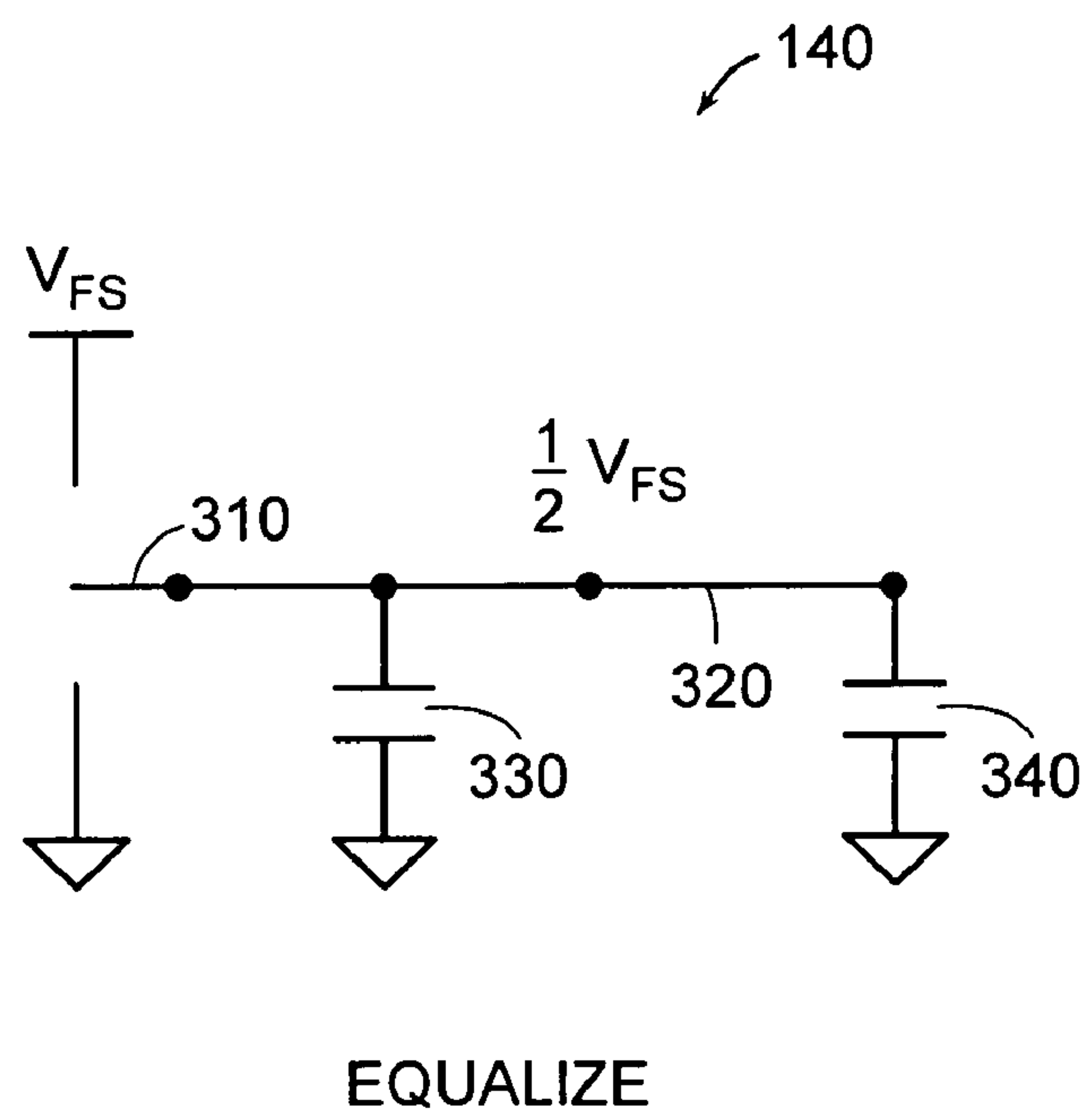
FIG. 3C PRIOR ART
