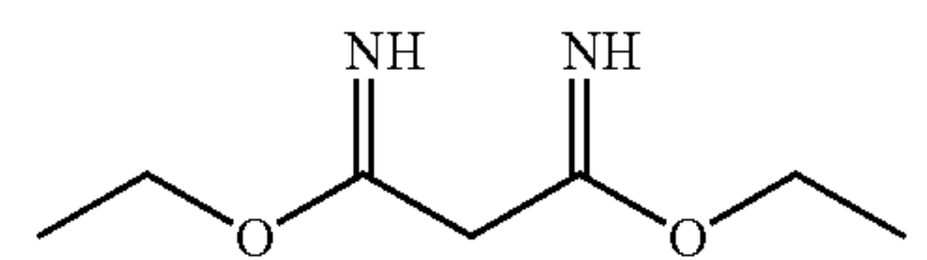
Diethyl malonite (DEM)
