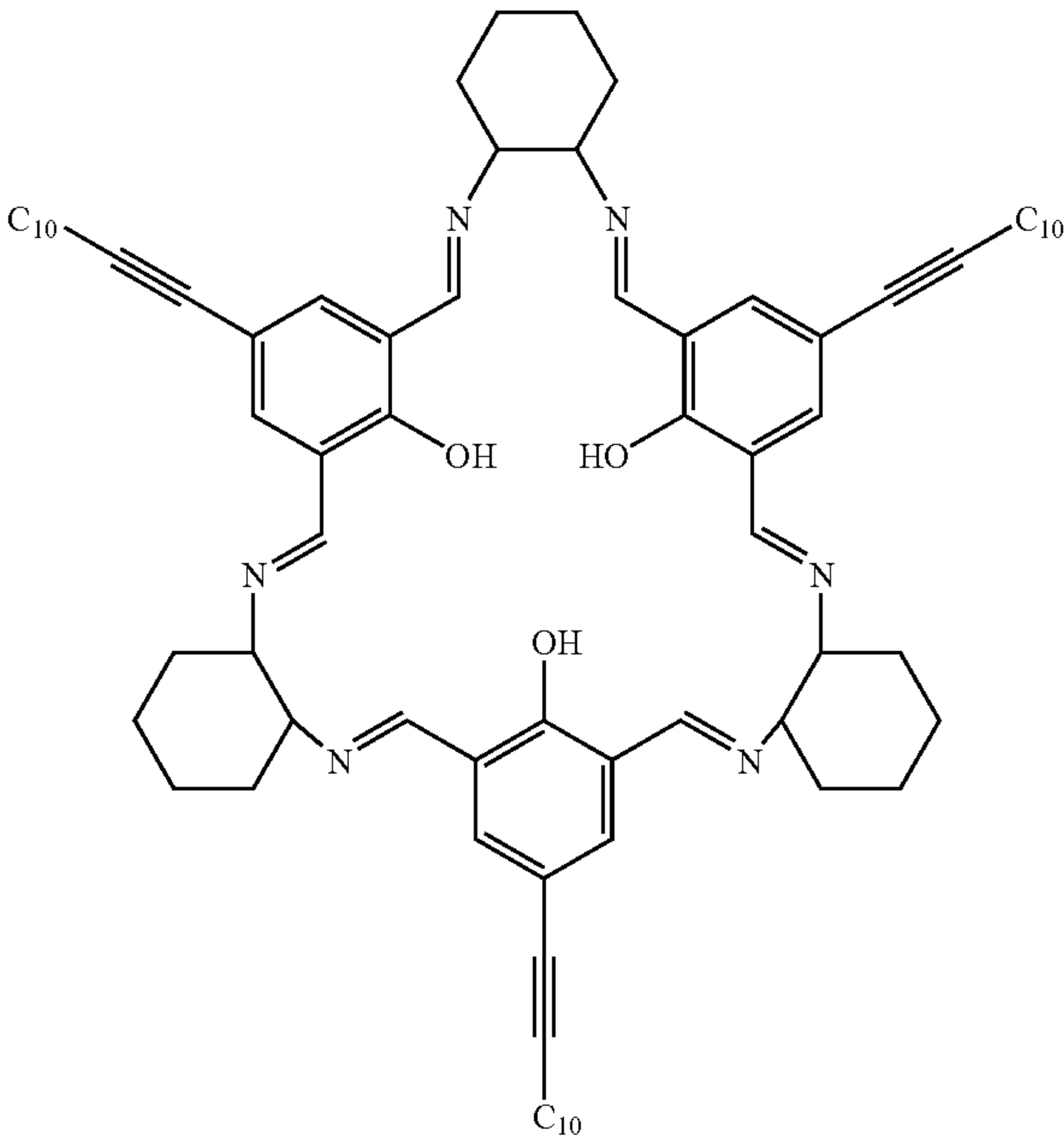
Hexamer 1a-1,2-imine
