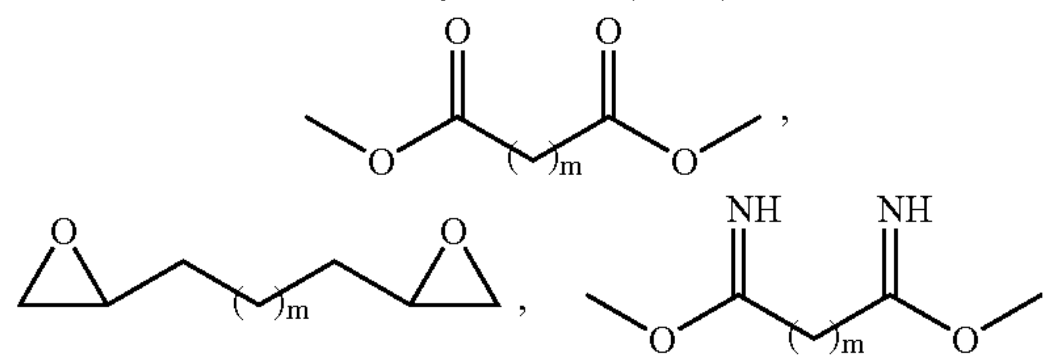
Diethyl malonite (DEM)
