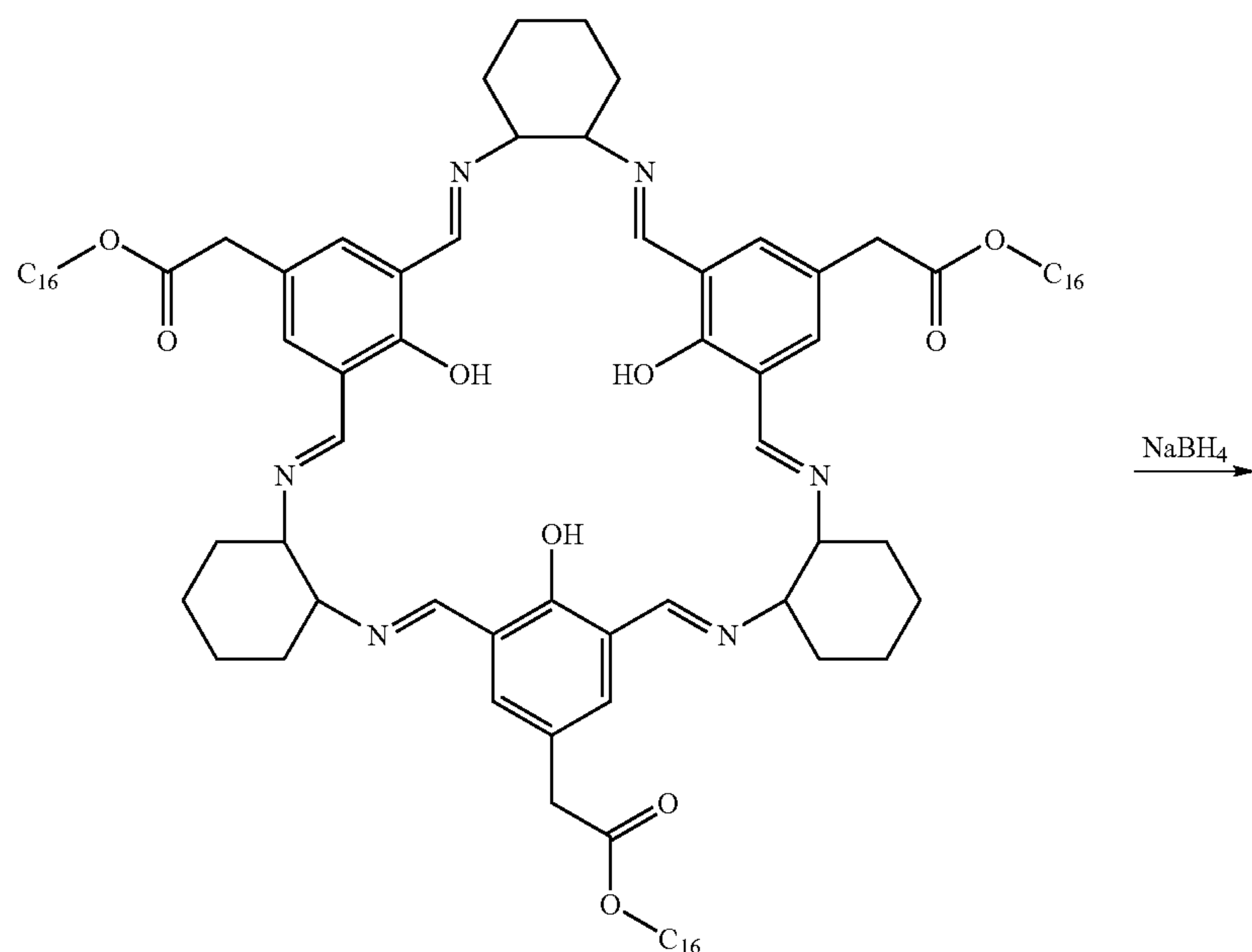
Hexamer 1j-1,2-imine
