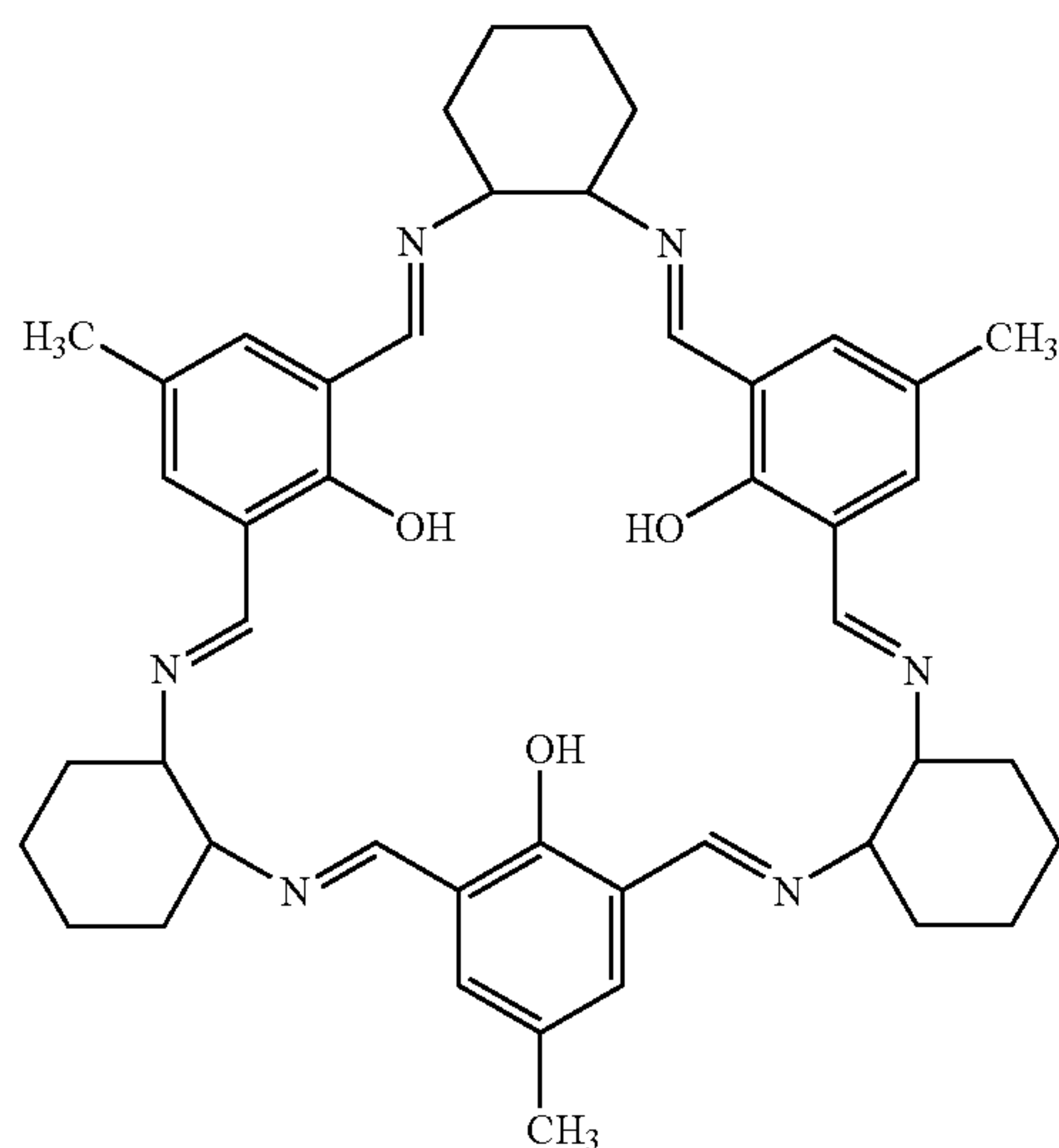
Hexamer 1a-Me-1,2-imine
