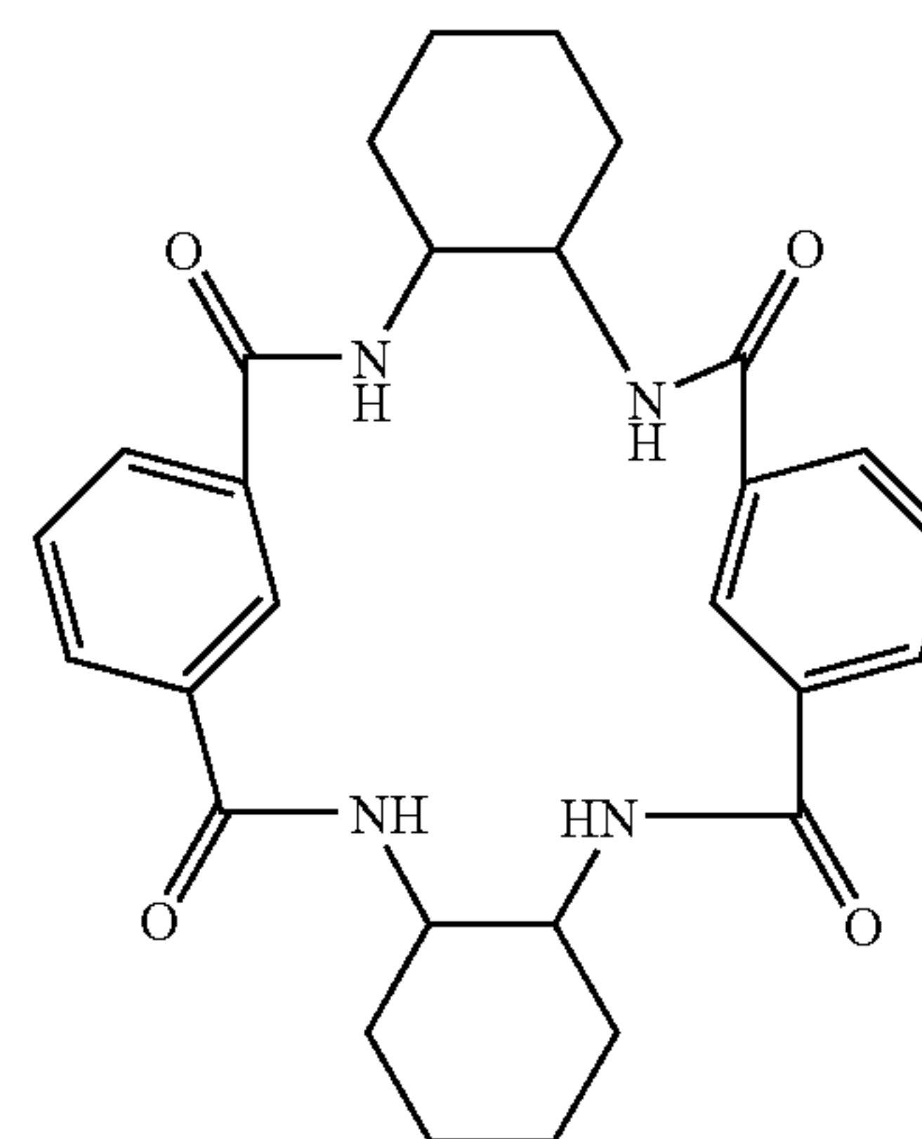
Tetramer 2-phenyl
