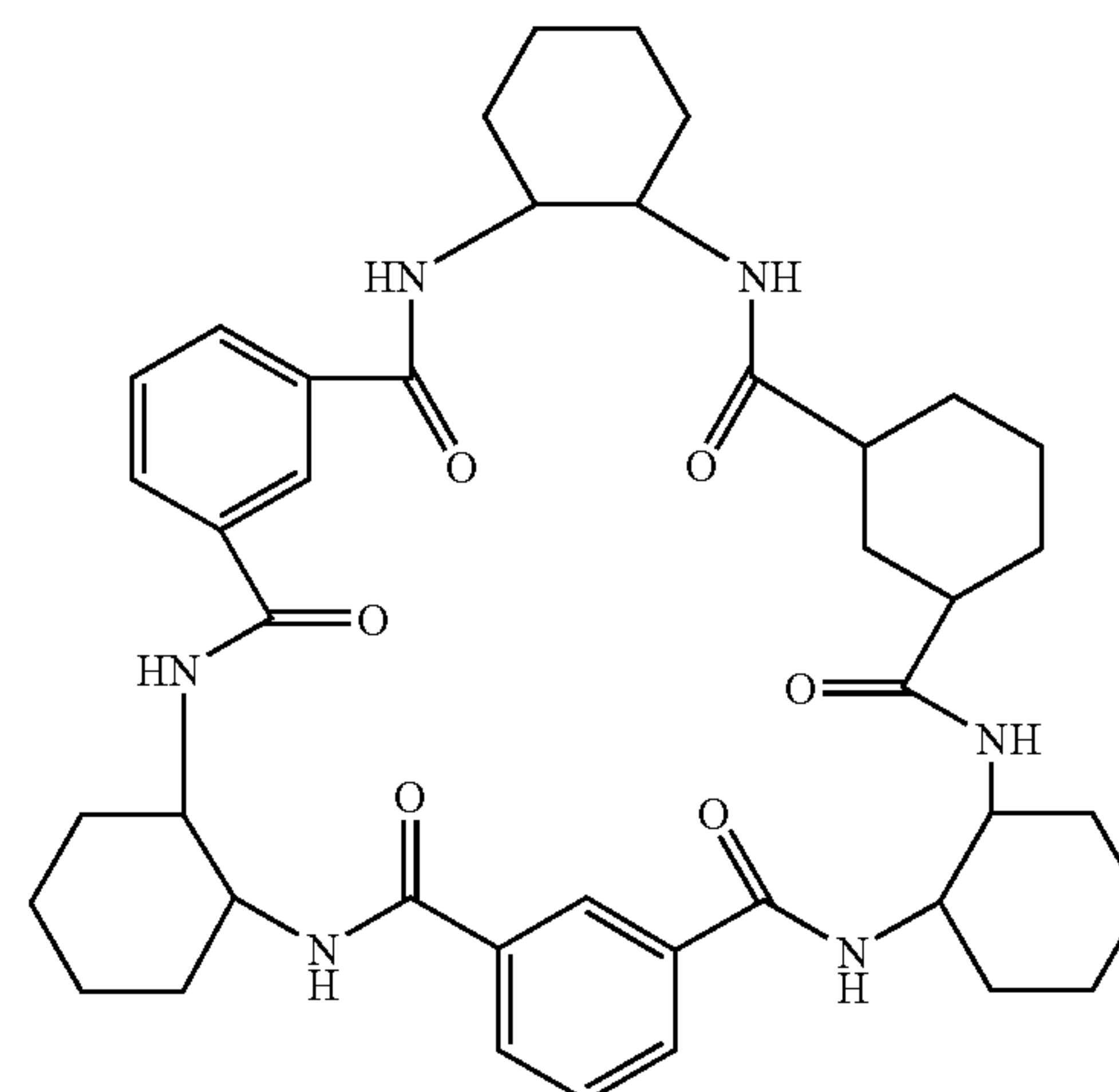
Hexamer 6-phenyl
