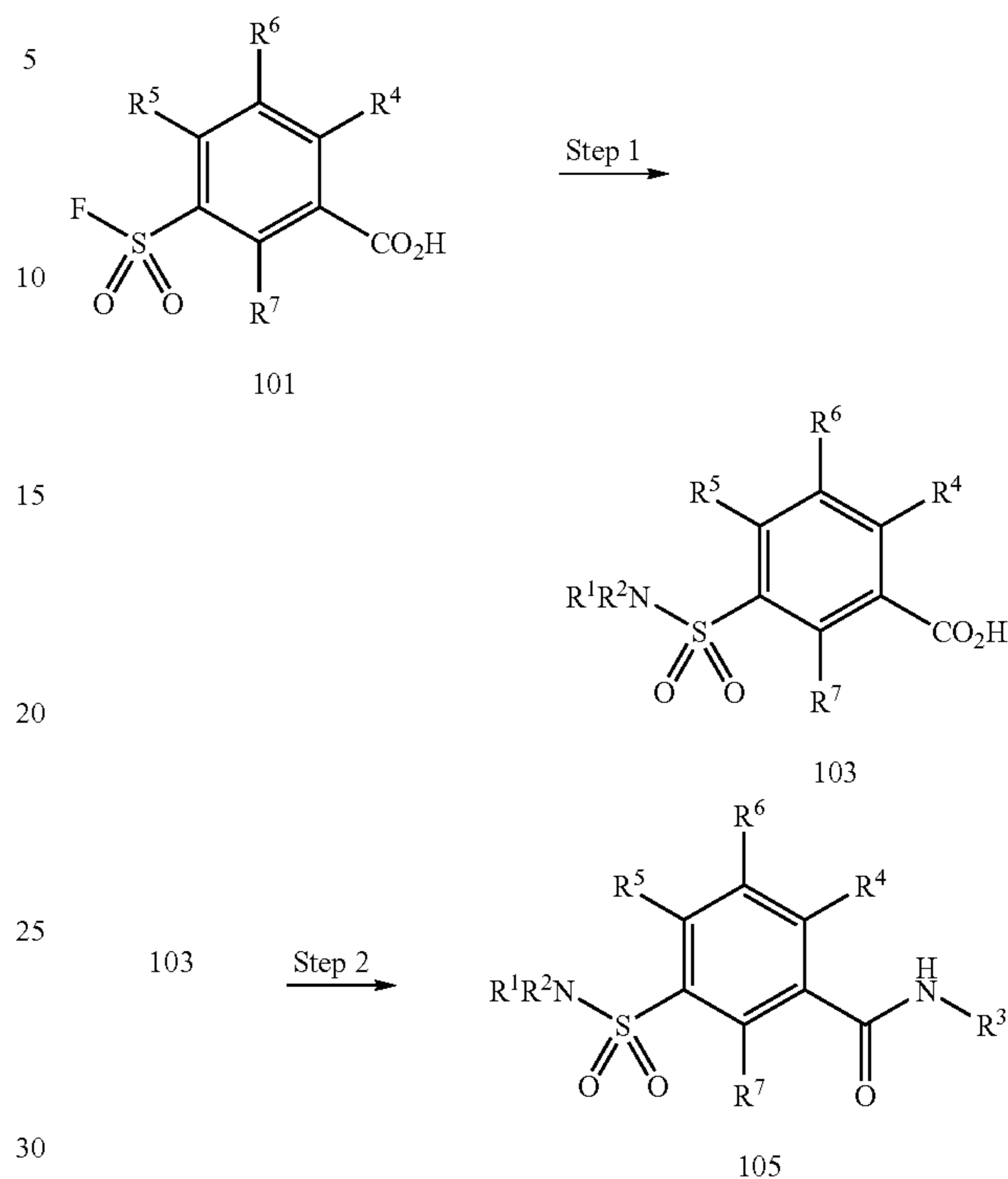
REACTION SCHEME 1
