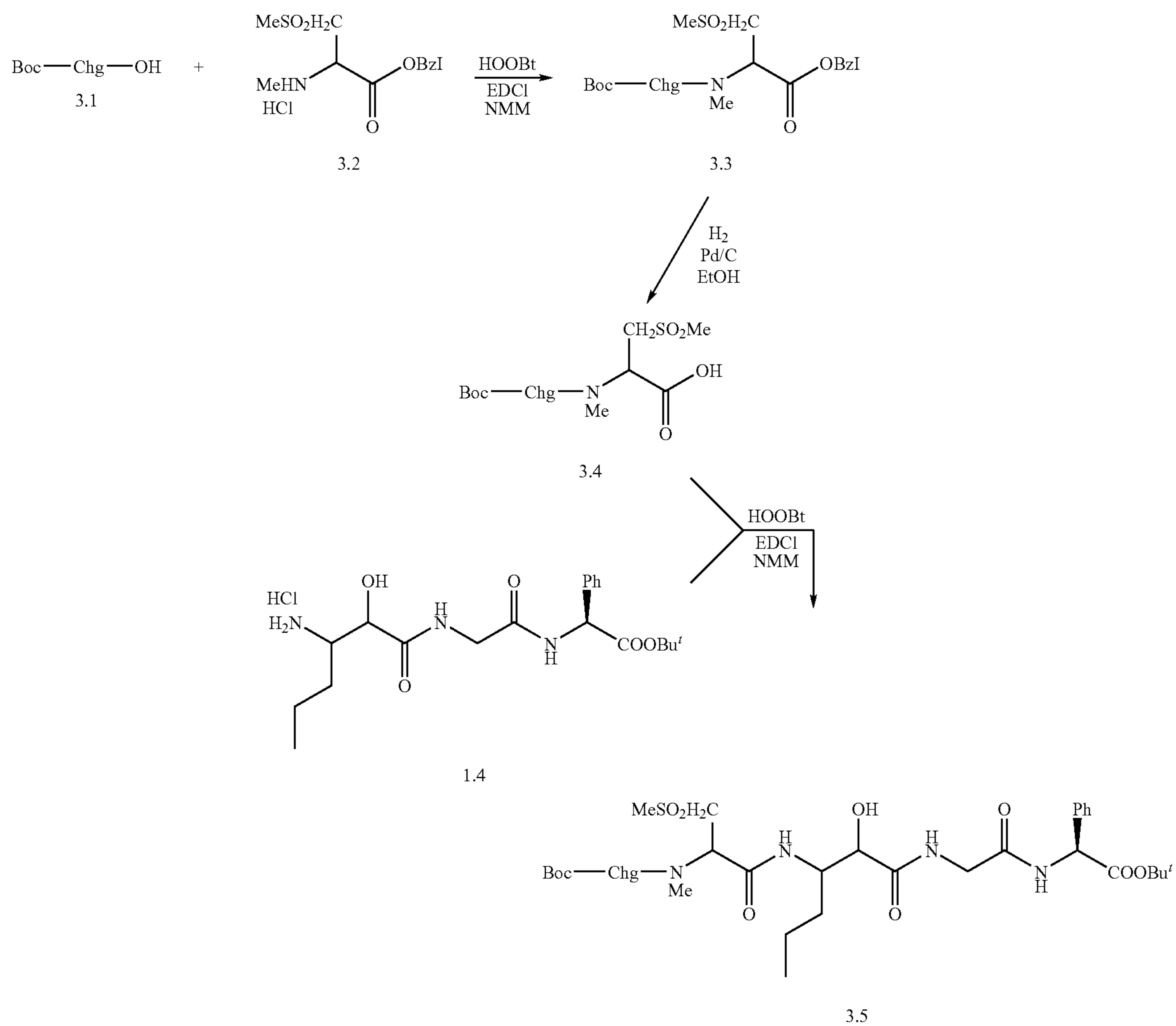
SCHEME 3
