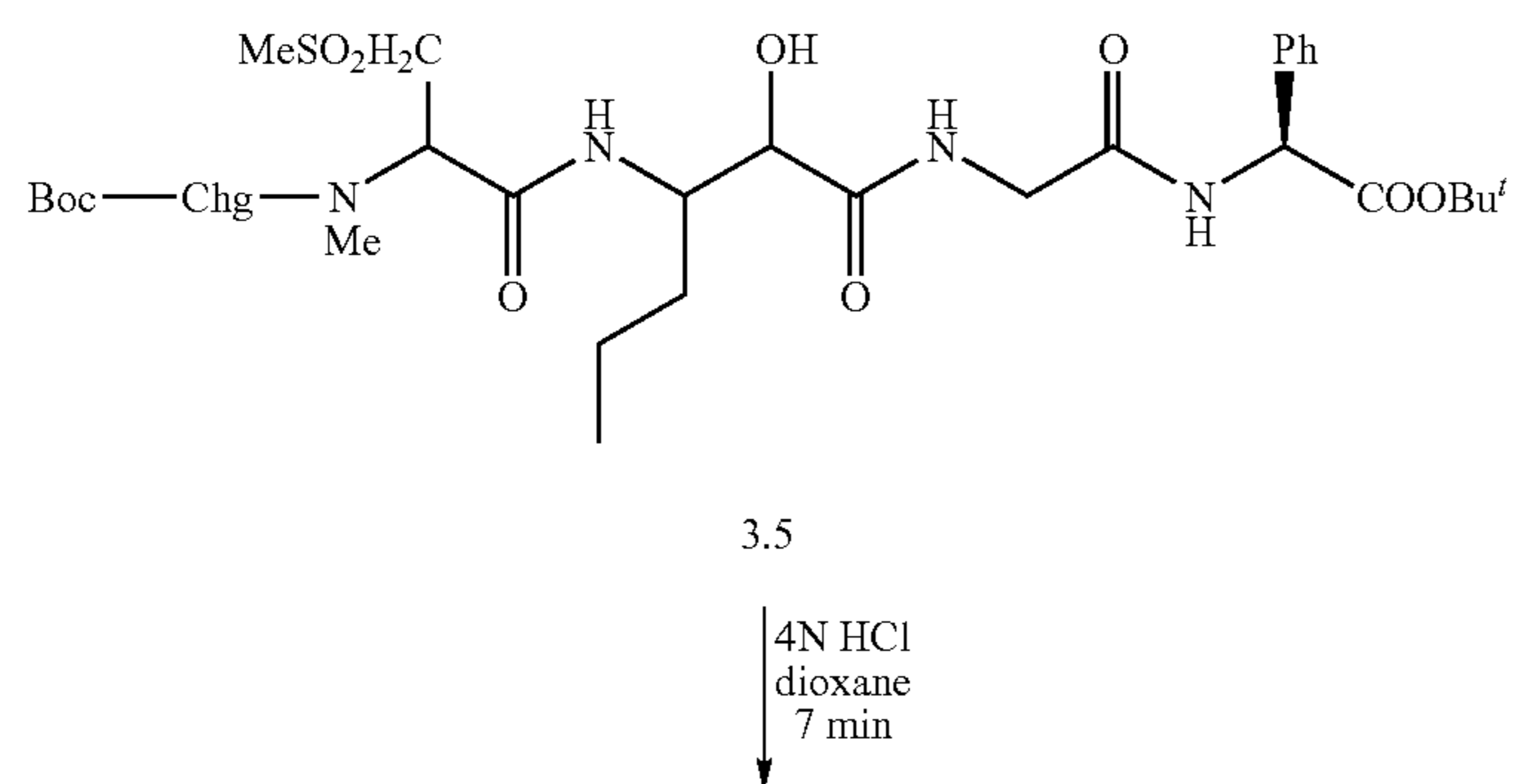
SCHEME 4
