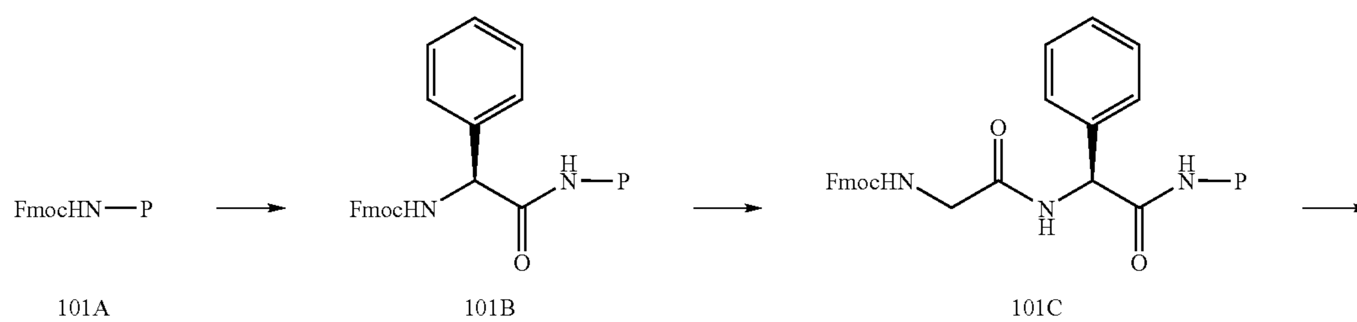
Scheme 5
