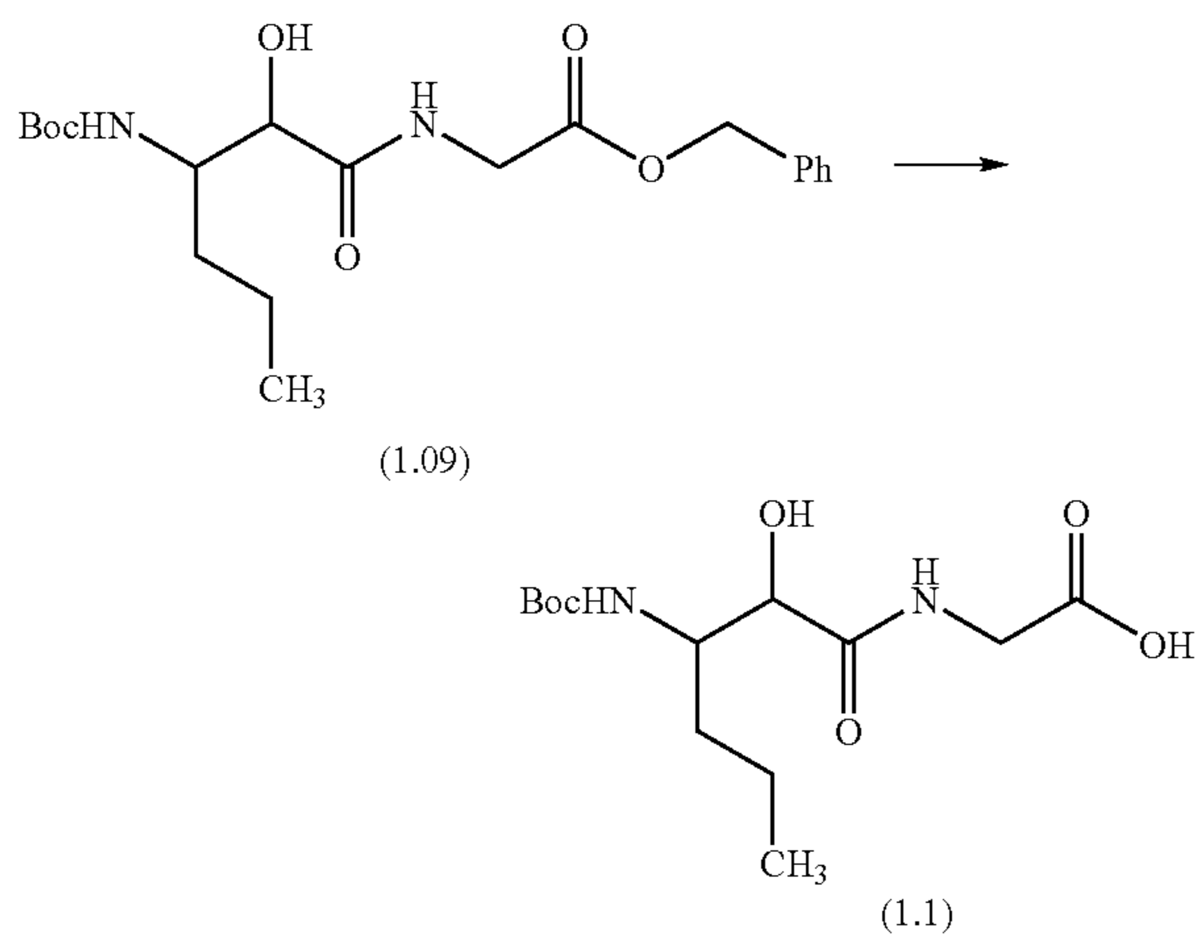
Compound (1.1)
