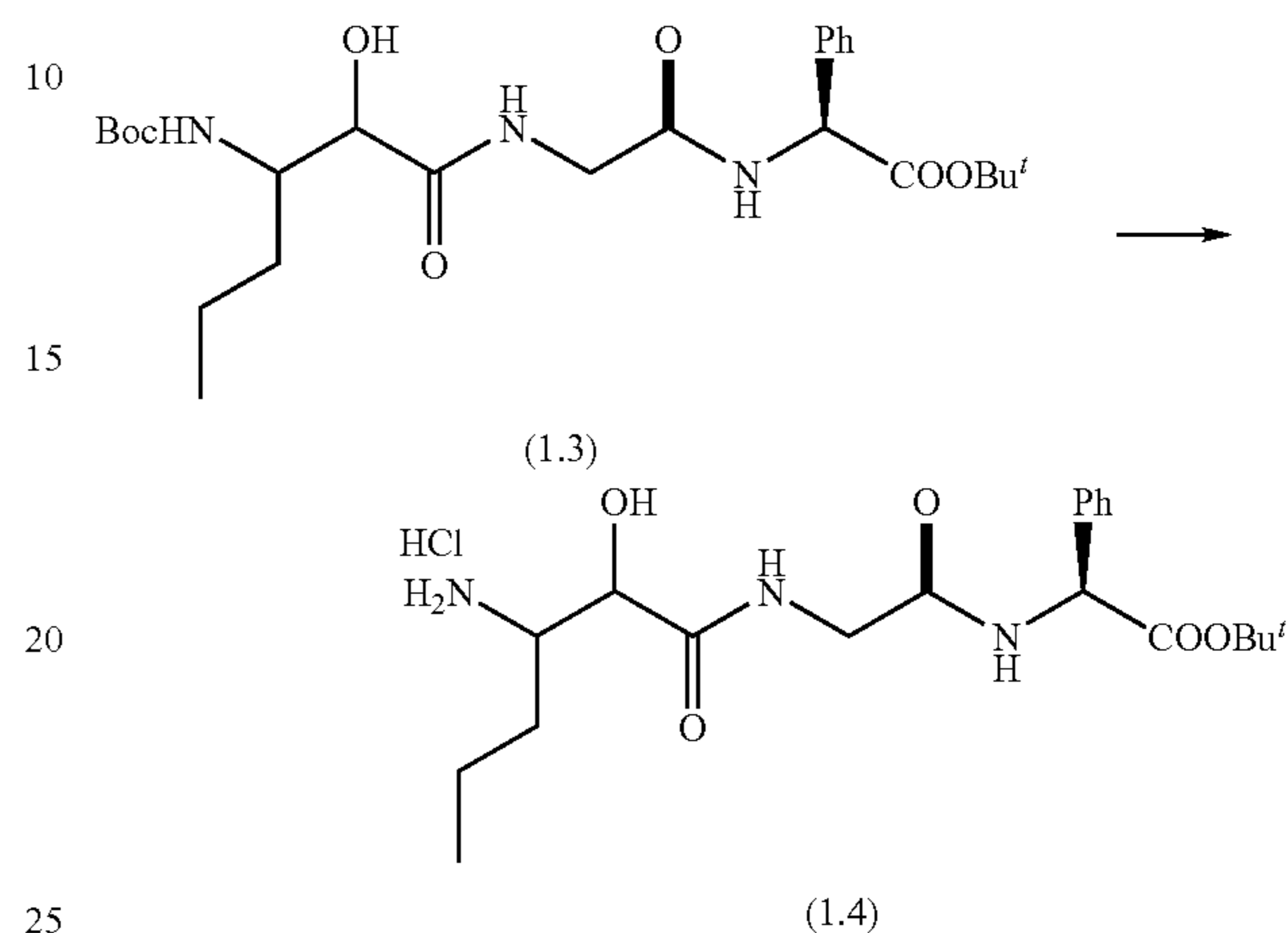
Compound (1.4)
