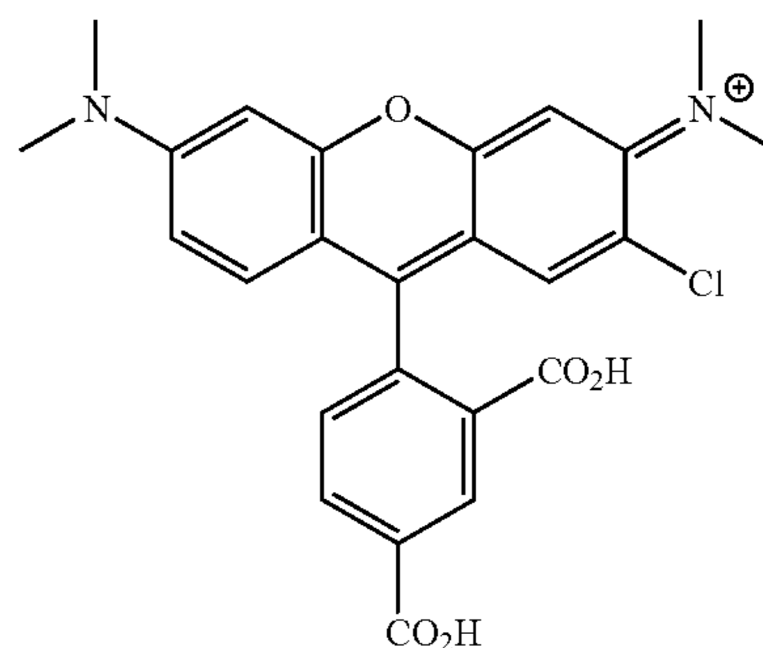
5-carboxyrhodamine
