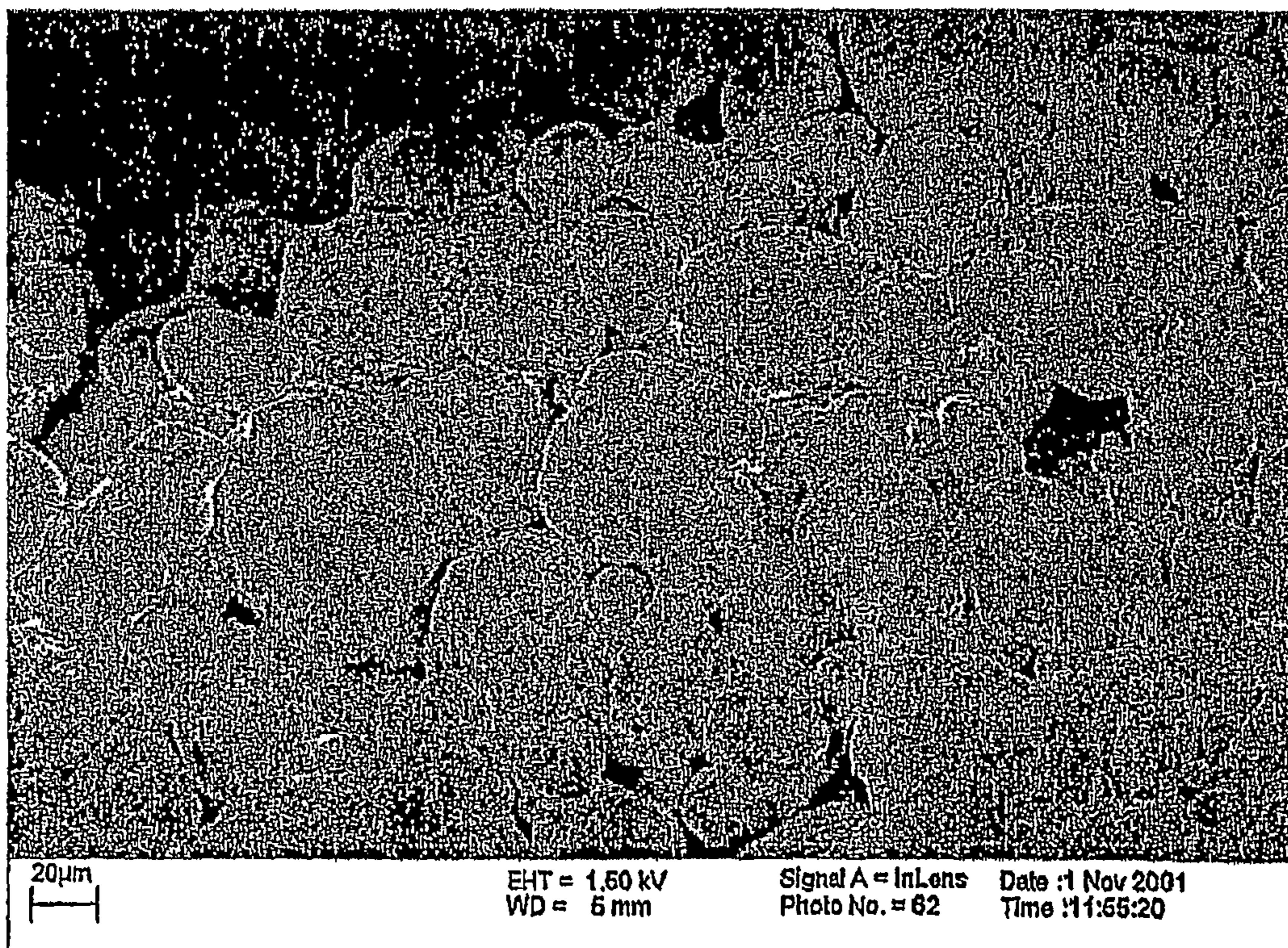
Figure 2: Standard basic magnesium carbonate
