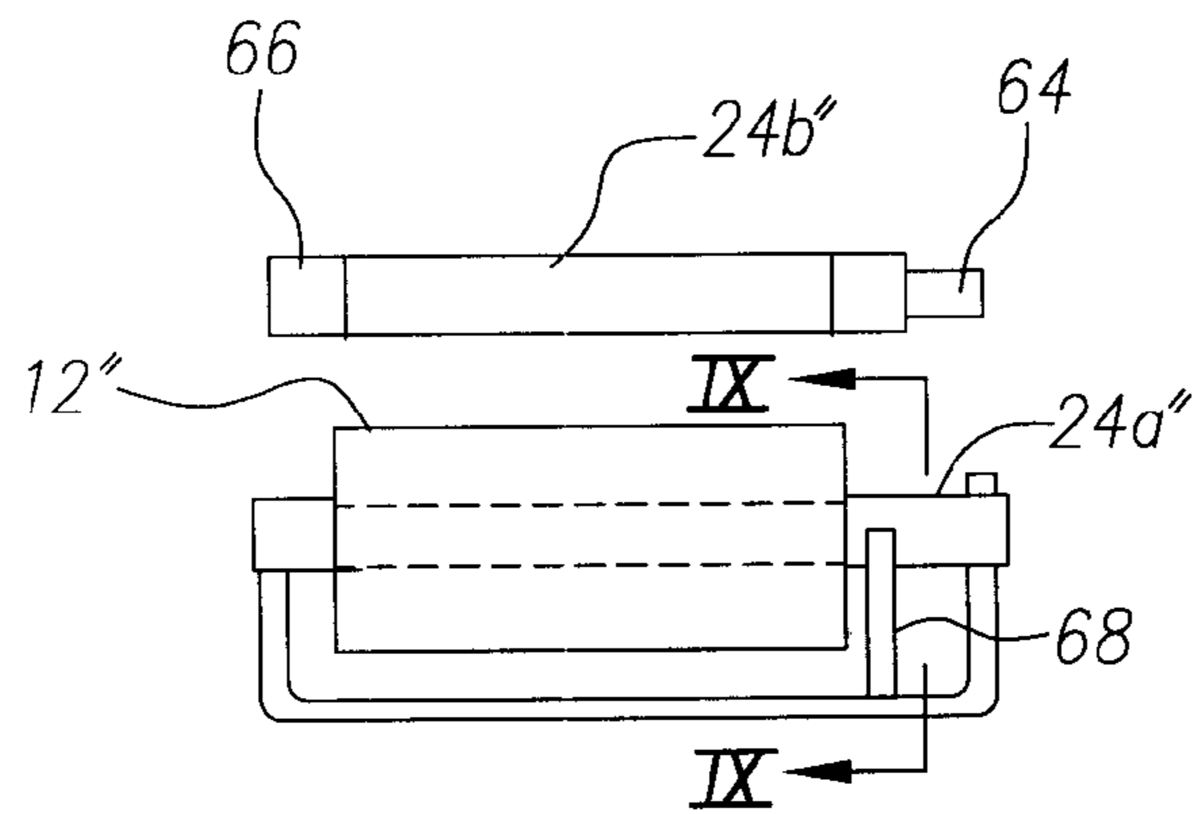
FIG. 7 (Prior Art)
