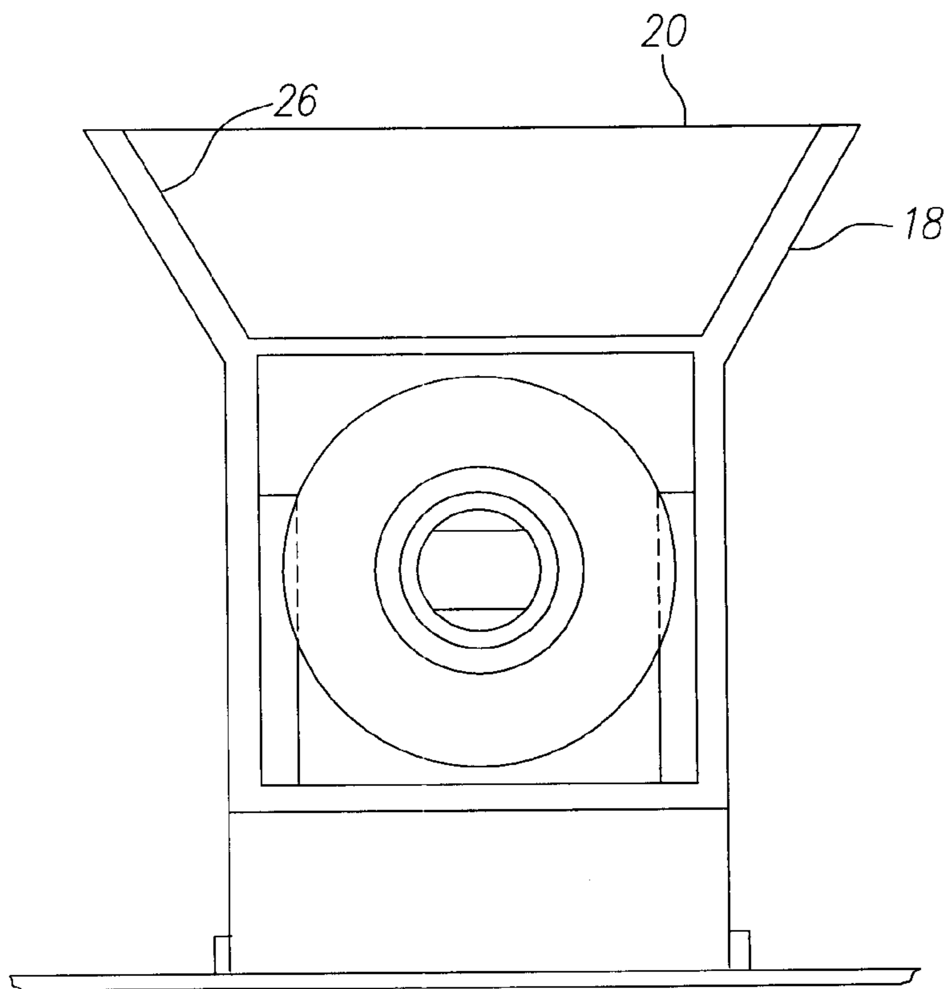
FIG. 4 (Prior Art)
