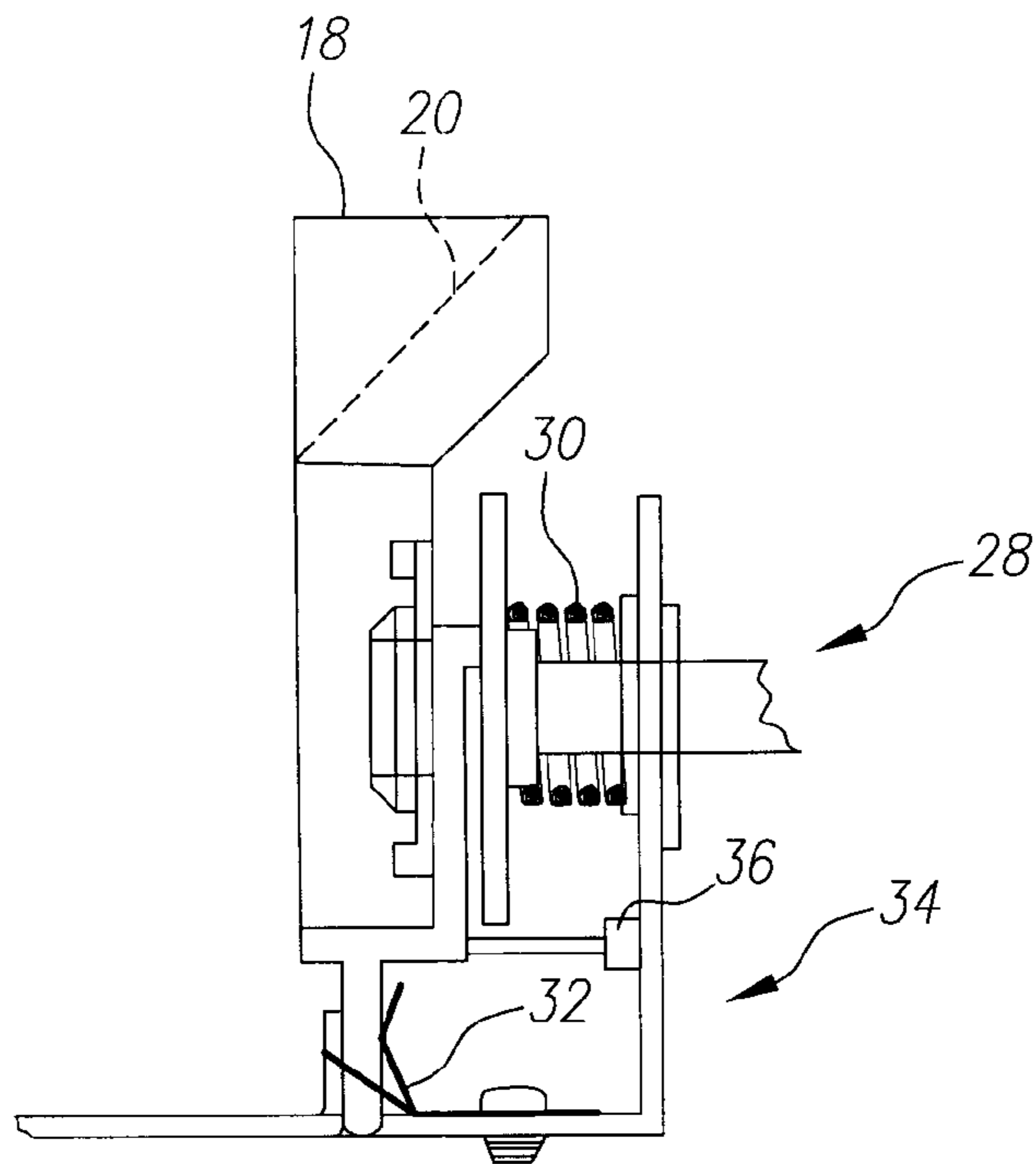
FIG. 3 (Prior Art)
