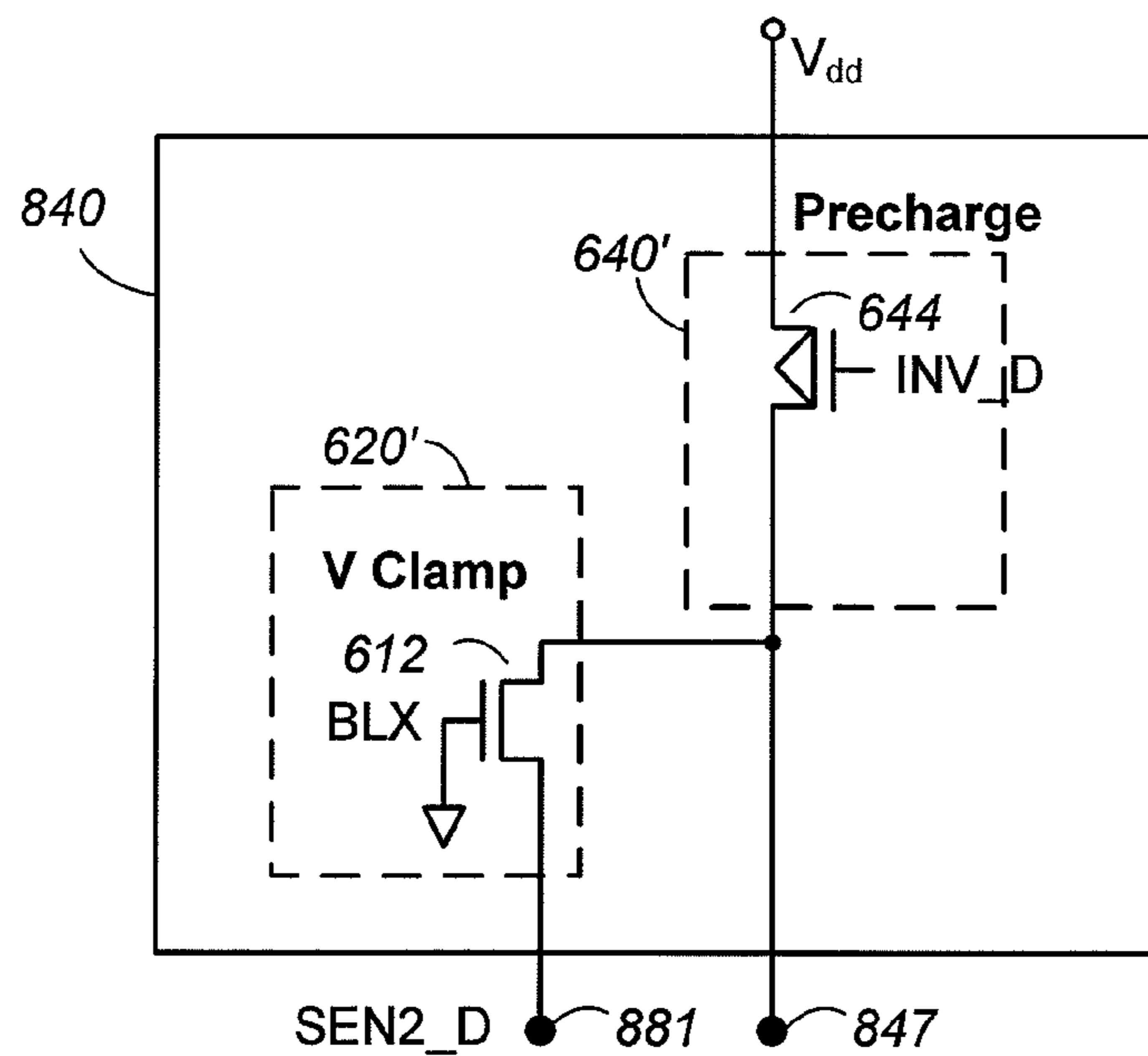
Precharge/Clamp Circuit of Ref Sense Amp
