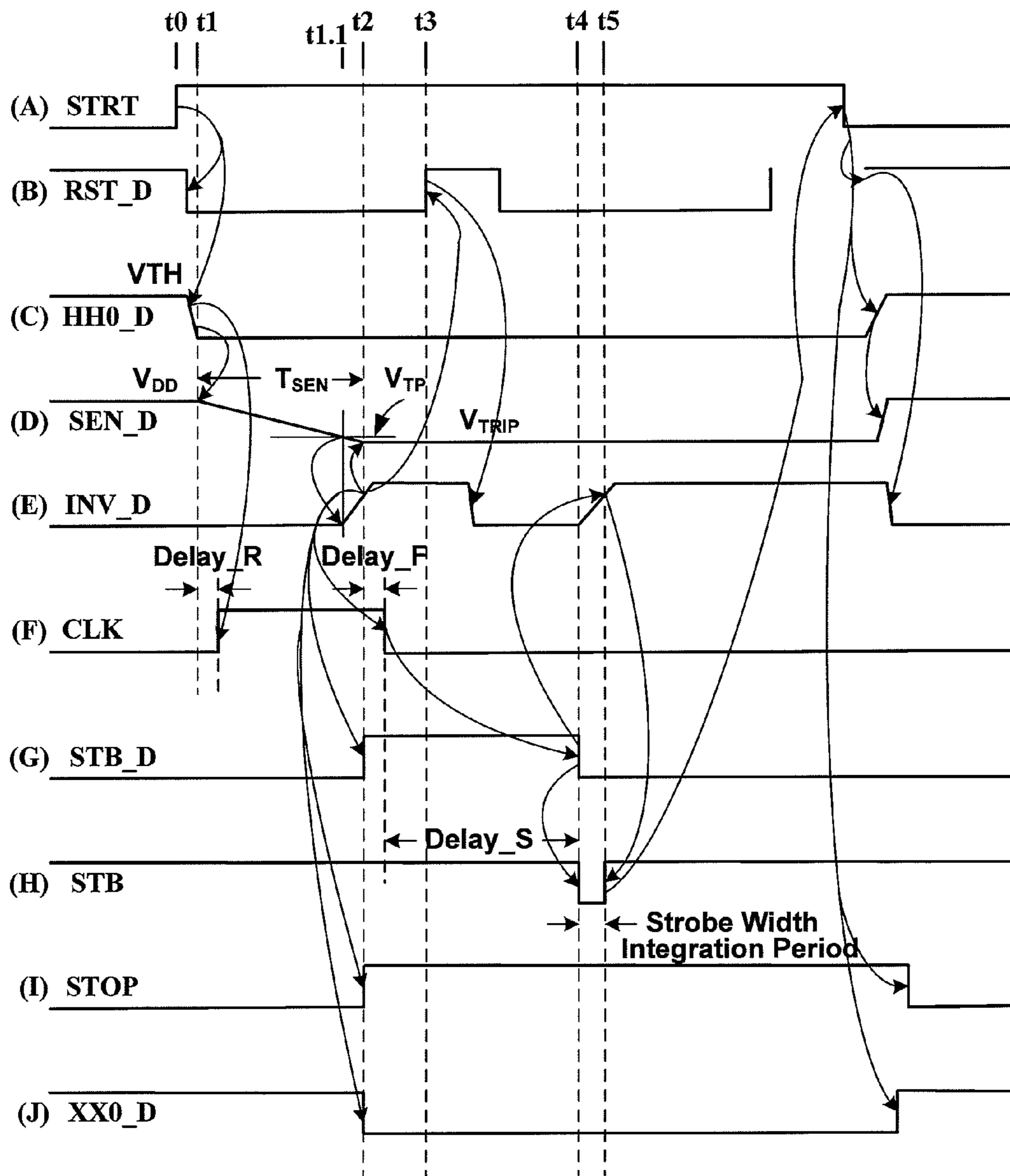
Reference Sense Amplifier's Timing Diagrams
