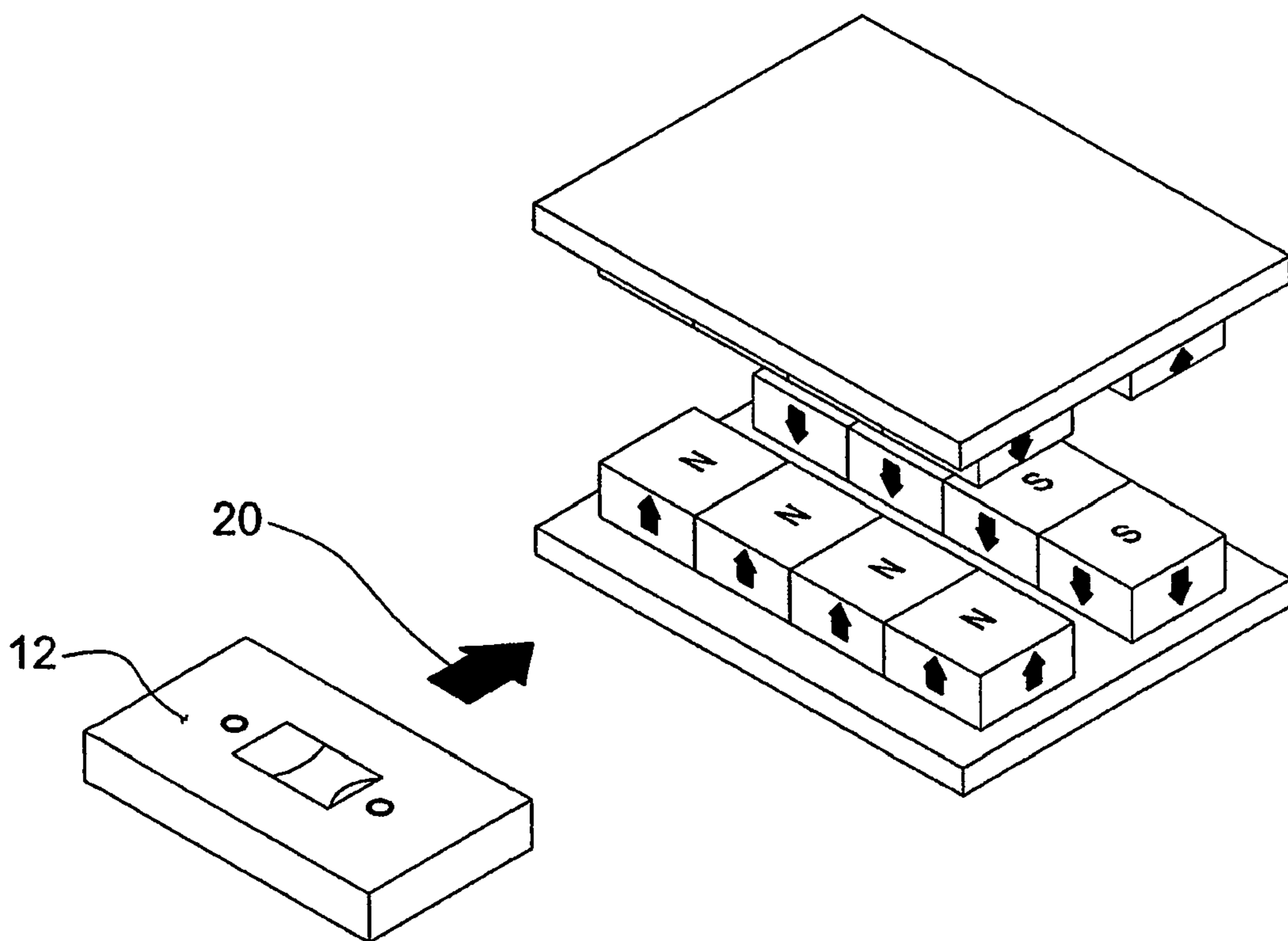
Figure 7 Prior Art
