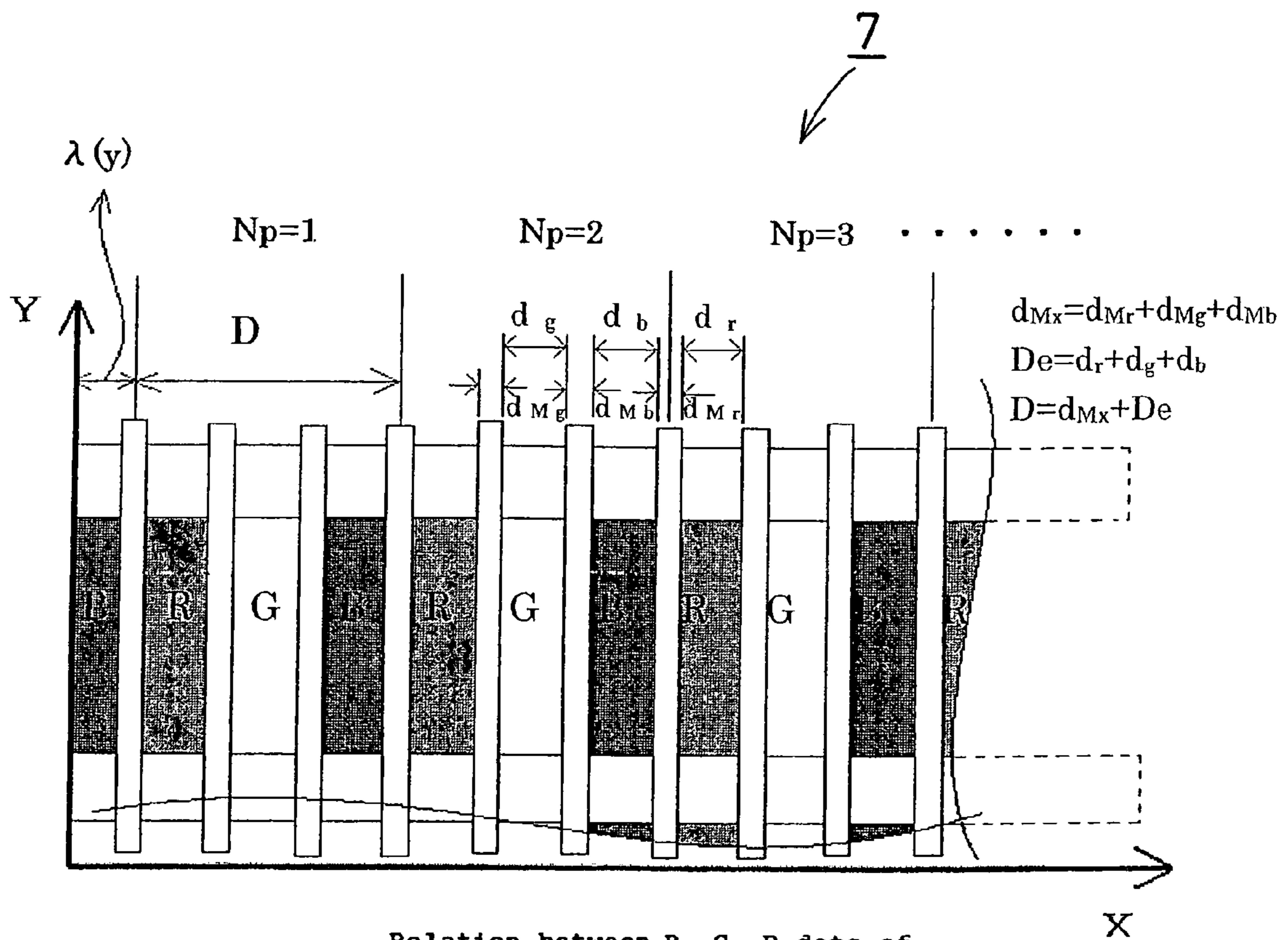
Relation between R, G, B dots of a liquid crystal panel and a pixel
