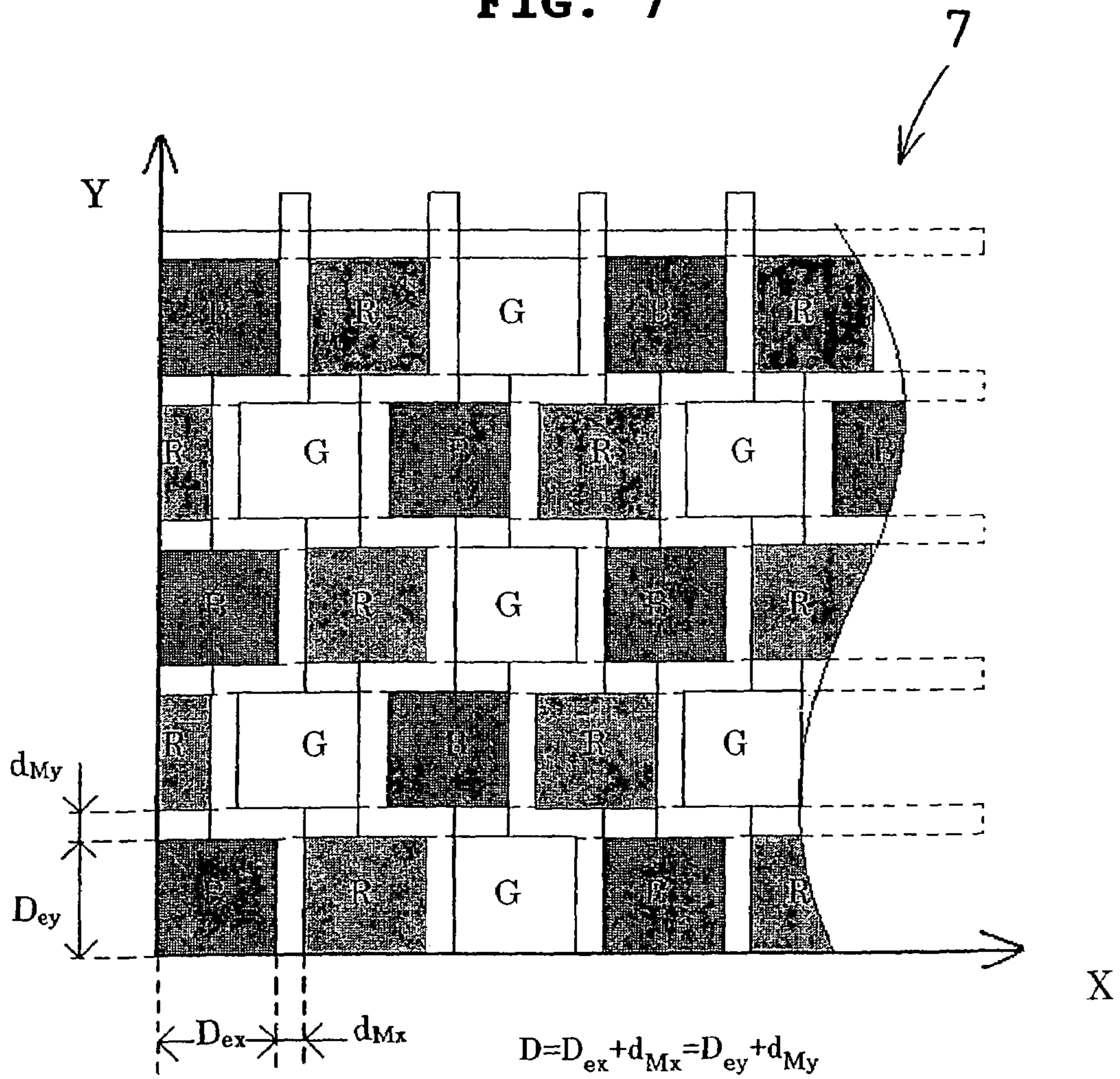
Liquid Crystal Panel with Delta Alignment
