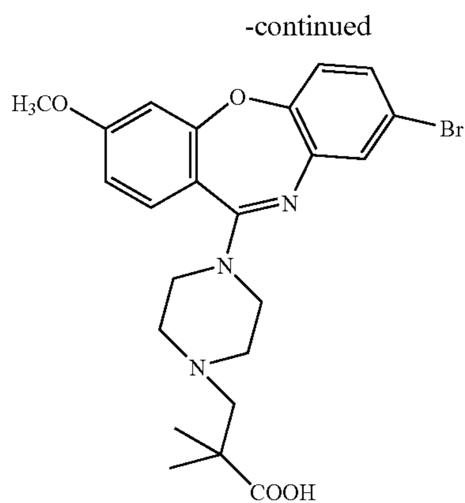
Compound 86
