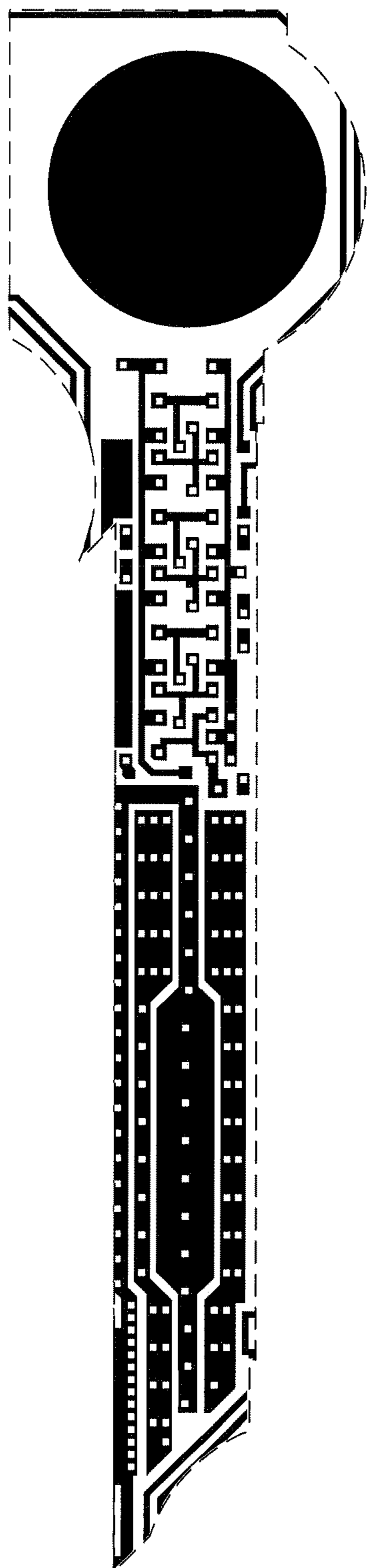
Metal 1 mask
