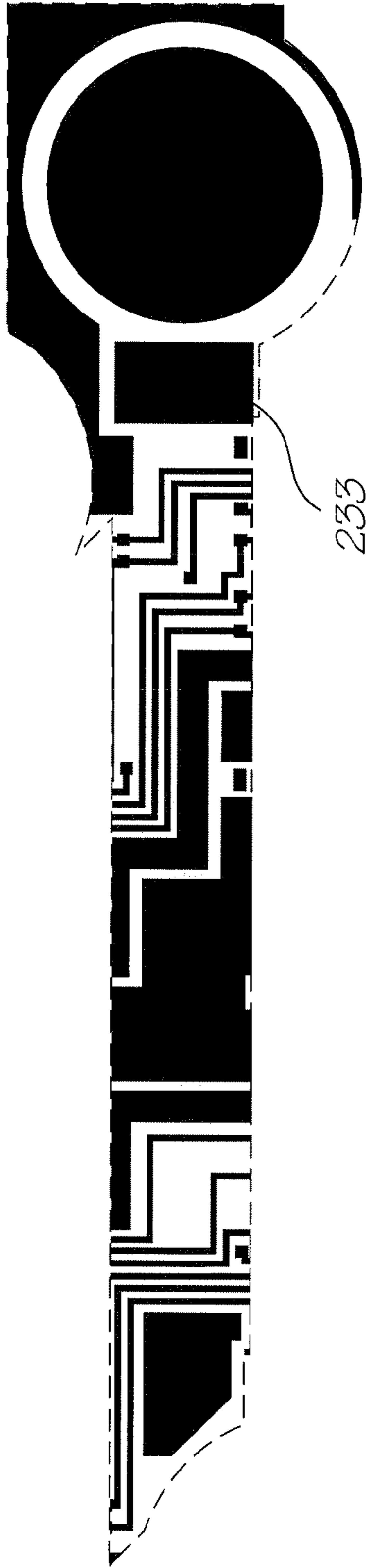
Metal 2 mask
