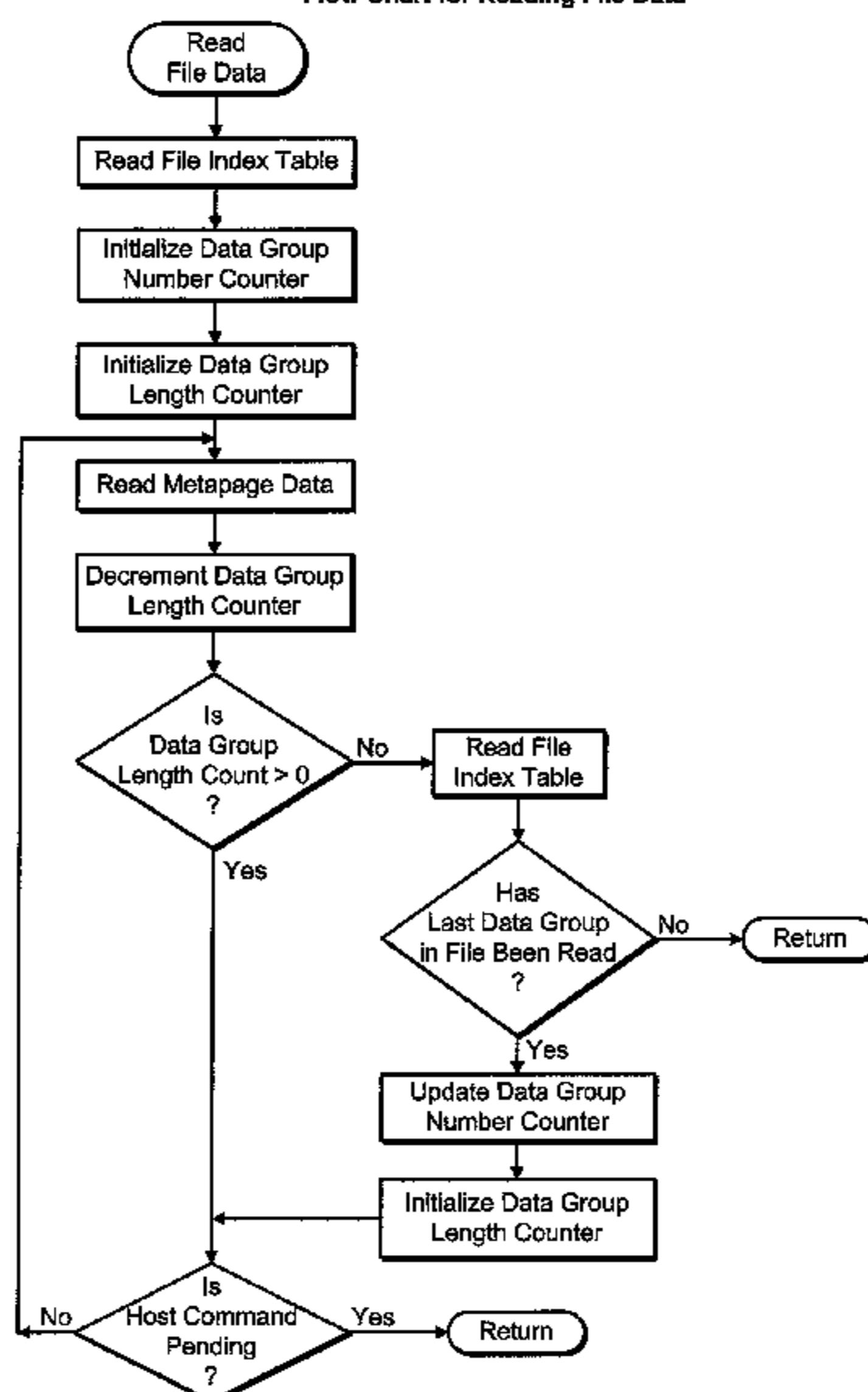
Flow Chart for Reading File Data
