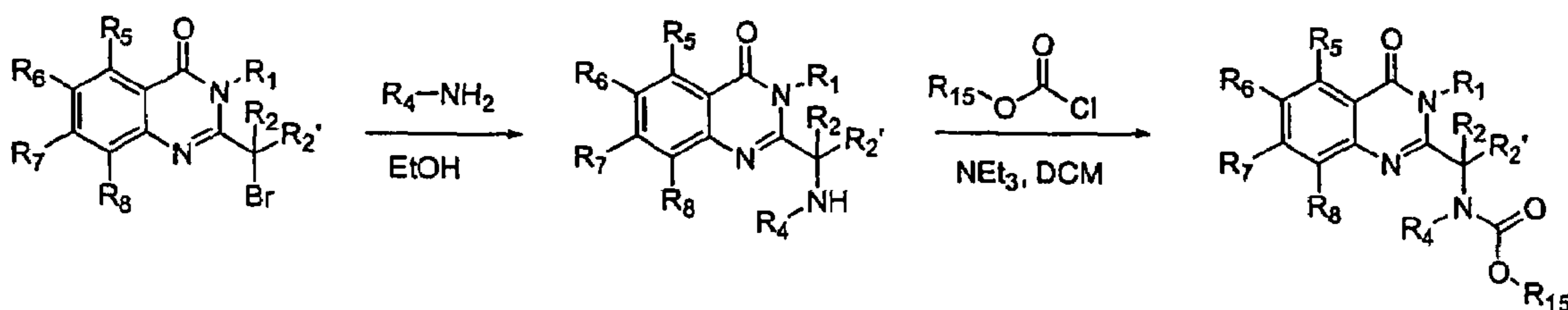
Figure 5c: Urea Synthesis
