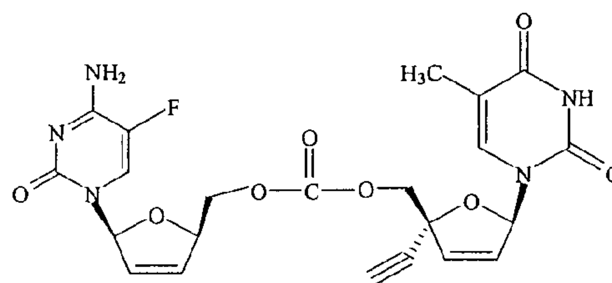
BLFd4C and TKD-4-114 Dinucleoside Carbonate
