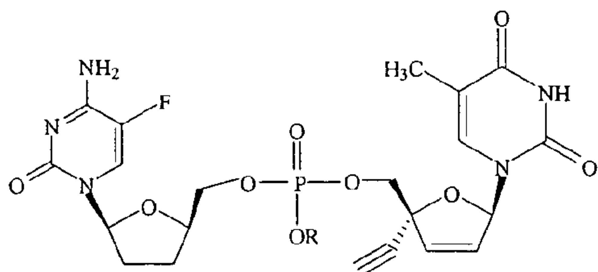
BLFddC and TKD-4-114 Dinucleoside Phosphate
