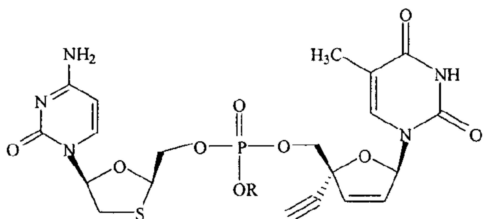
3TC and TKD-4-114 Dinucleoside Phosphate
