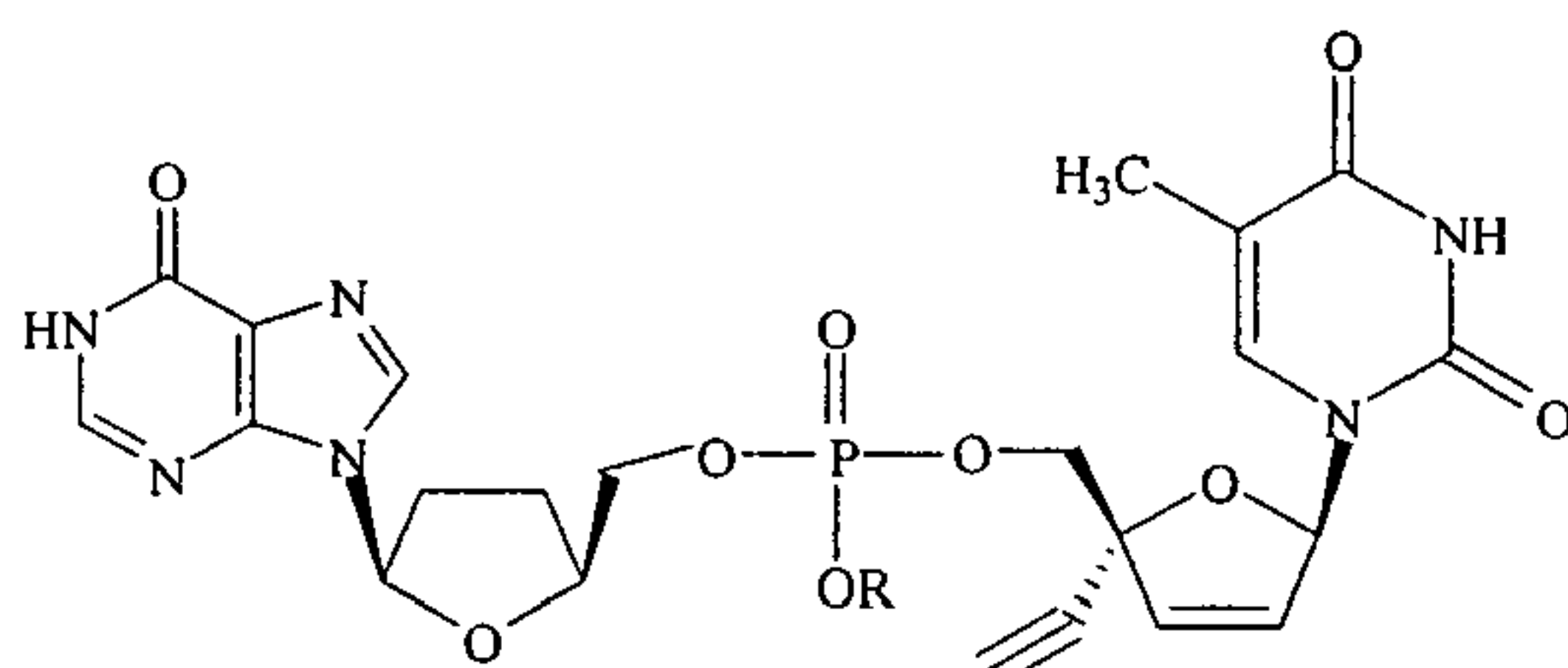
ddI and TKD-4-114 Dinucleoside Phosphate
