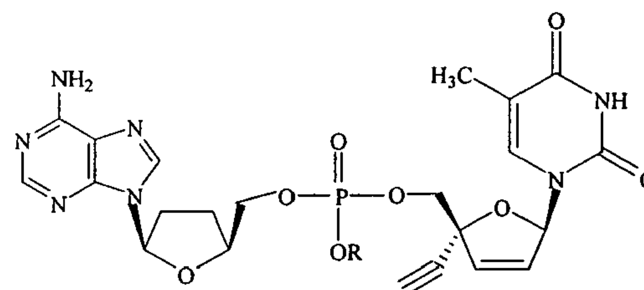
ddA and TKD-4-114 Dinucleoside Phosphate
