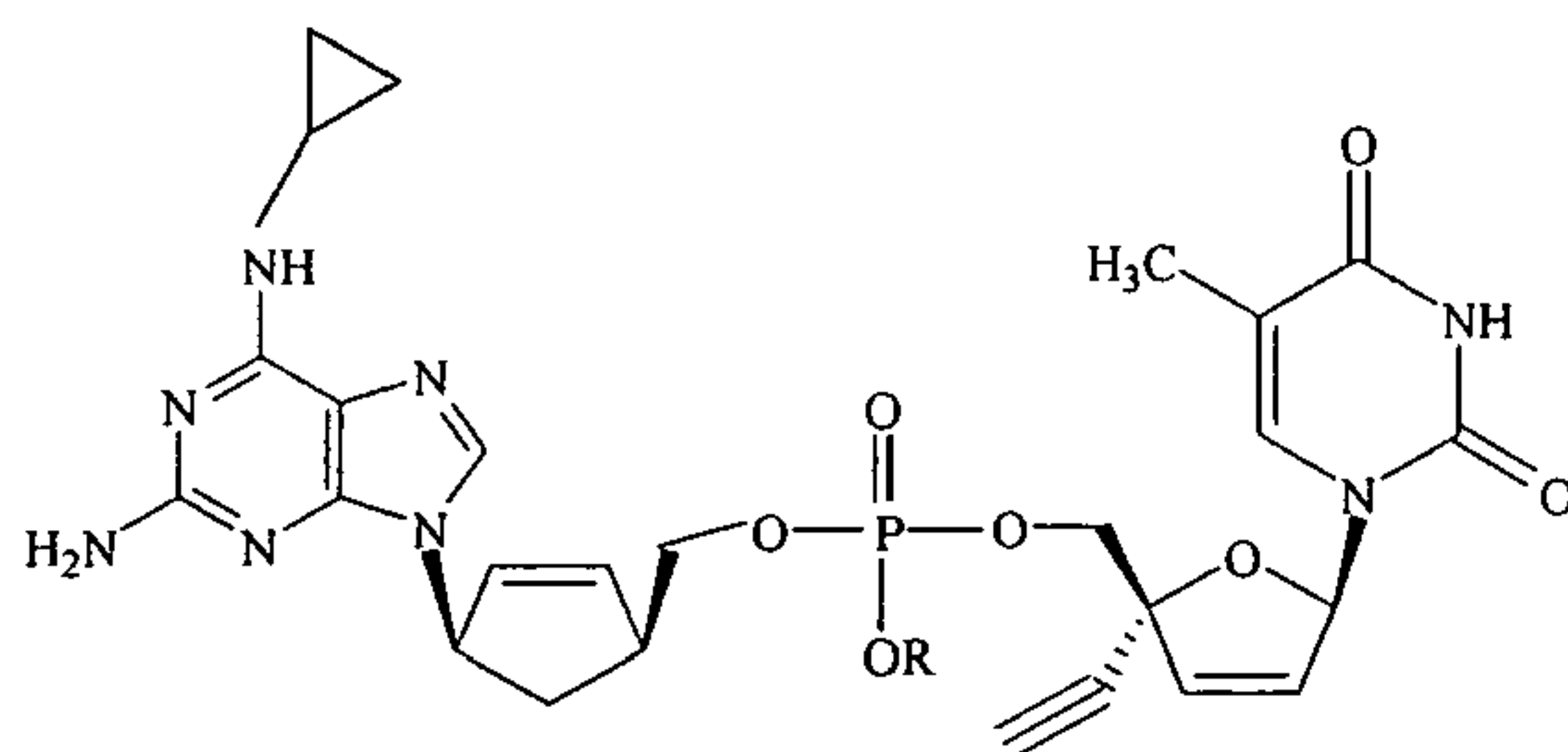
Abacavir and TKD-4-114 Dinucleoside Phosphate
