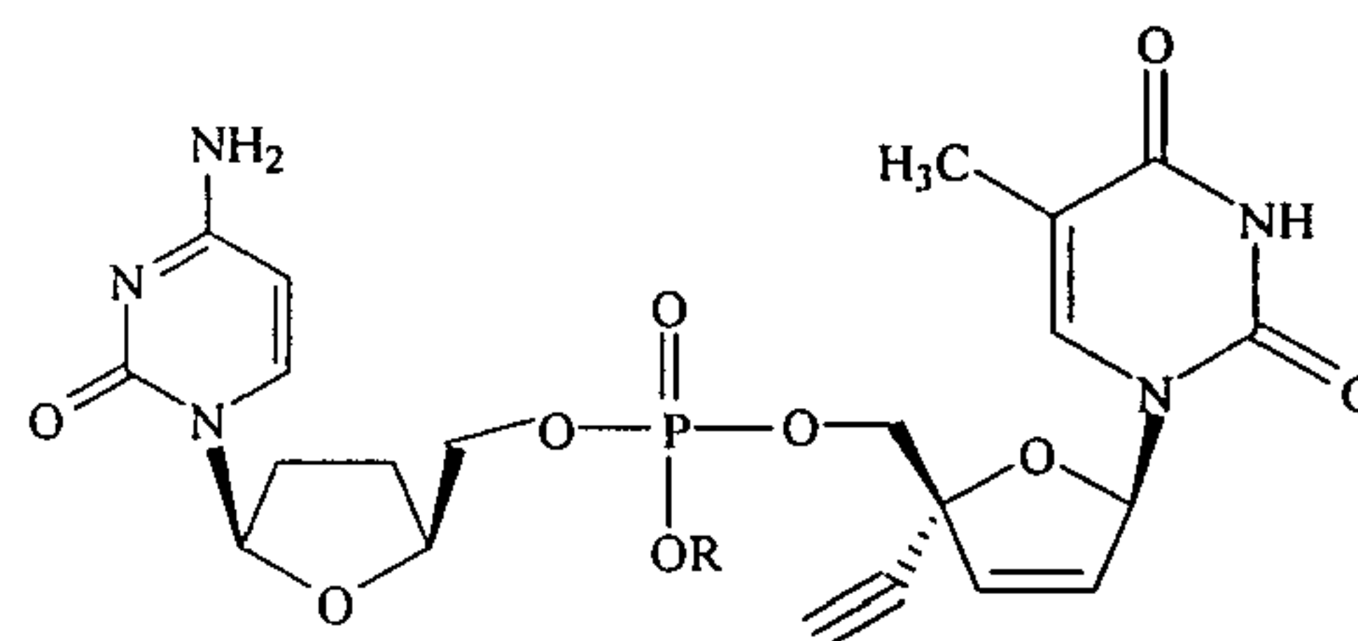
ddC and TKD-4-114 Dinucleoside Phosphate
