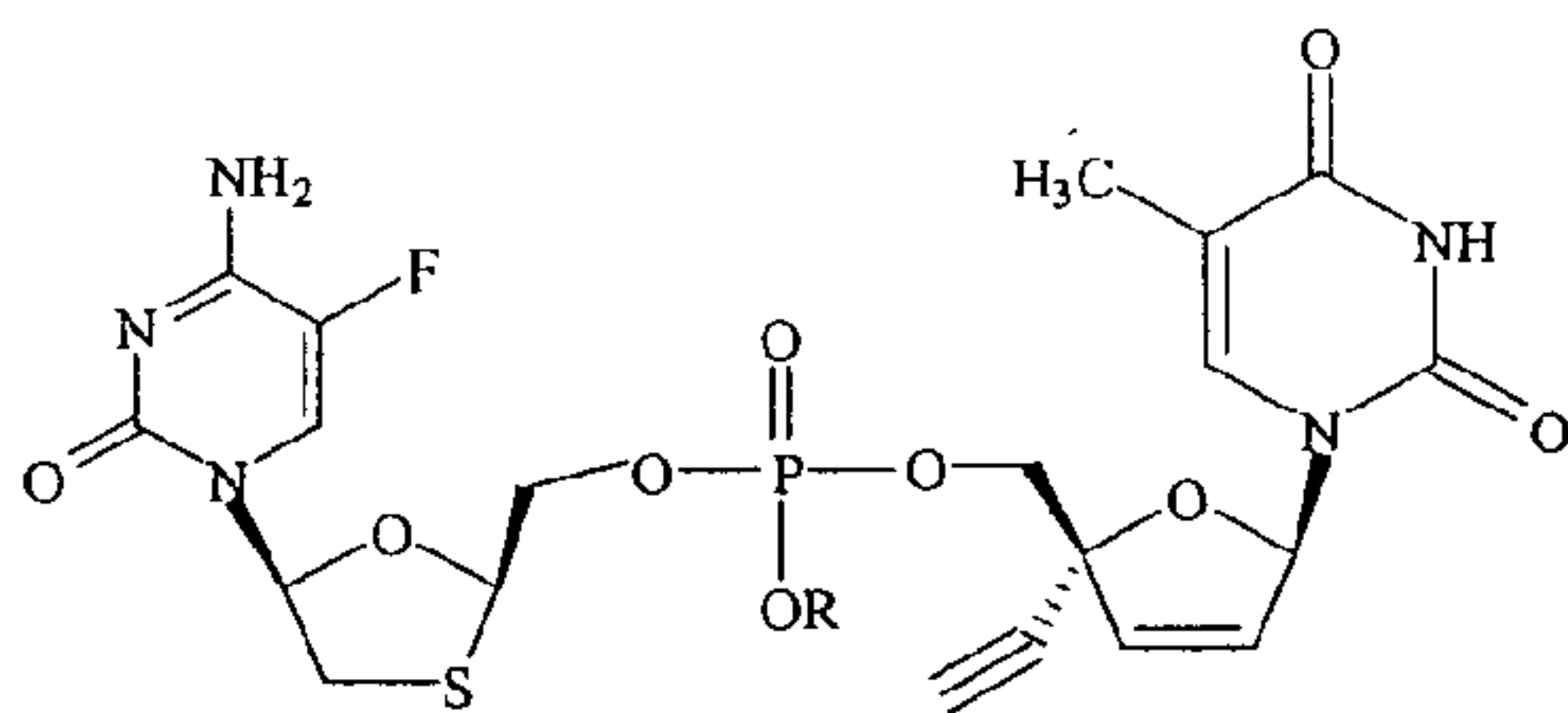
BLFd4C and TKD-4-114 Dinucleoside Phosphate
