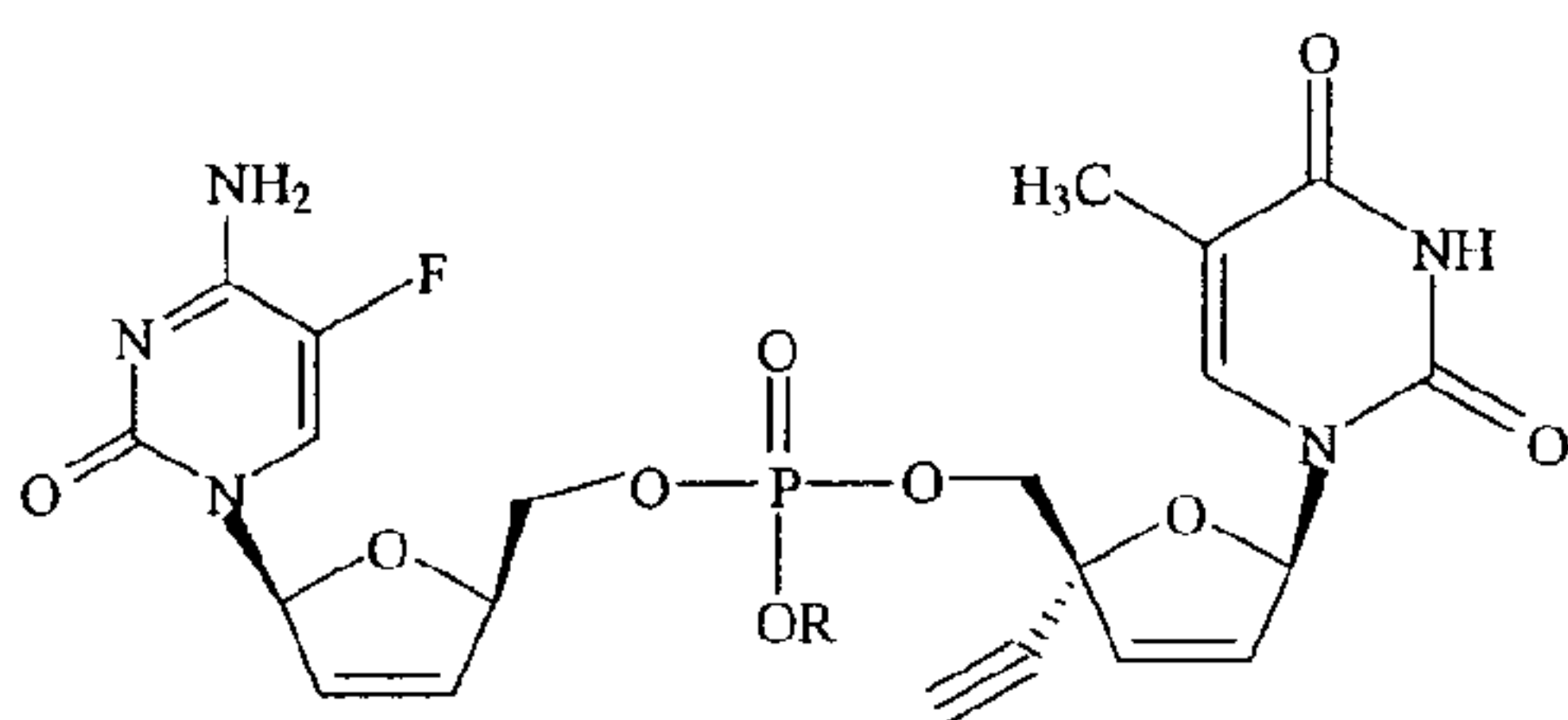
BLFd4C and TKD-4-114 Dinucleoside Phosphate
