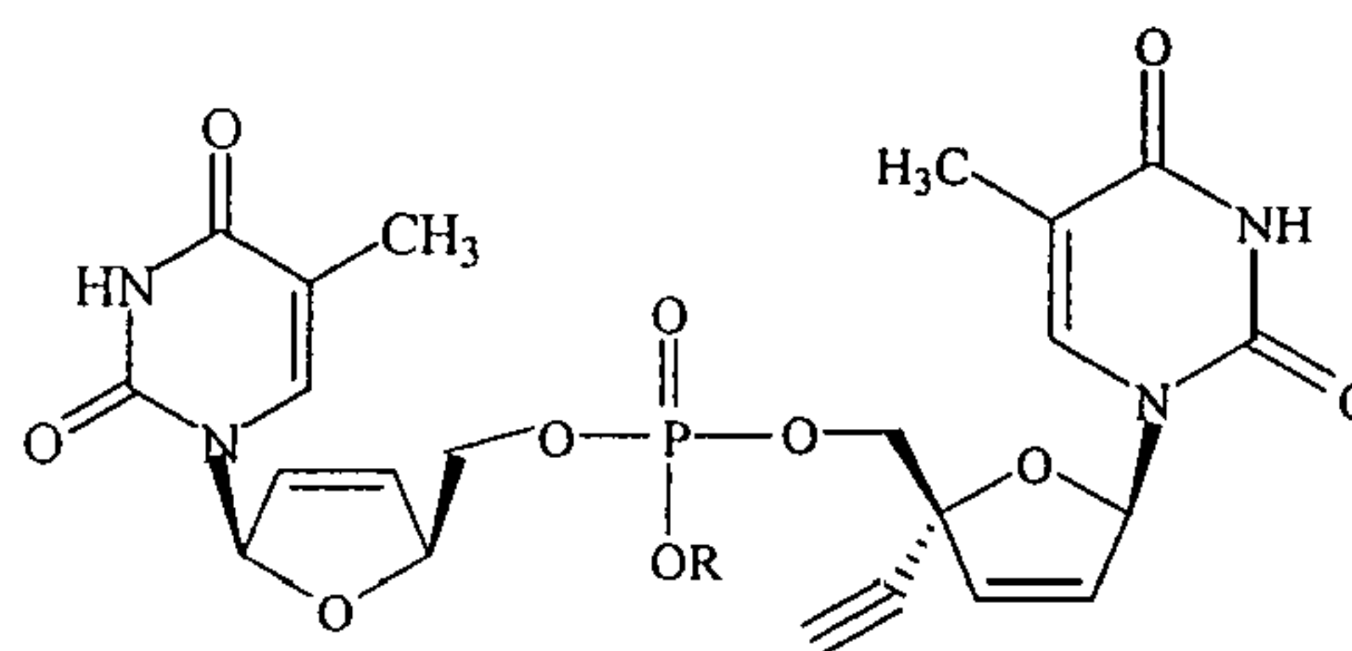
d4T and TKD-4-114 Dinucleoside Phosphate
