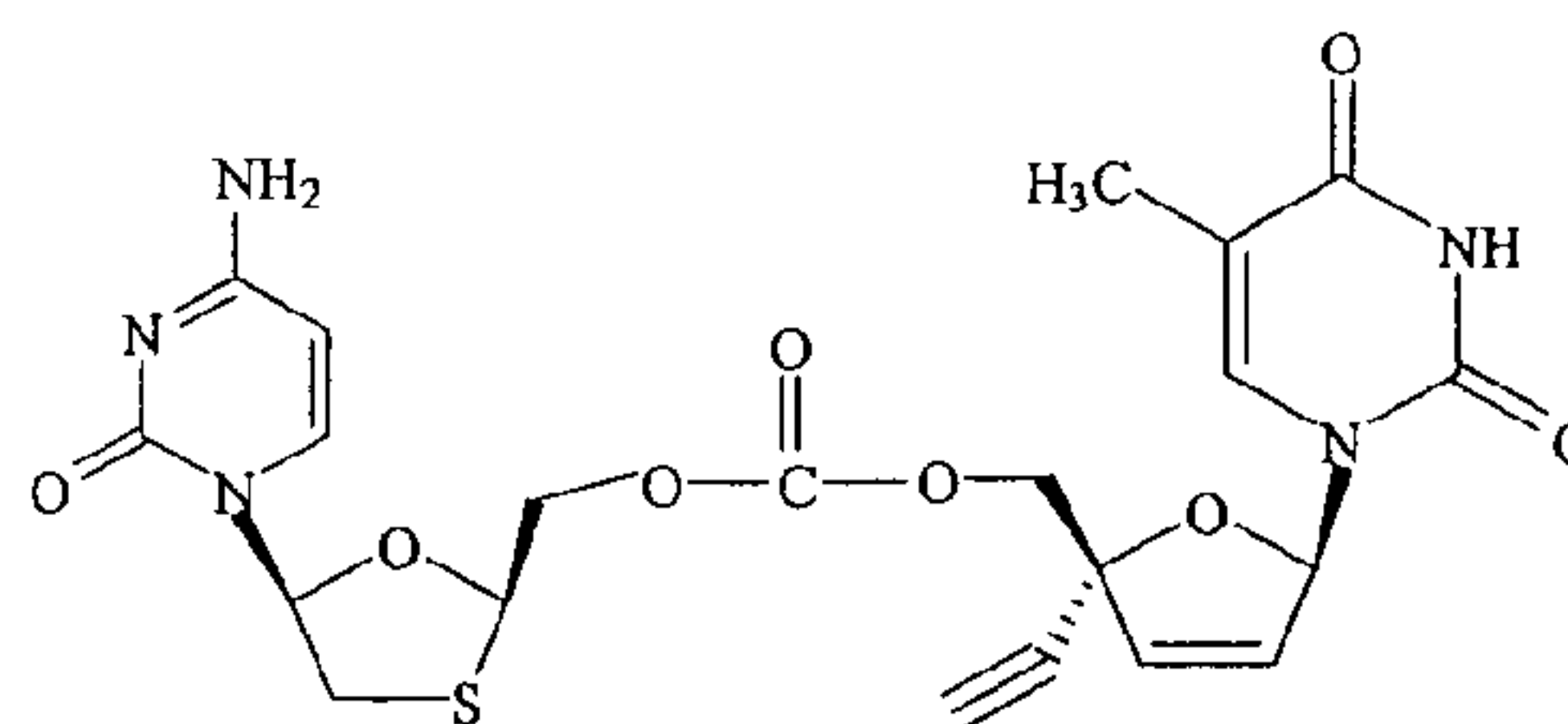
3TC and TKD-4-114 Dinucleoside Carbonate
