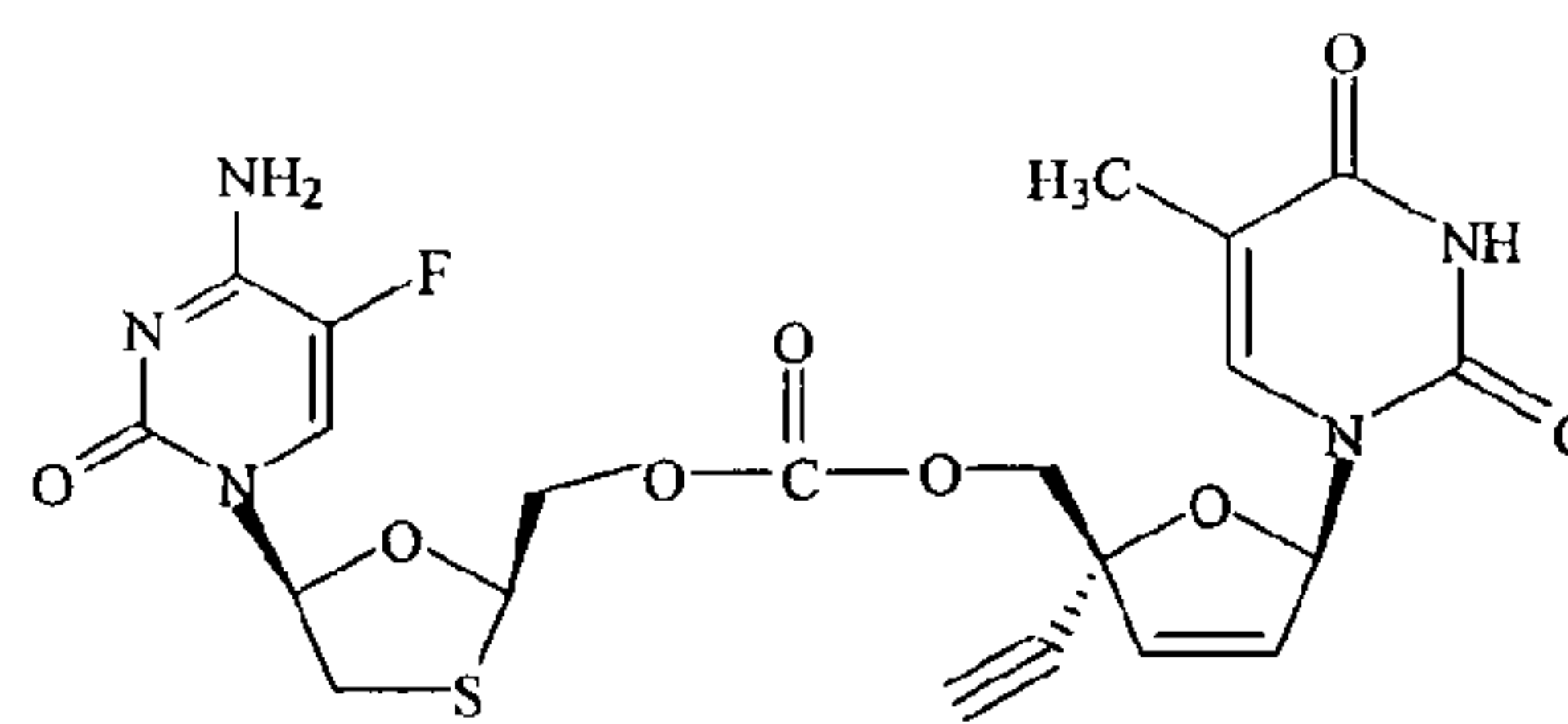
FTC and TKD-4-114 Dinucleoside Carbonate
