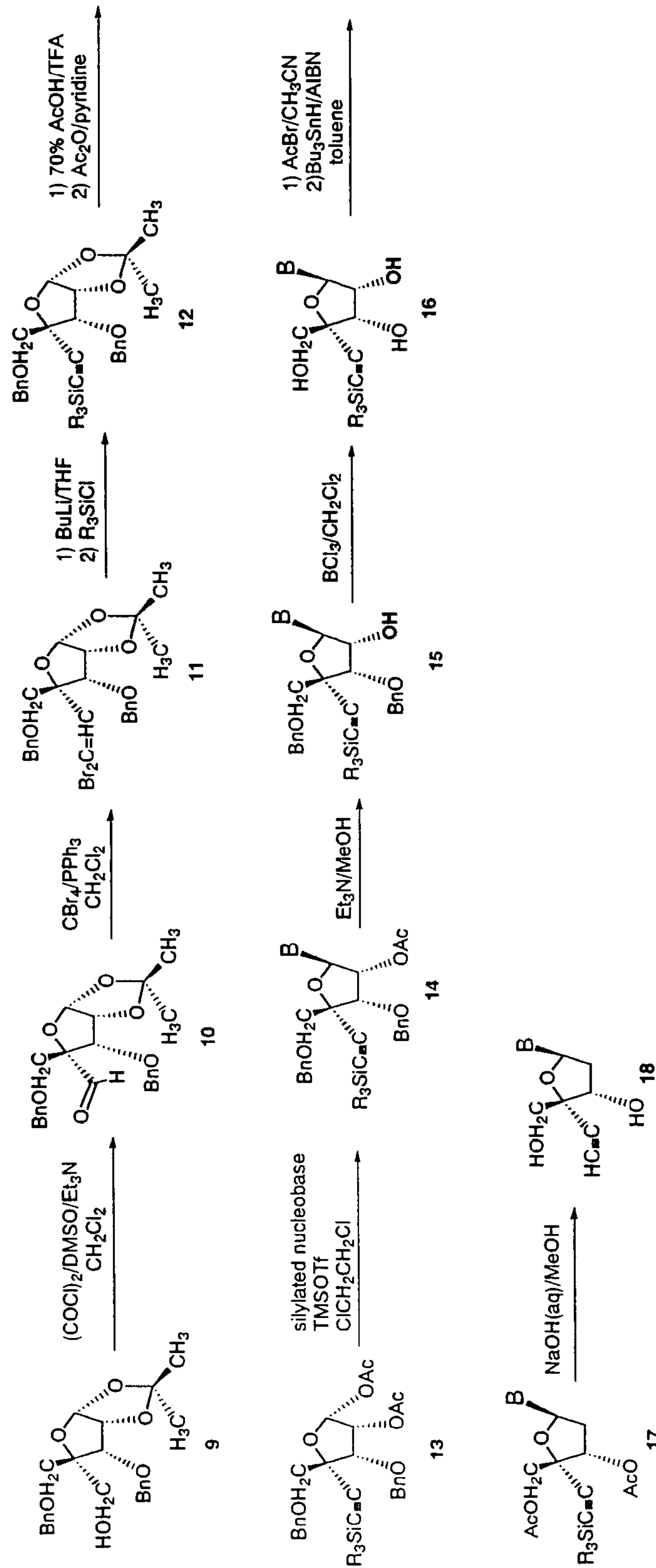
Scheme 2. Synthesis of 4'-ethynyl-2'-deoxynucleosides from sugar precursor
