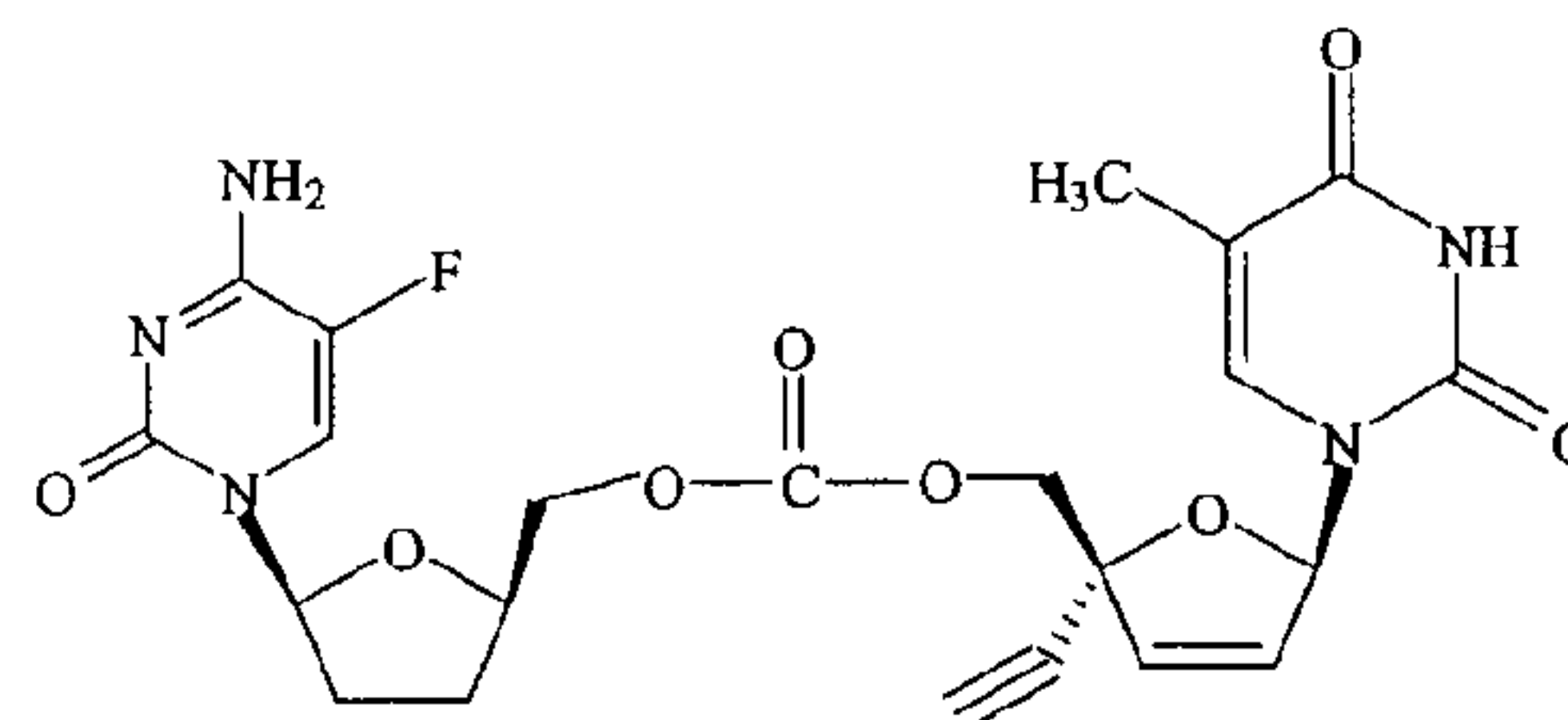
BLFddC and TKD-4-114 Dinucleoside Carbonate
