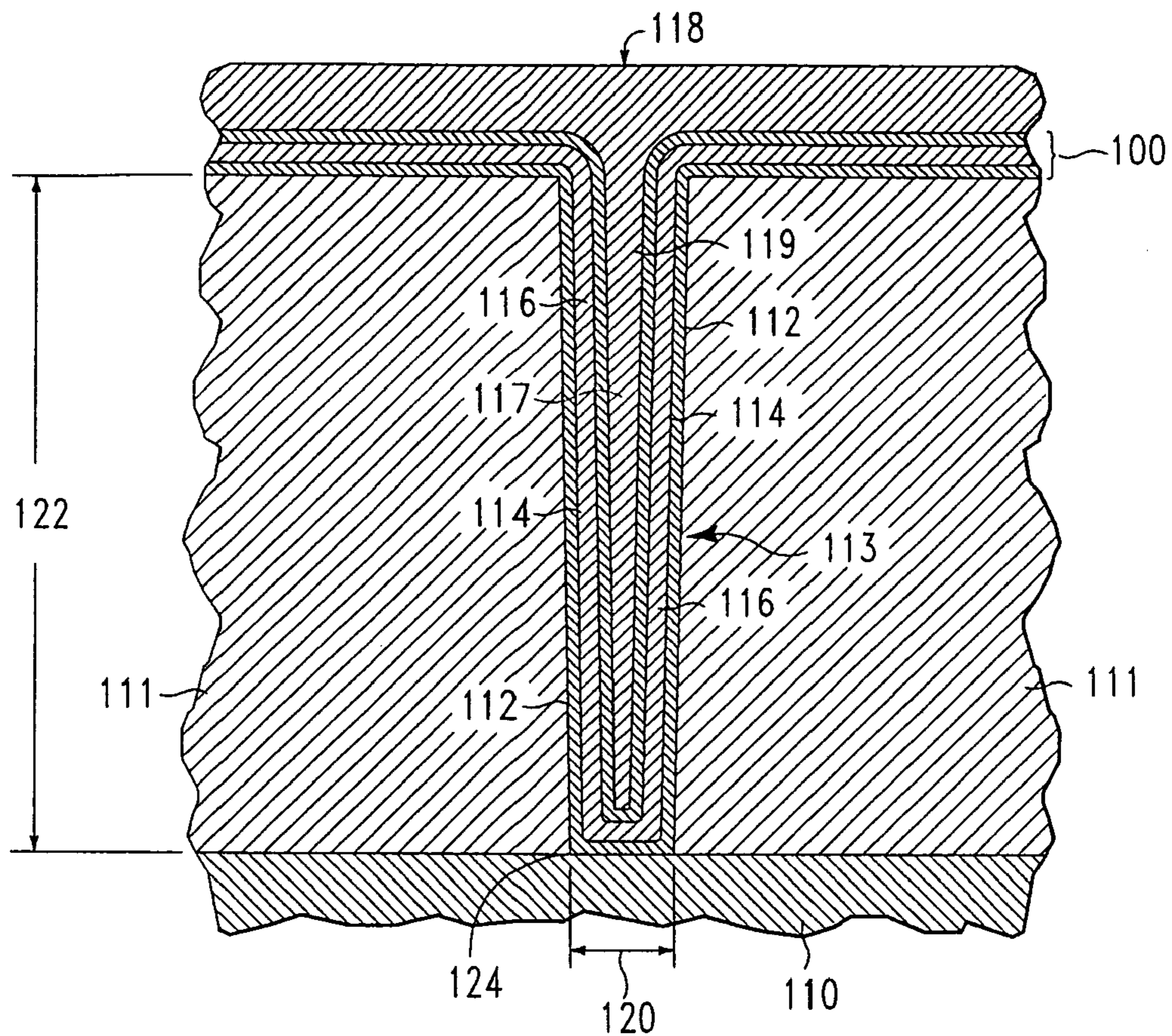
FIG. 1 (PRIOR ART)
