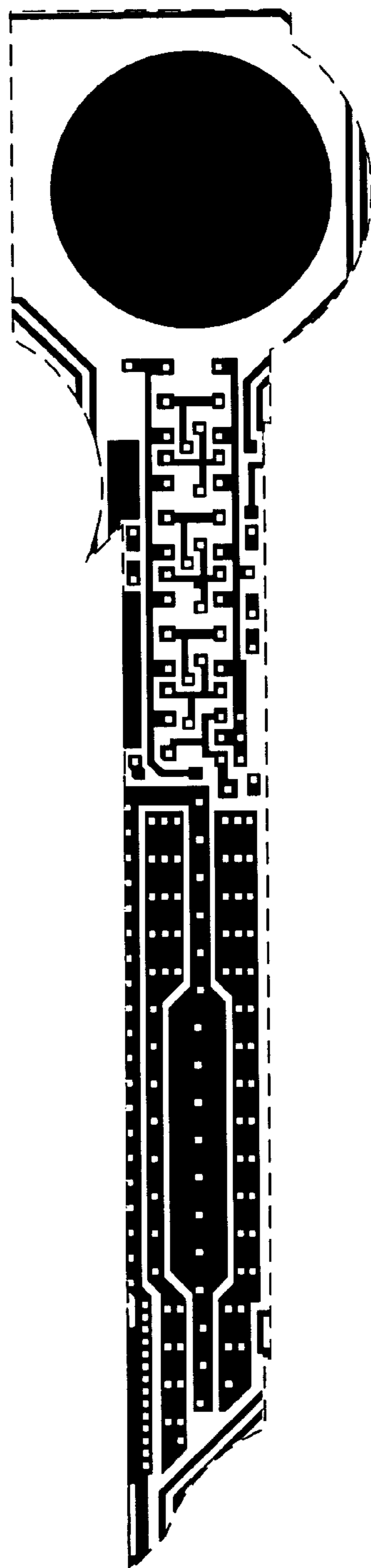
Metal 1 mask
