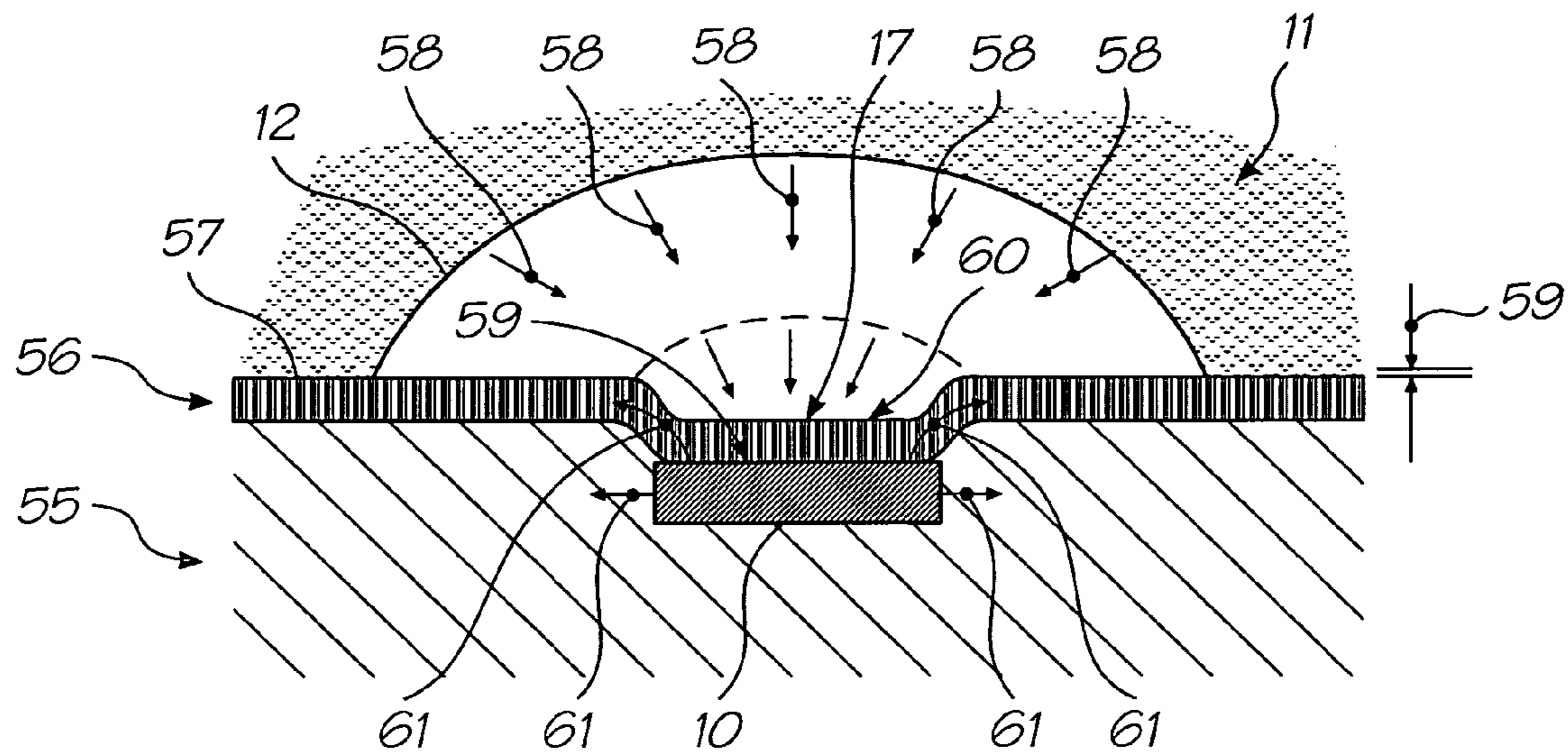
FIG. 47 (PRIOR ART)
