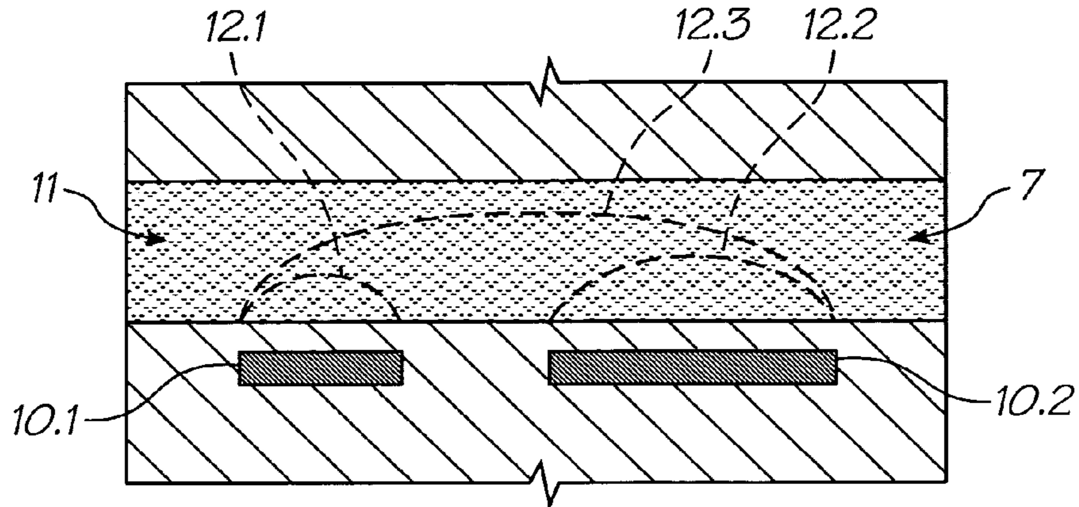
FIG. 52 (PRIOR ART)
