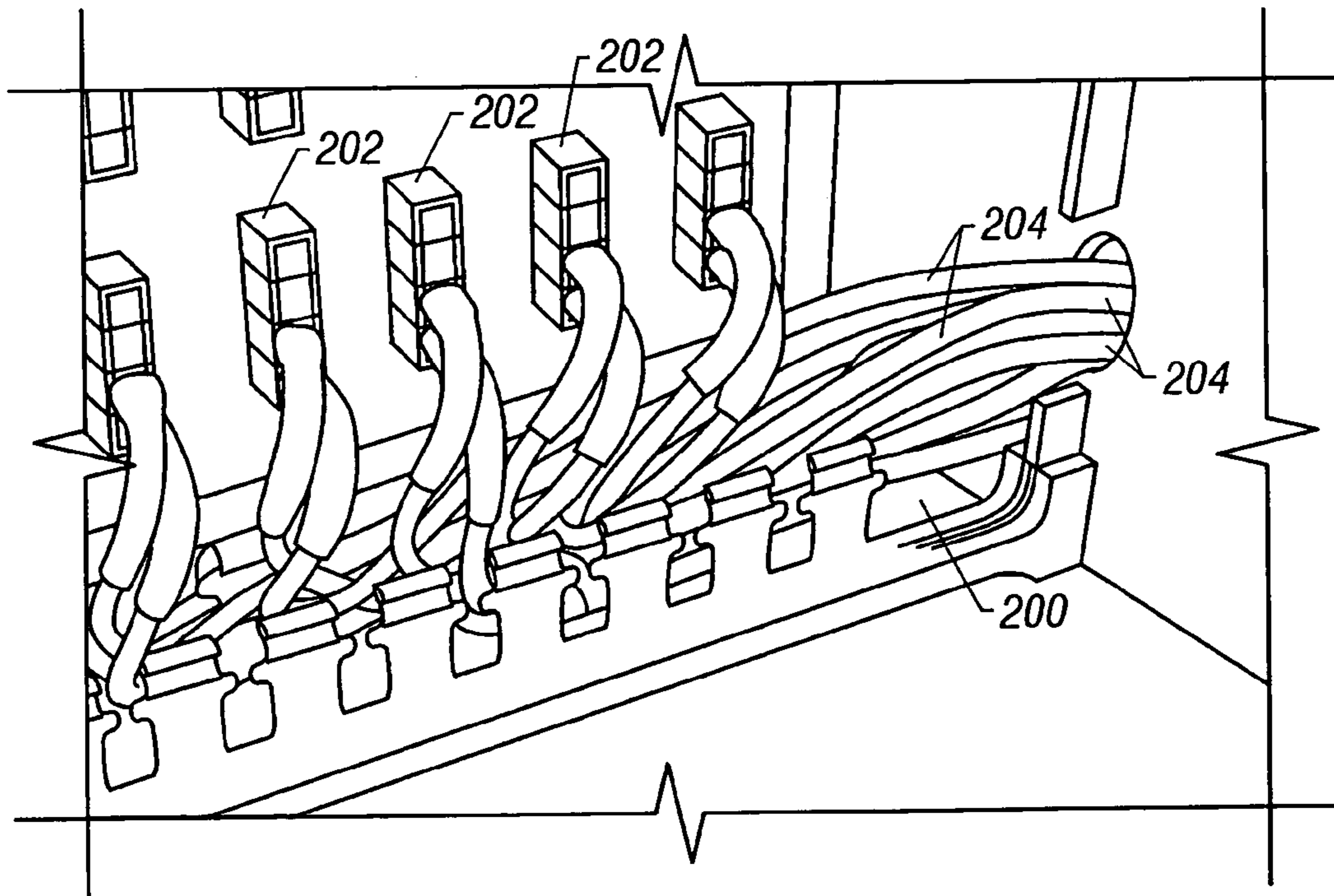
FIG. 2 (Prior Art)
