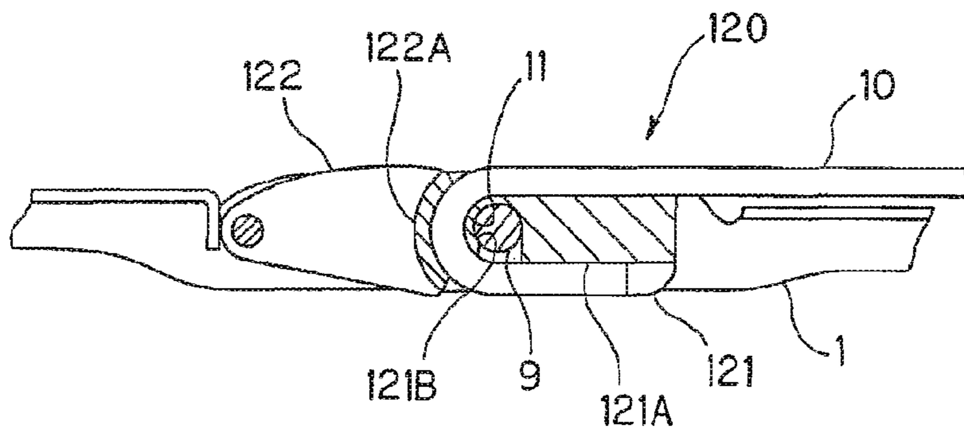
FIG. 19(C) (PRIOR ART)
