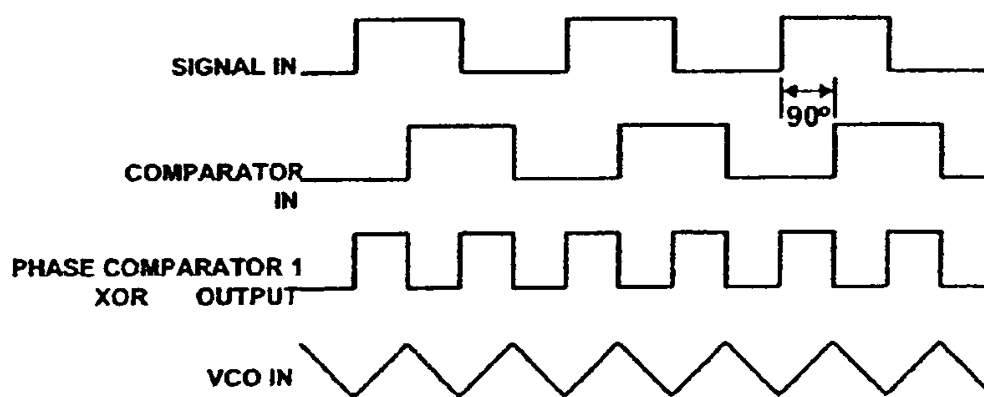
(C) TYPICAL XOR DETECTOR WAVEFORMS
