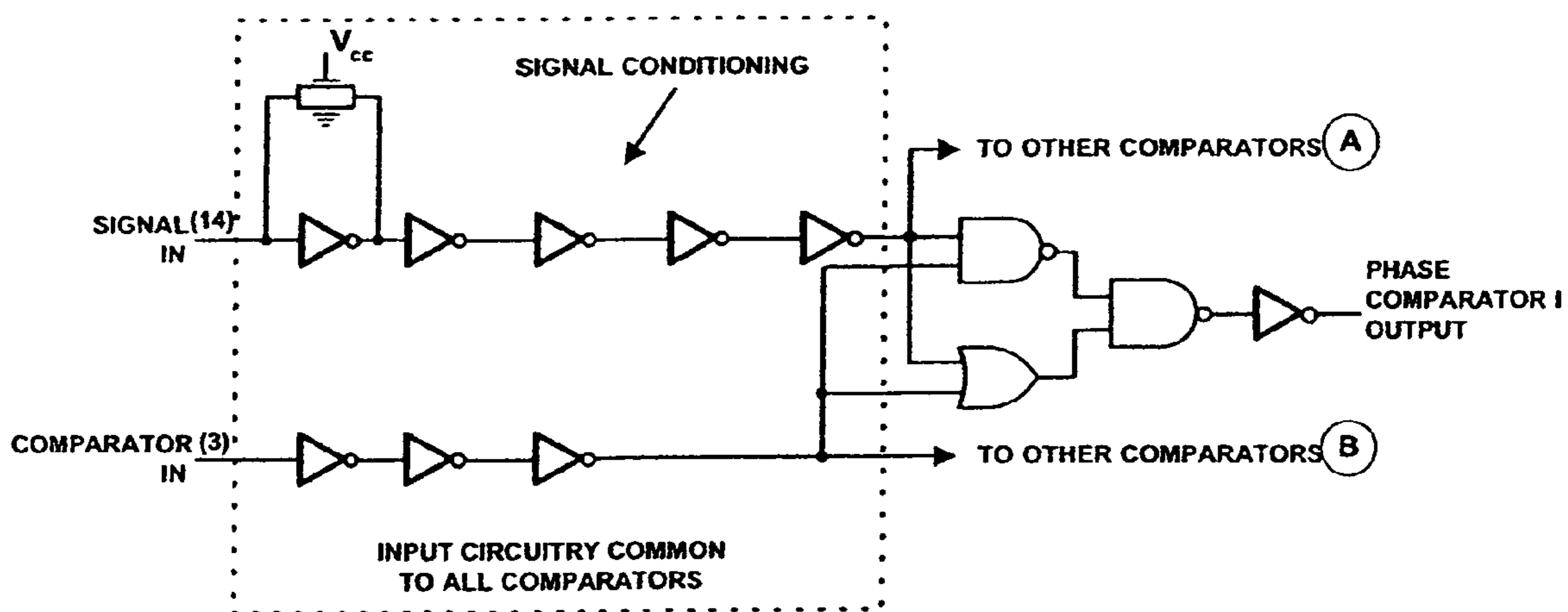
(B) DETAILED ON-CHIP IC CIRCUITRY IN 74HC4046
