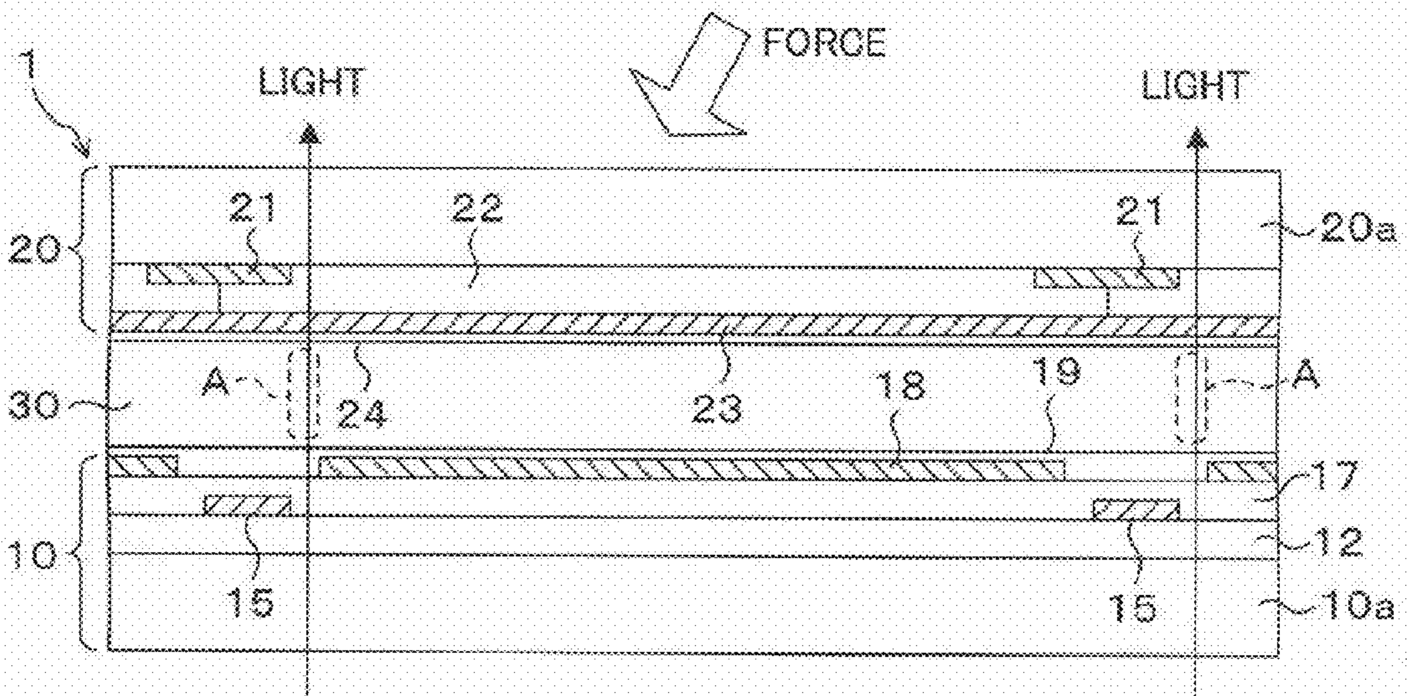
FIG. 3 (PRIOR ART)
