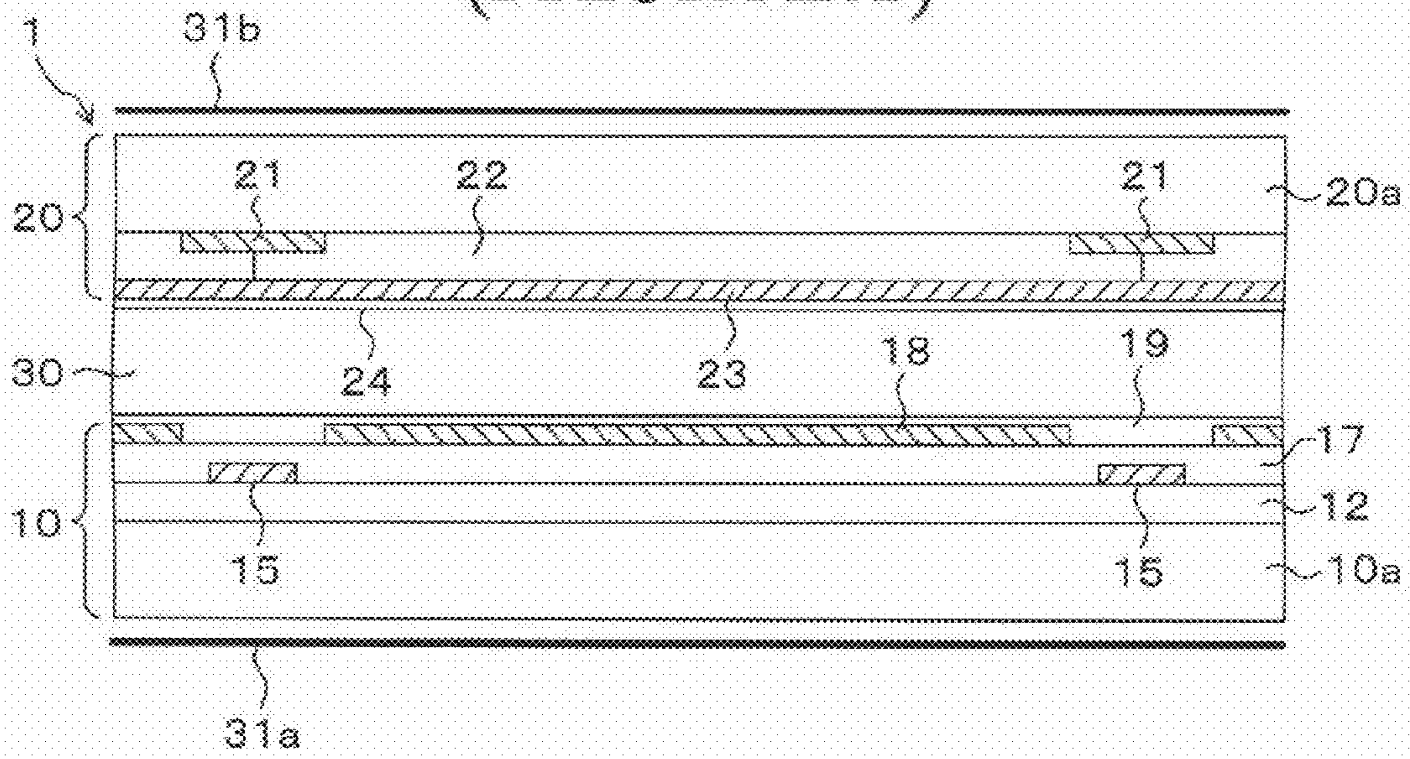
FIG. 2 (PRIOR ART)
