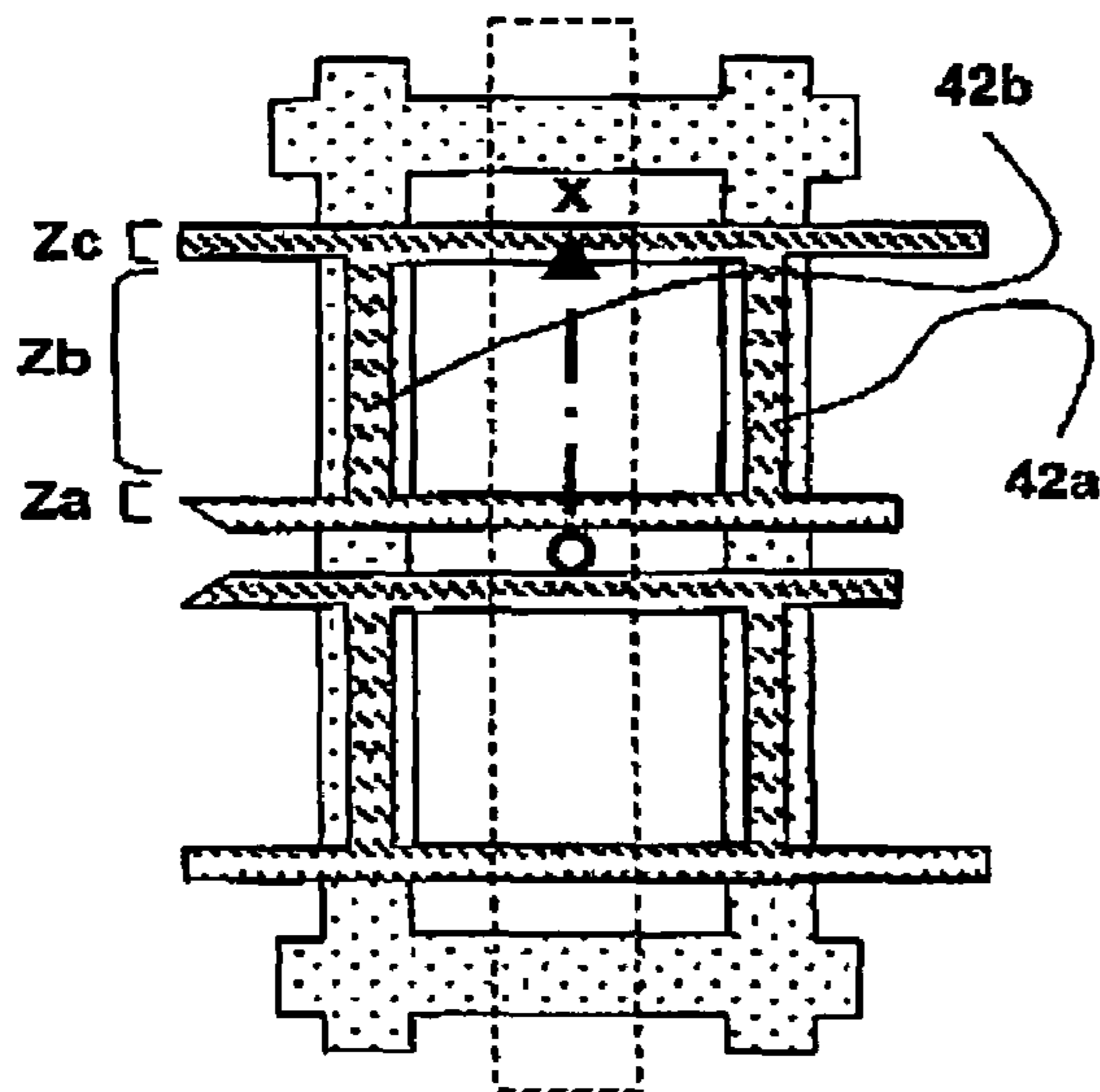
PRIOR ART Fig.4-A
