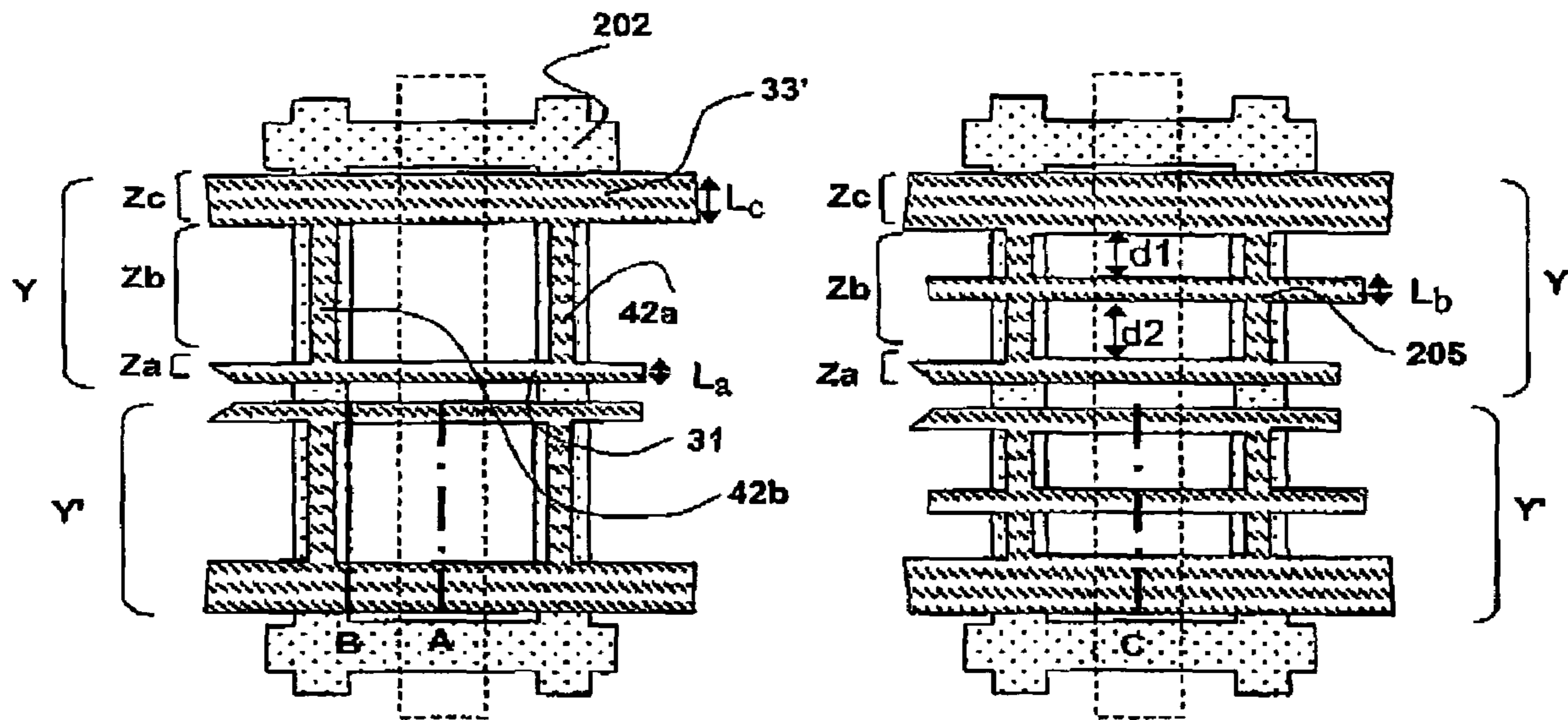
PRIOR ART Fig.20A
