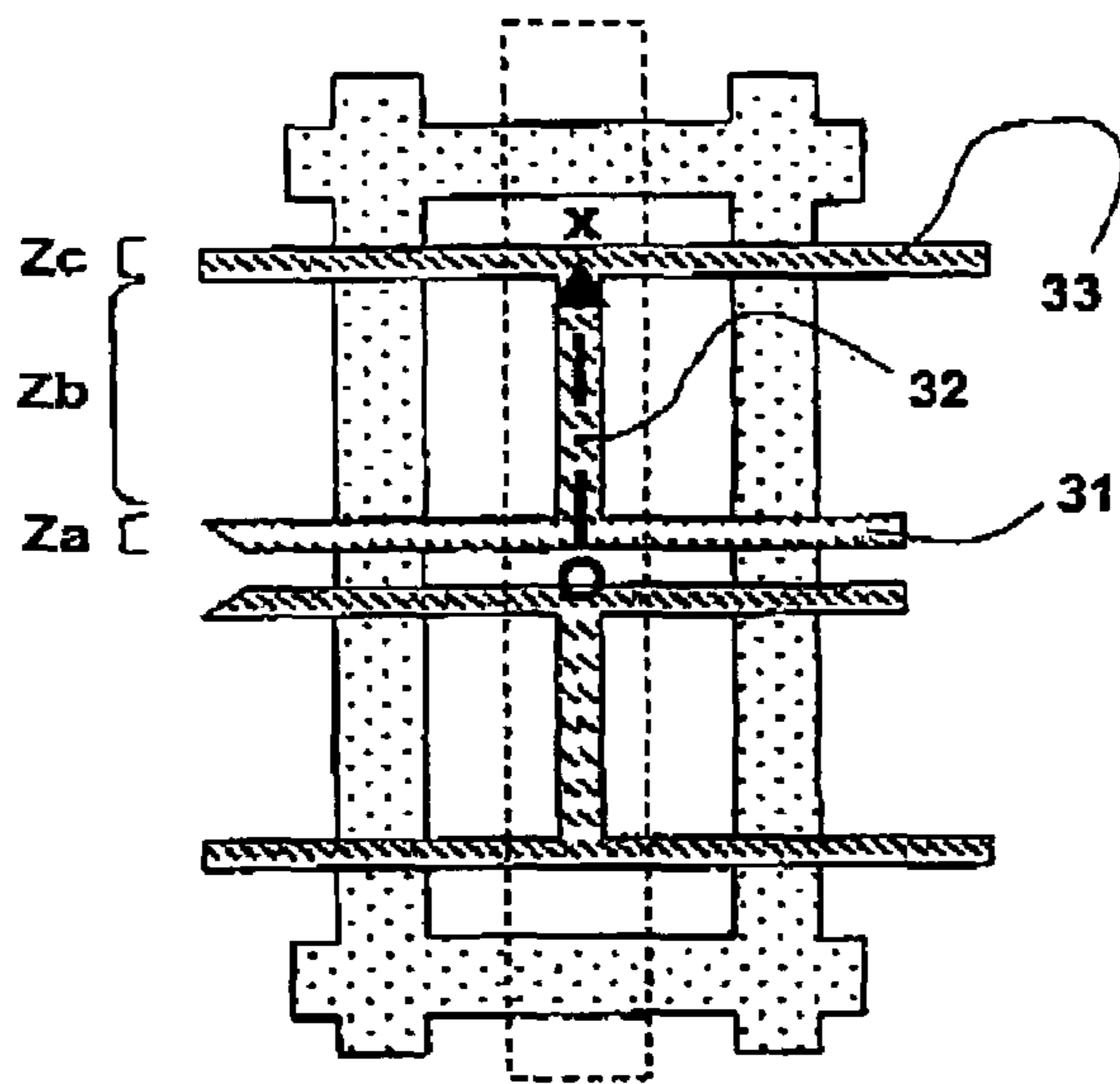
PRIOR ART Fig.3-A
