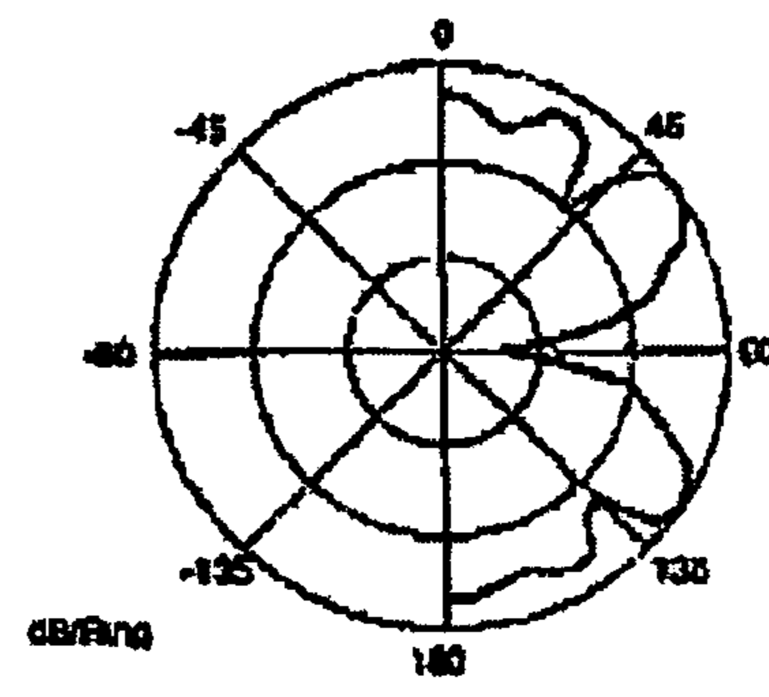
450 MHz
