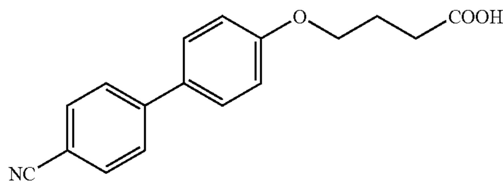
[(4'-cyano-1,1'-biphenyl-4-yl)oxy]butyric acid
