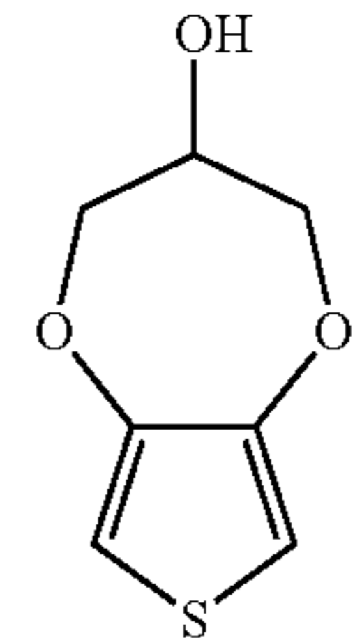
hydroxy-PDT
