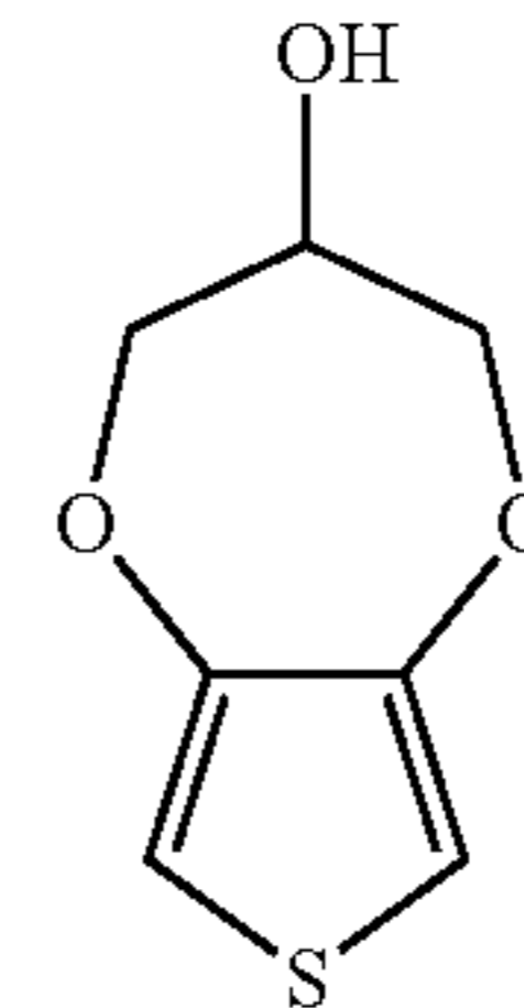
hydroxy-PDT
