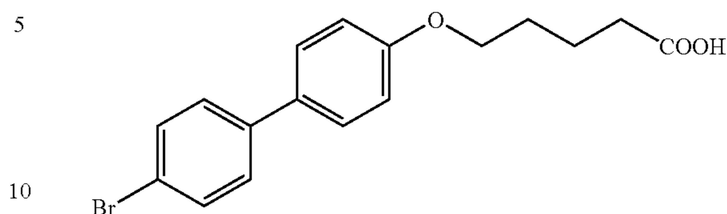
[(4'-bromo-1,1'-biphenyl-4-yl)oxy]valeric acid
