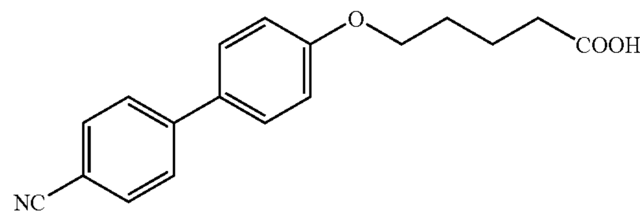
[(4'-cyano-1,1'-biphenyl-4-yl)oxy]valeric acid
