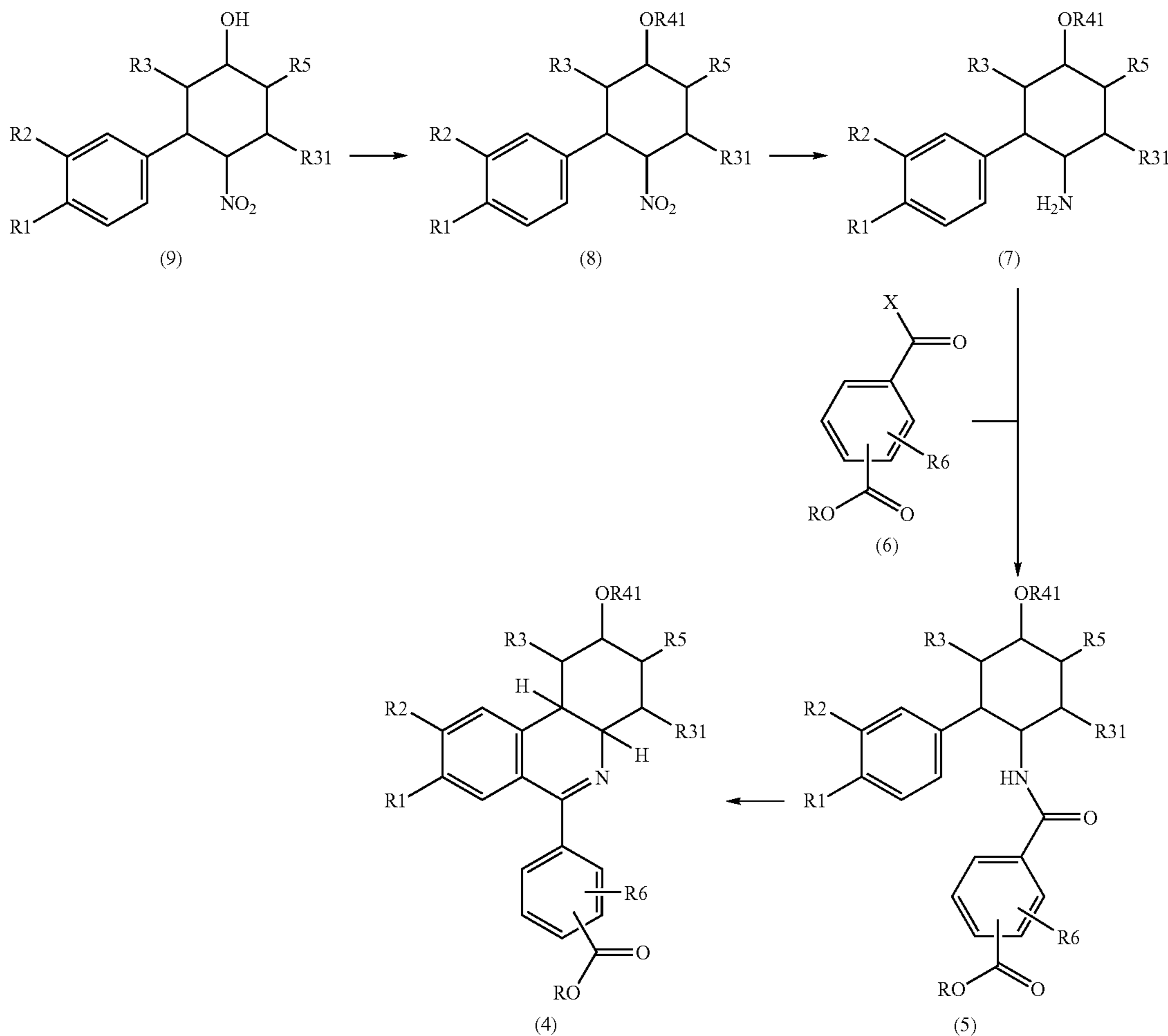
Reaction scheme 3:
