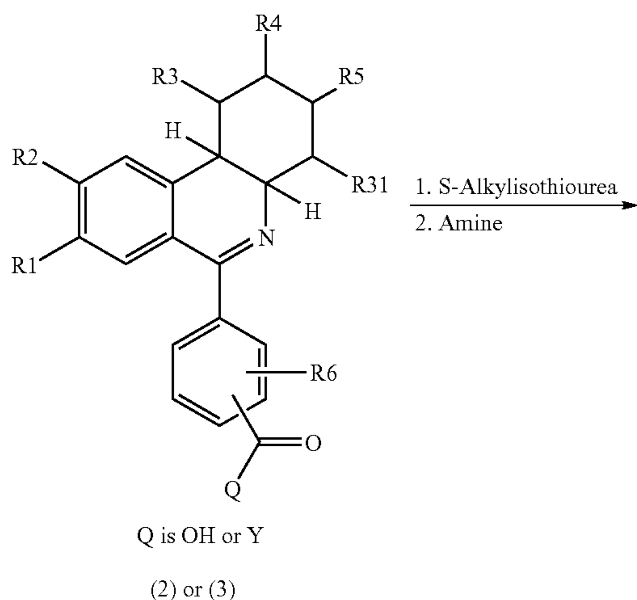
Reaction scheme 2:
