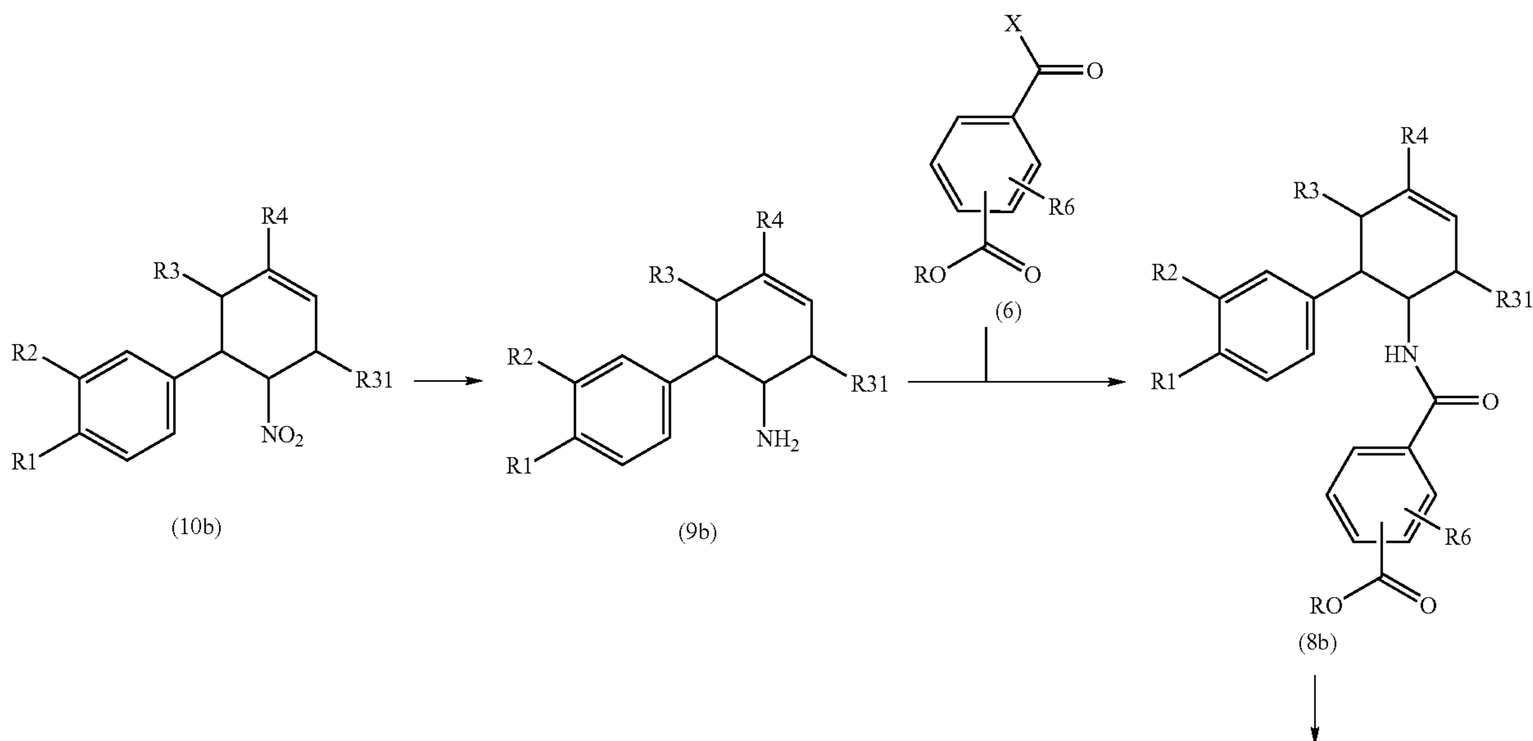
Reaction scheme 5:
