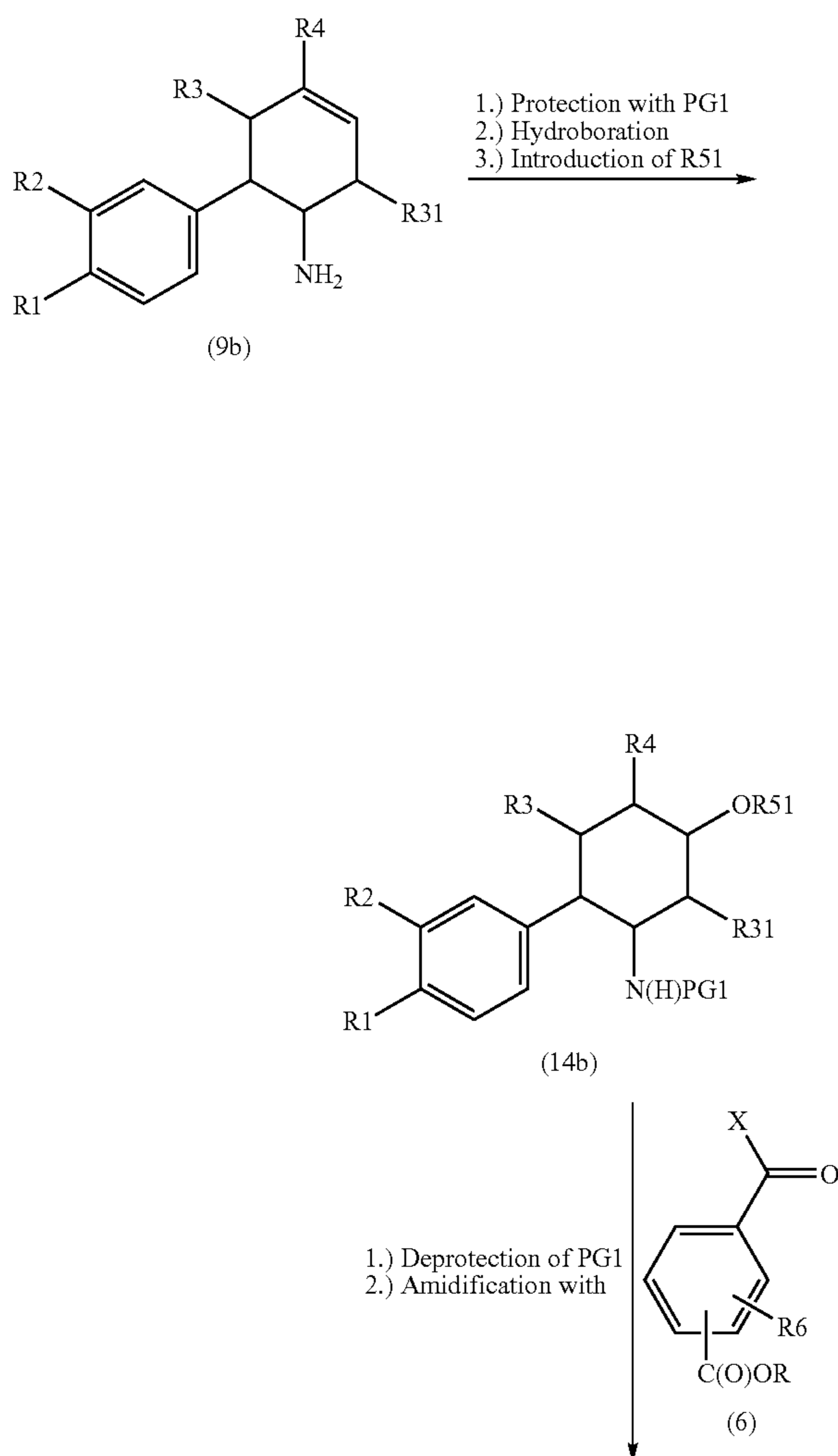
Reaction scheme 8:
