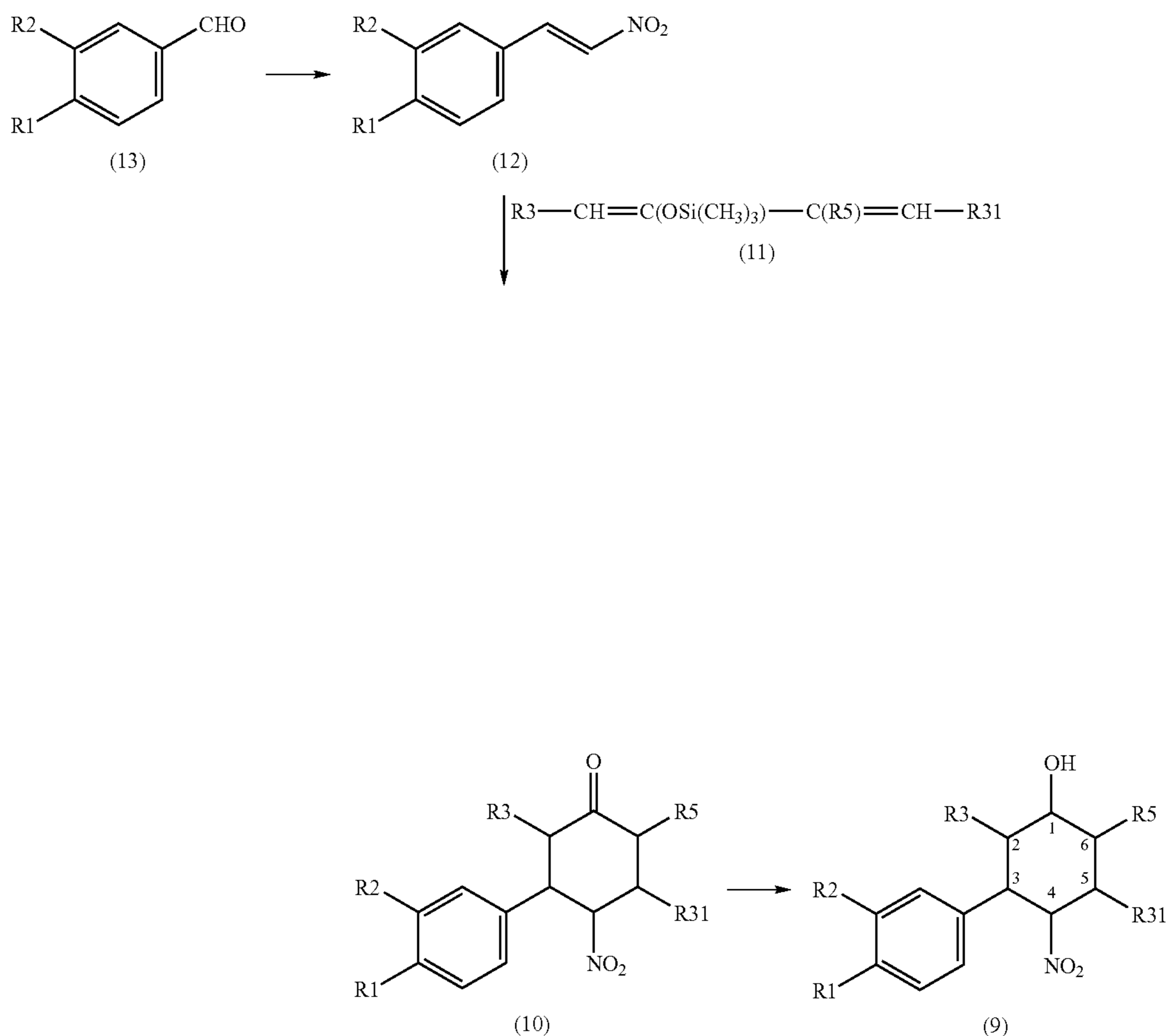
Reaction scheme 4:
