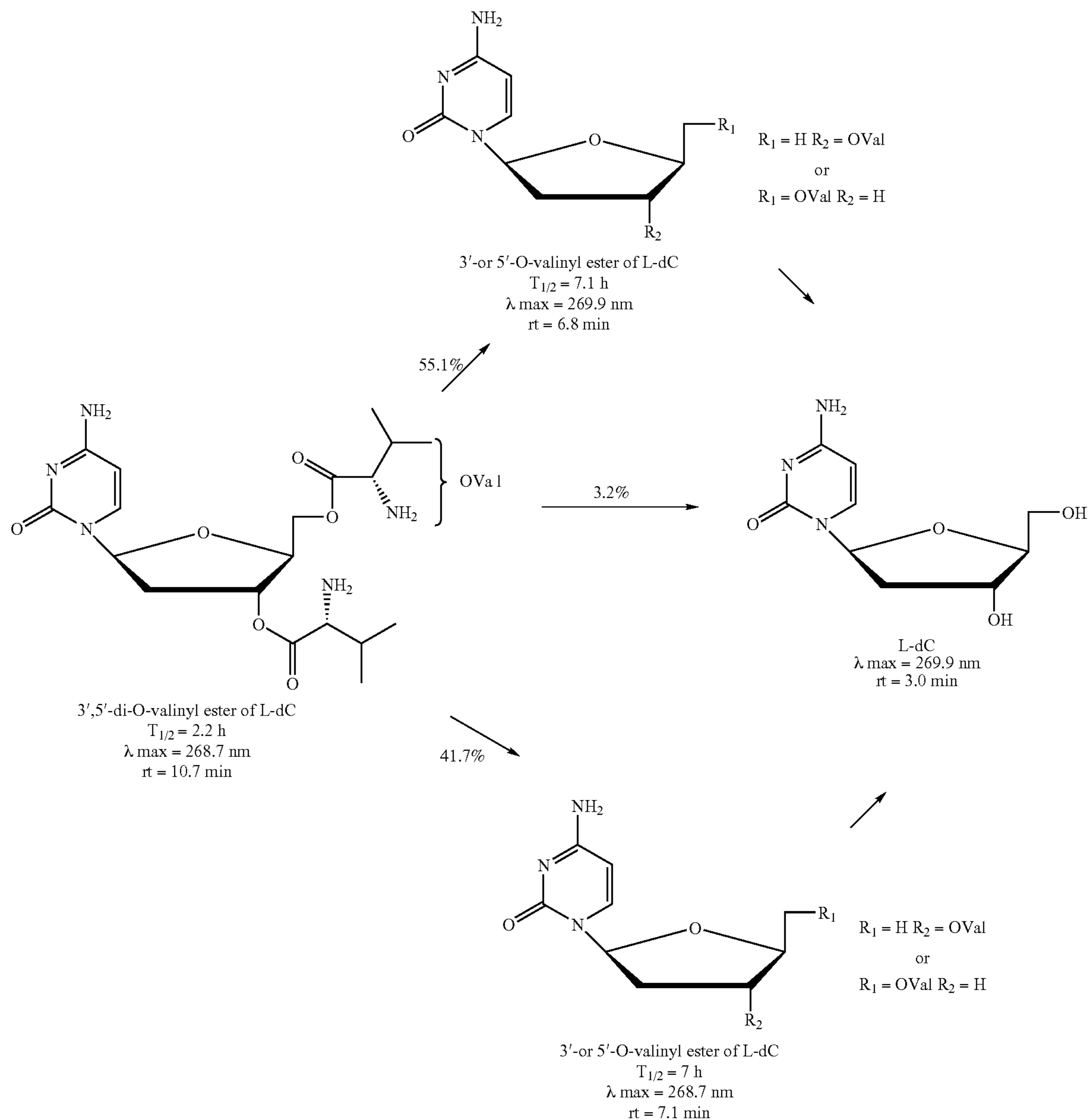
Scheme 5
