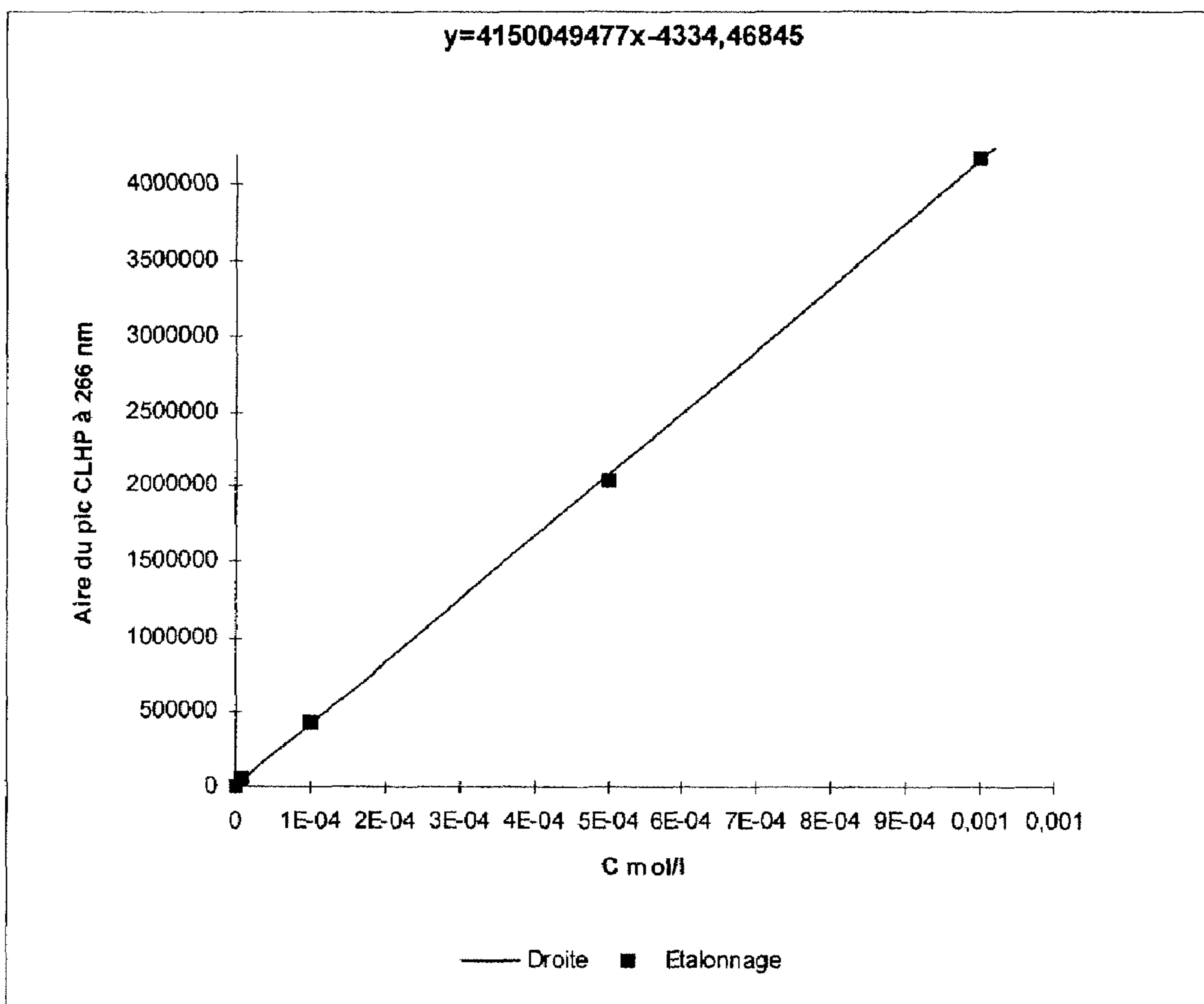
Figure 8a: Solubility Calibration Curve for D-dC
