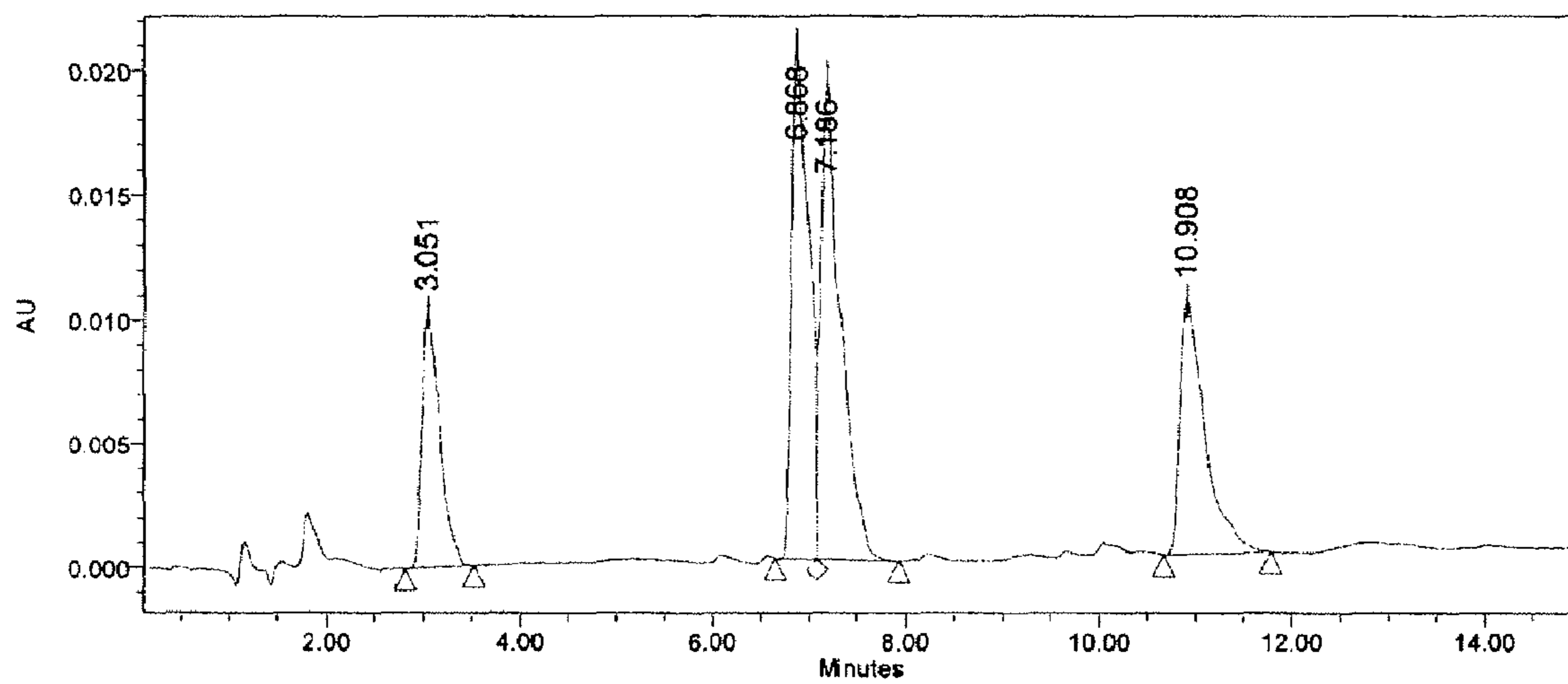
Figure 11a: HPLC profile – 95.7 hours at pH of 4.51
