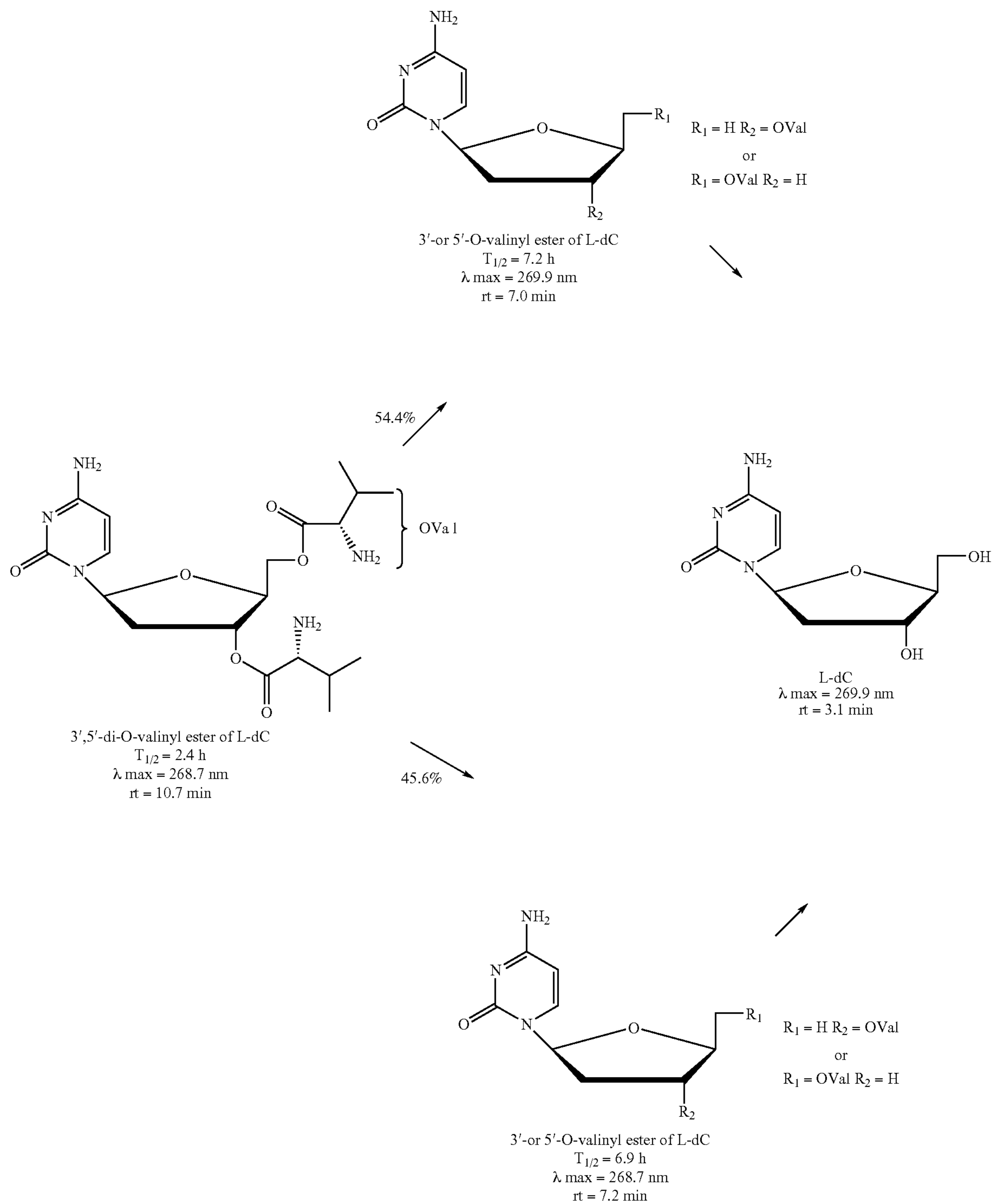
Scheme 4
