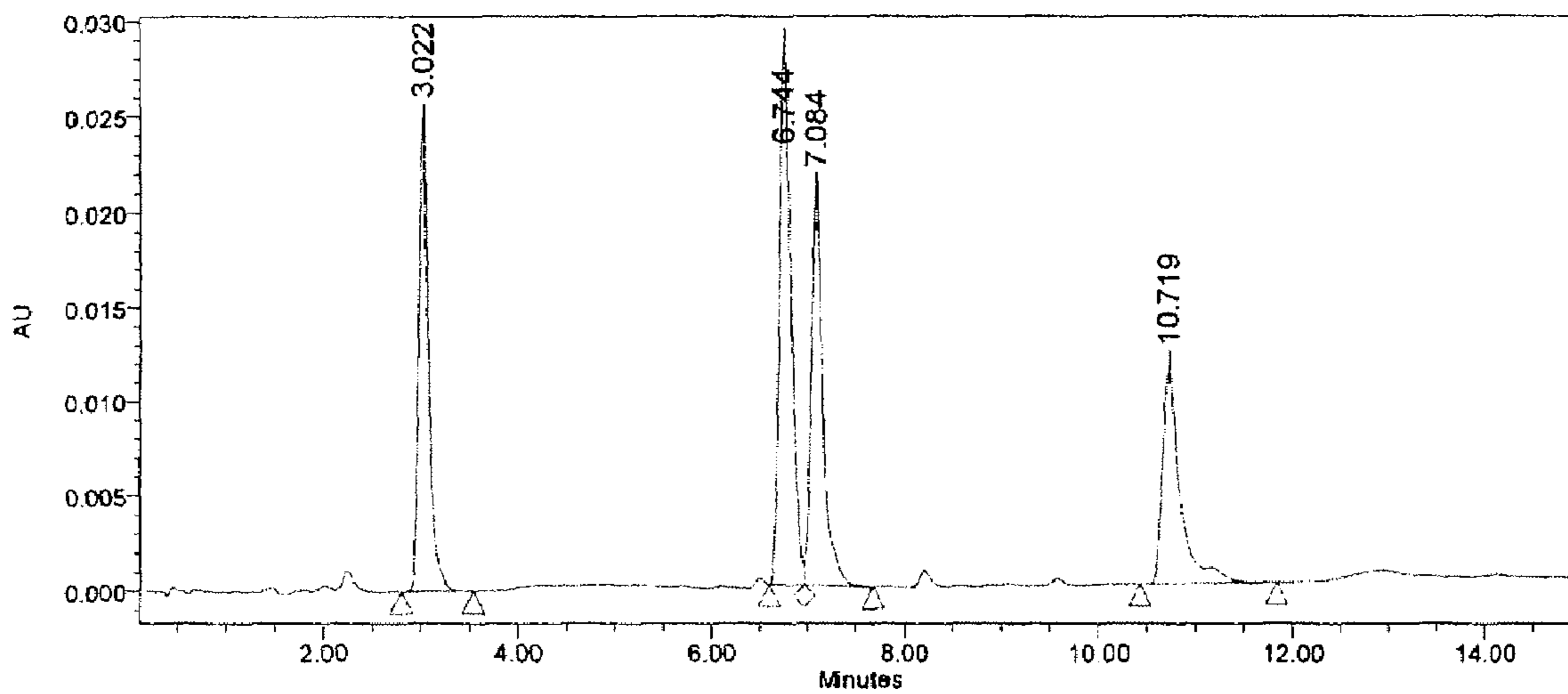
Figure 9a: HPLC profile – 7.5 hours at pH of 7.42
