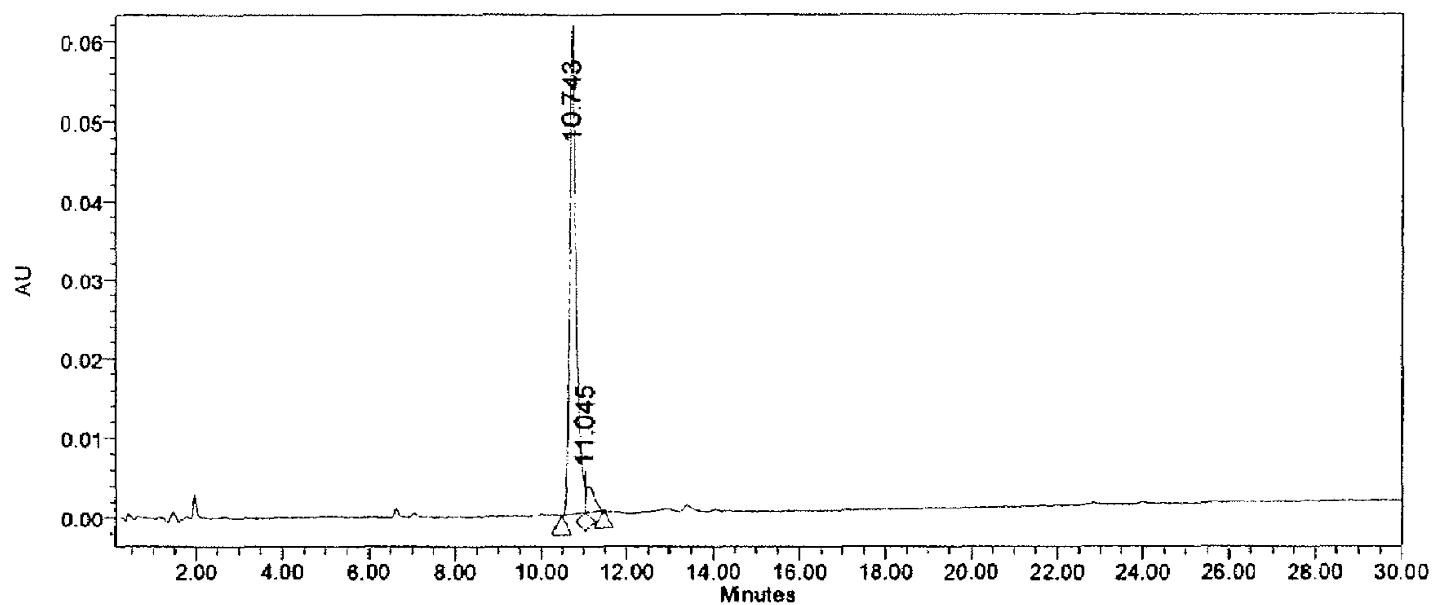
Figure 12: HPLC profile ~ 48 hours at pH of 1.23
