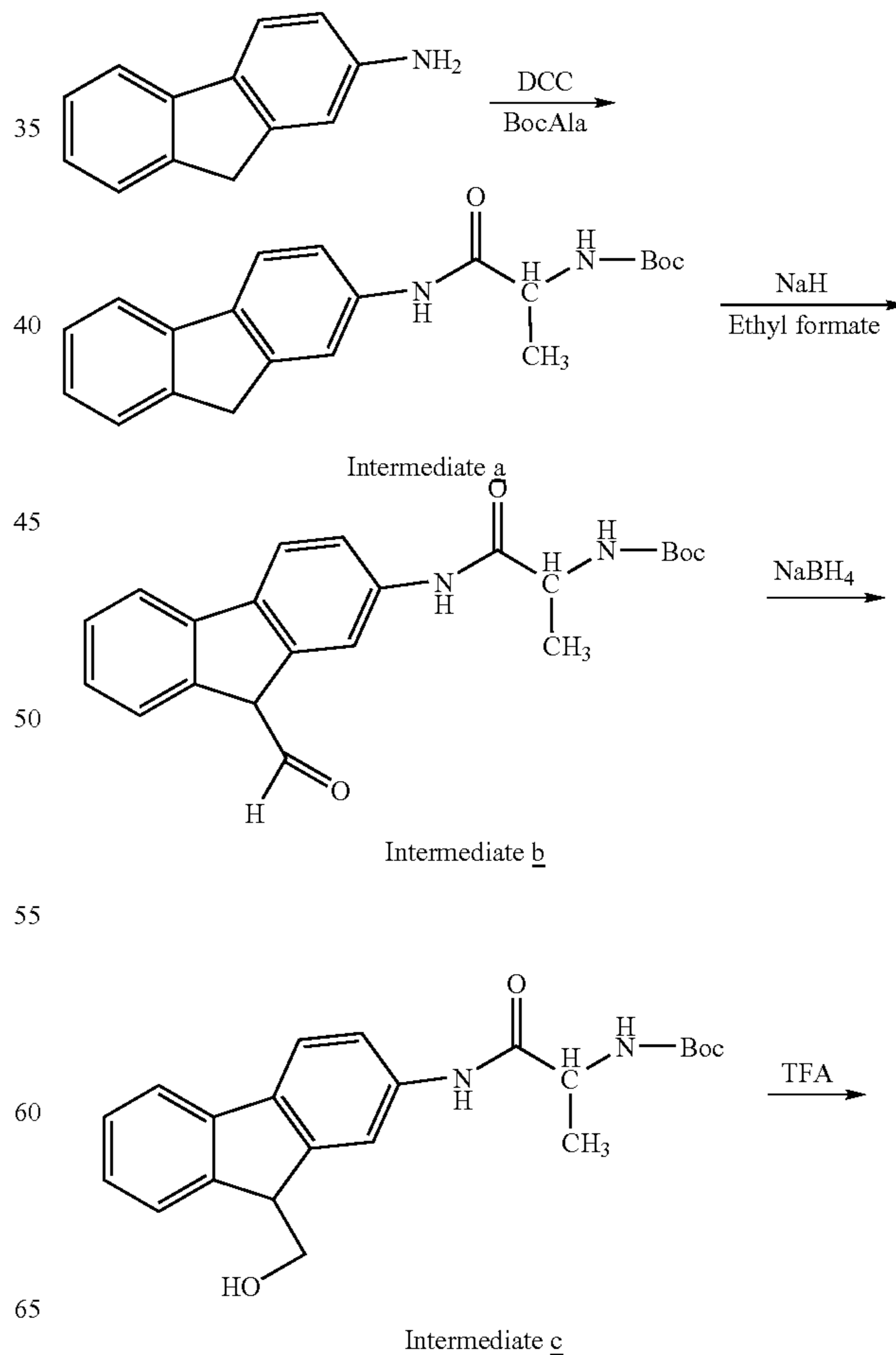
Scheme 2: Synthesis of Precursors 1-4
