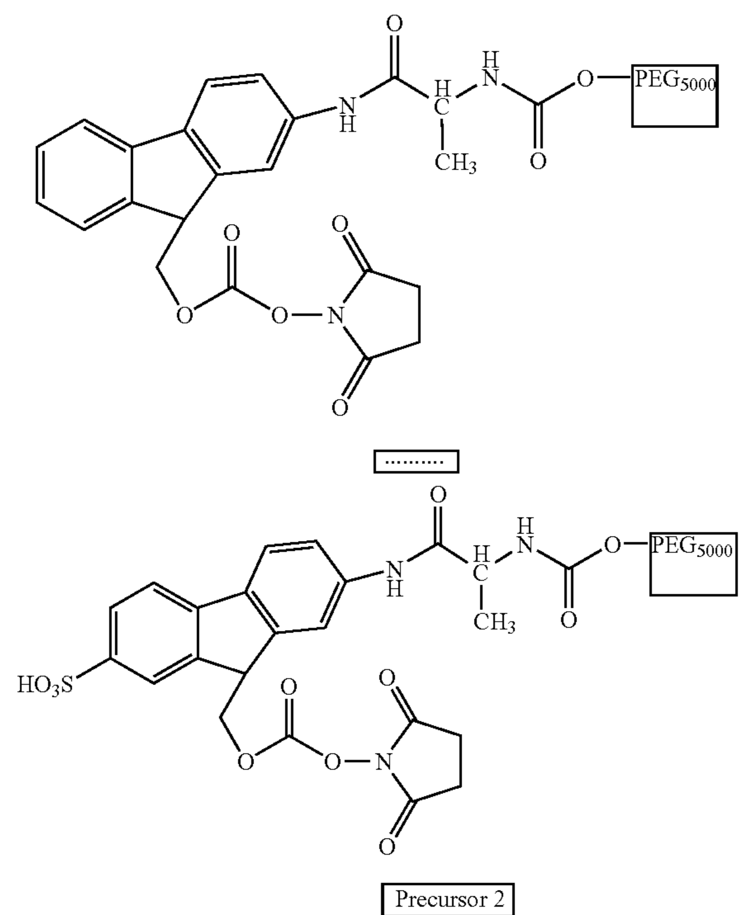
Scheme 1: Precursors 1-4
