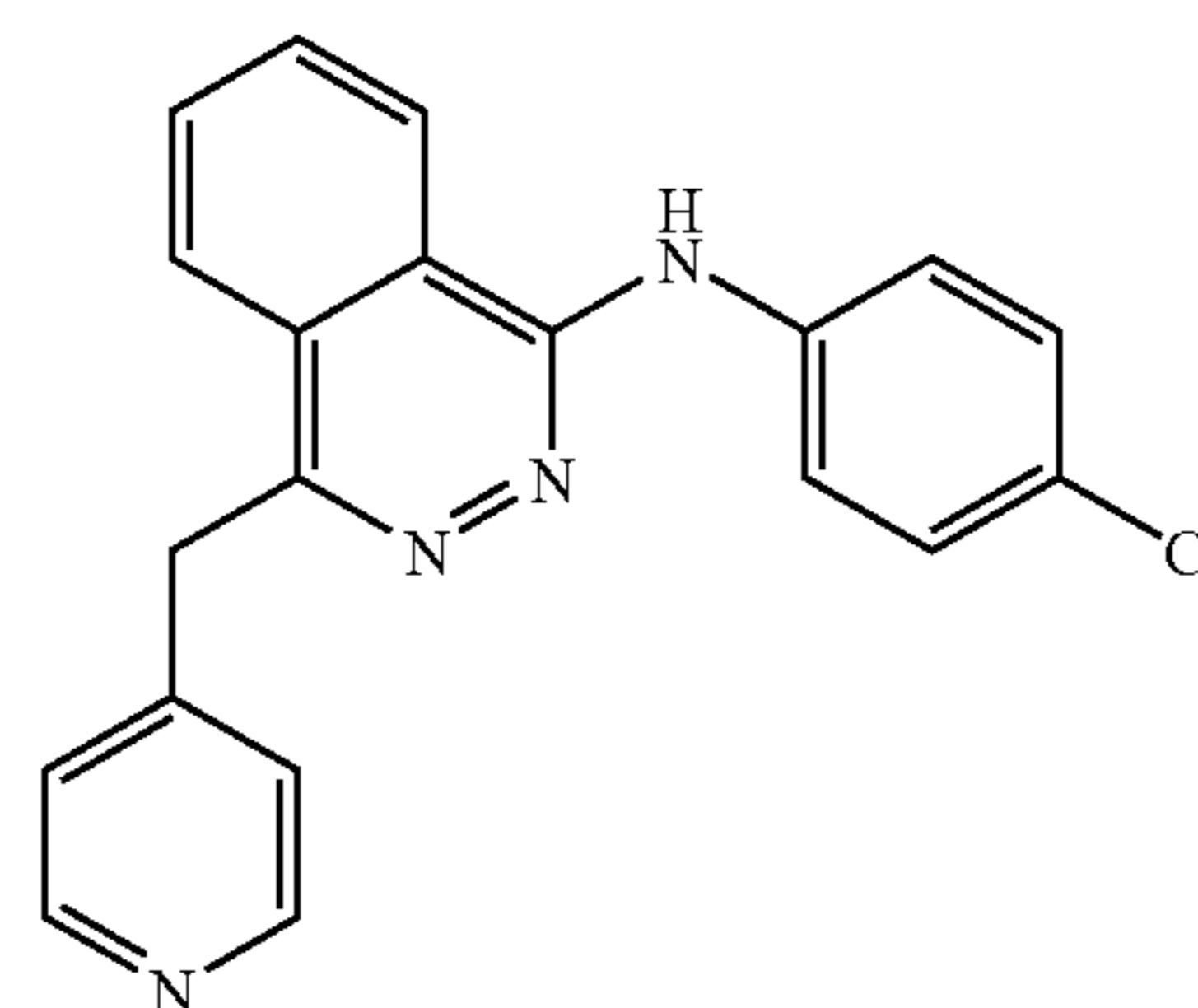
PTK787
