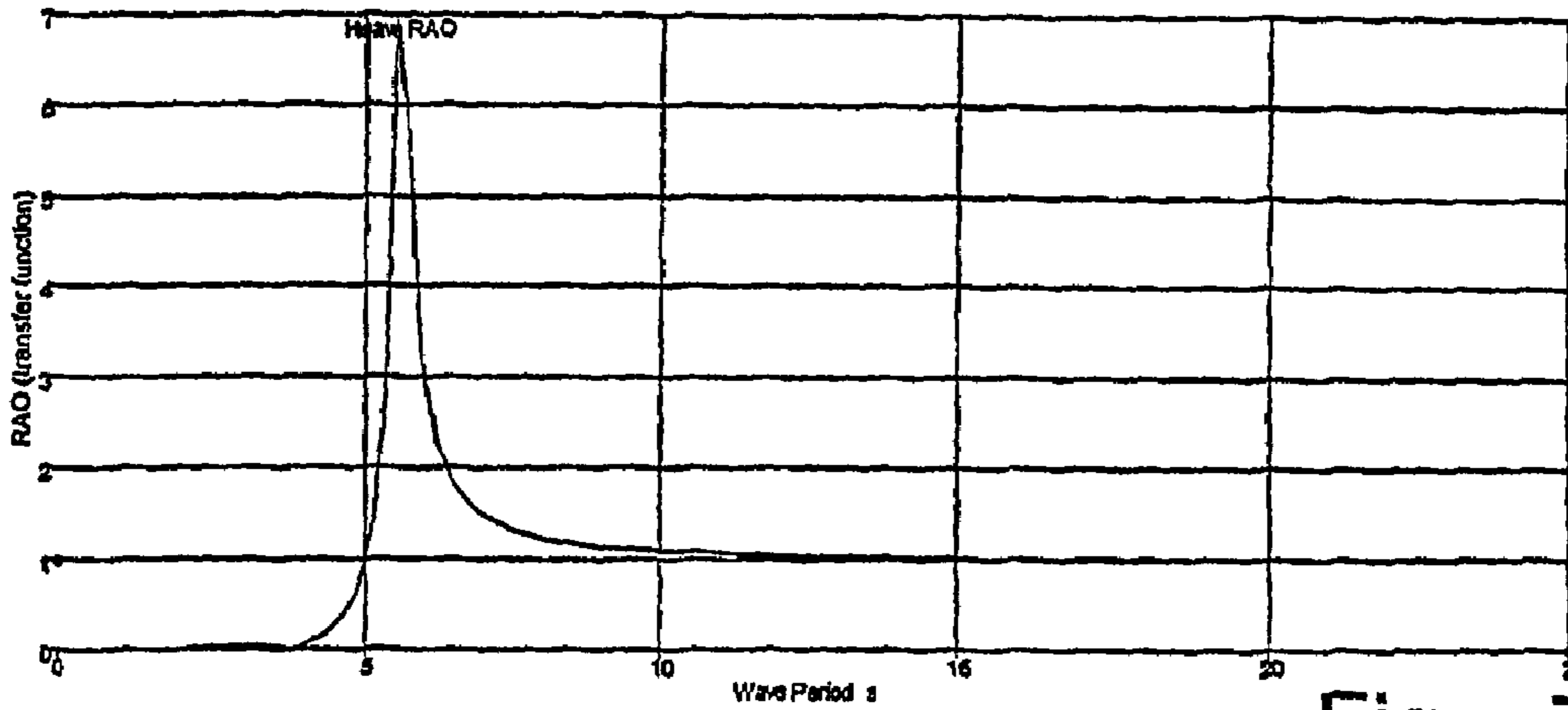
Egg Dia 3.5m Draught 4.5m
