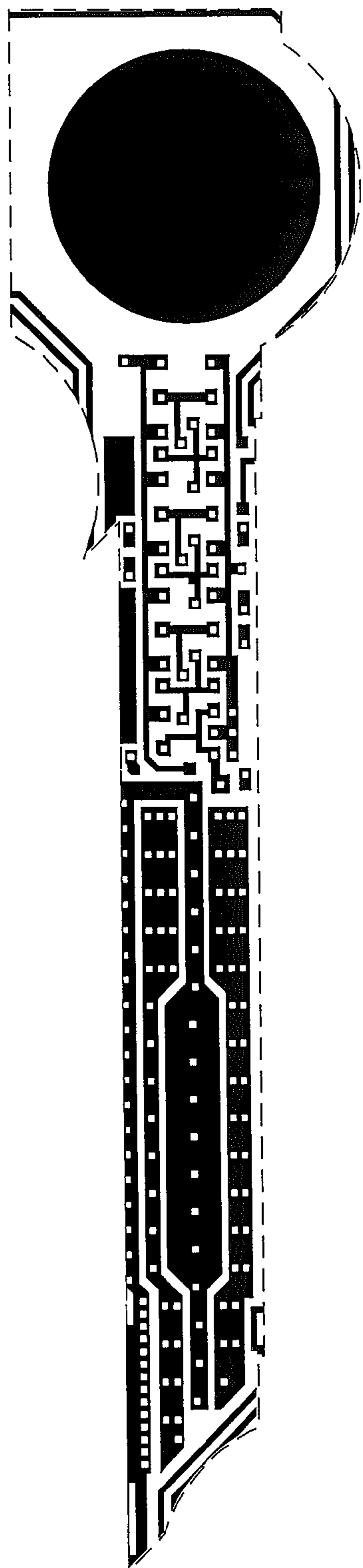
Metal 1 mask
