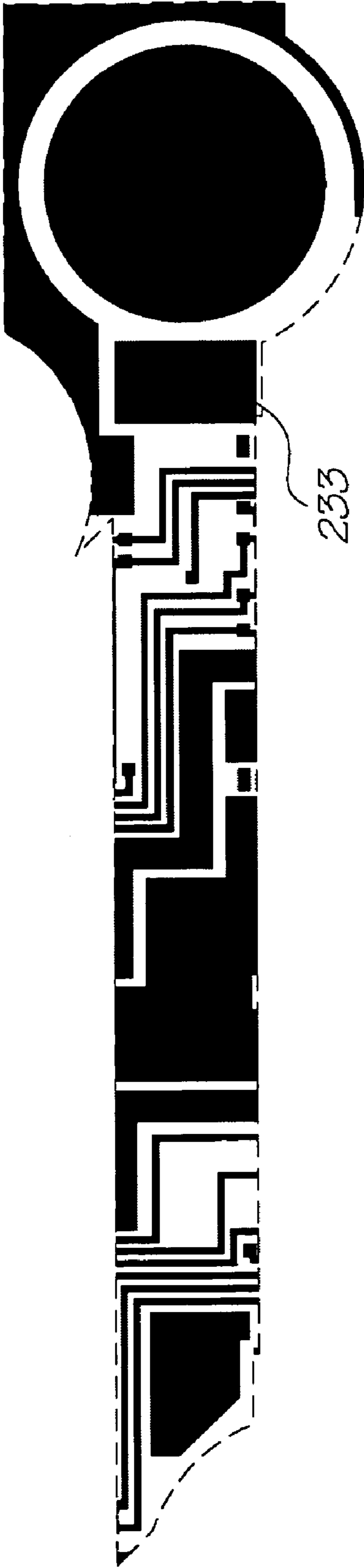
Metal 2 mask
