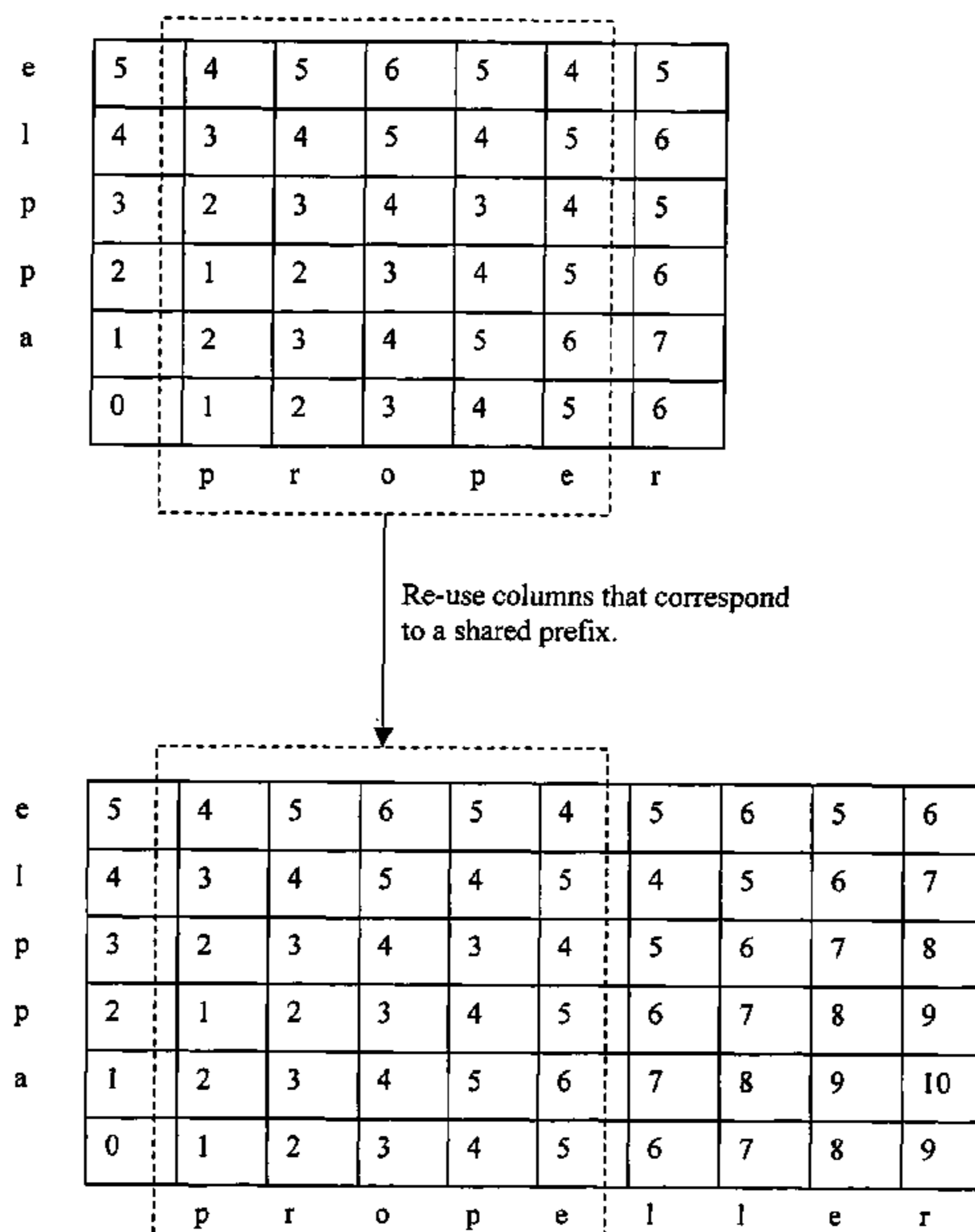
Re-Using Columns that Correspond to a Shared Prefix.
