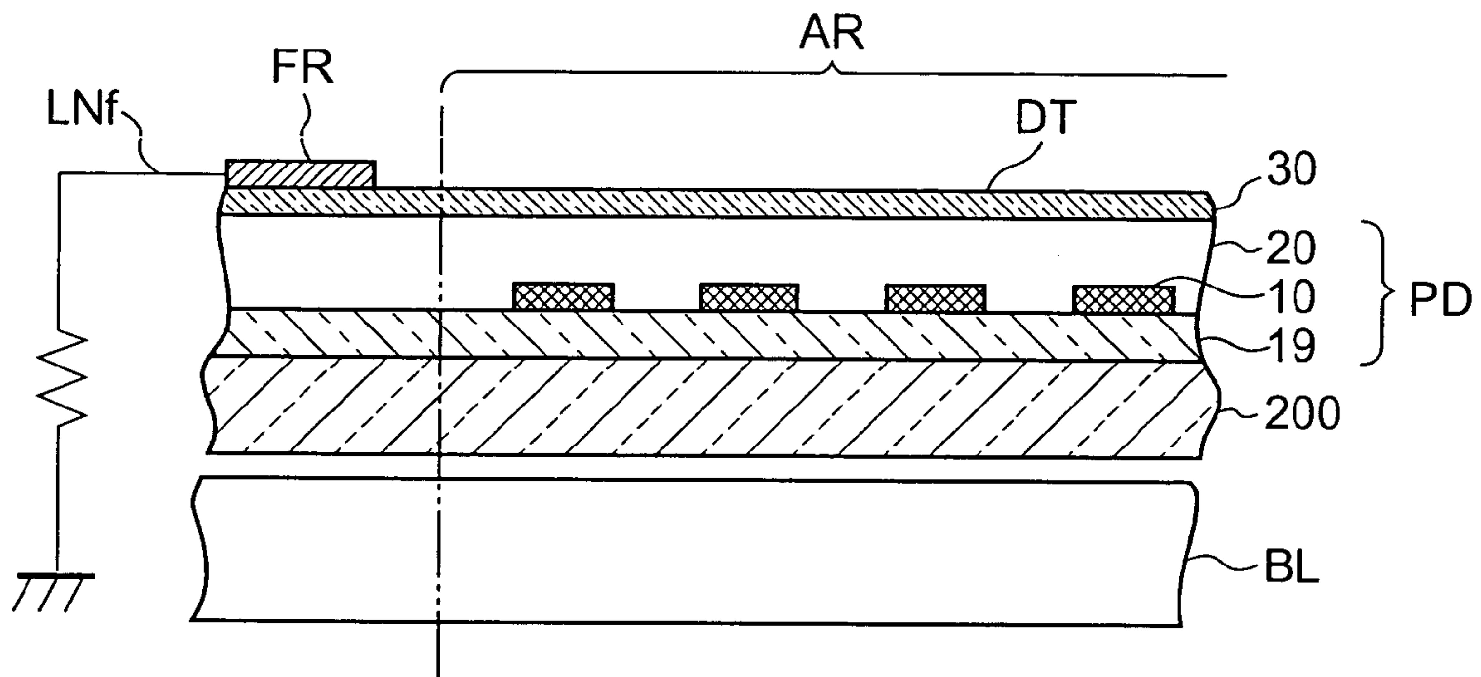
B-B PARTIAL CROSS SECTION
