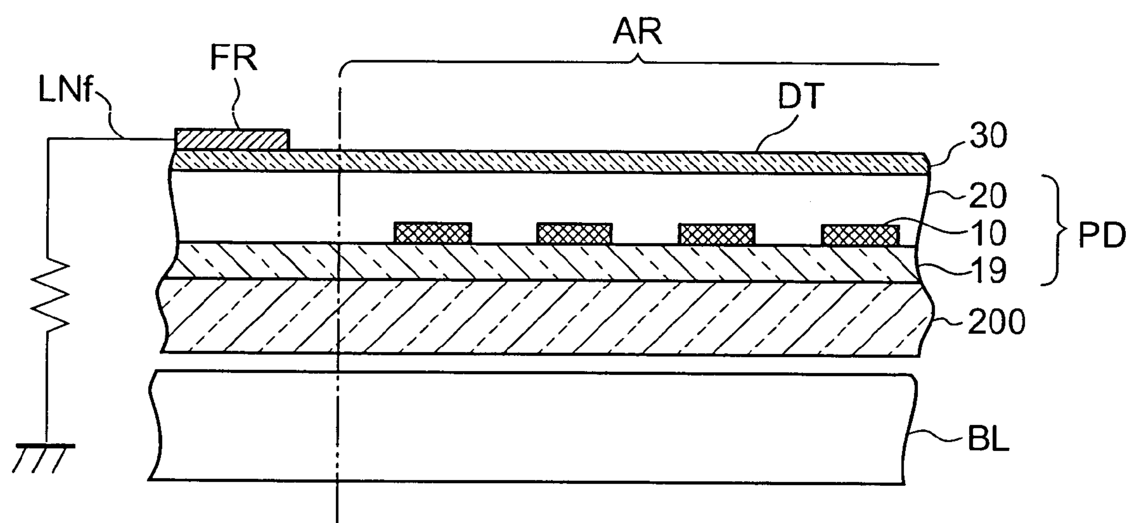
B-B PARTIAL CROSS SECTION
