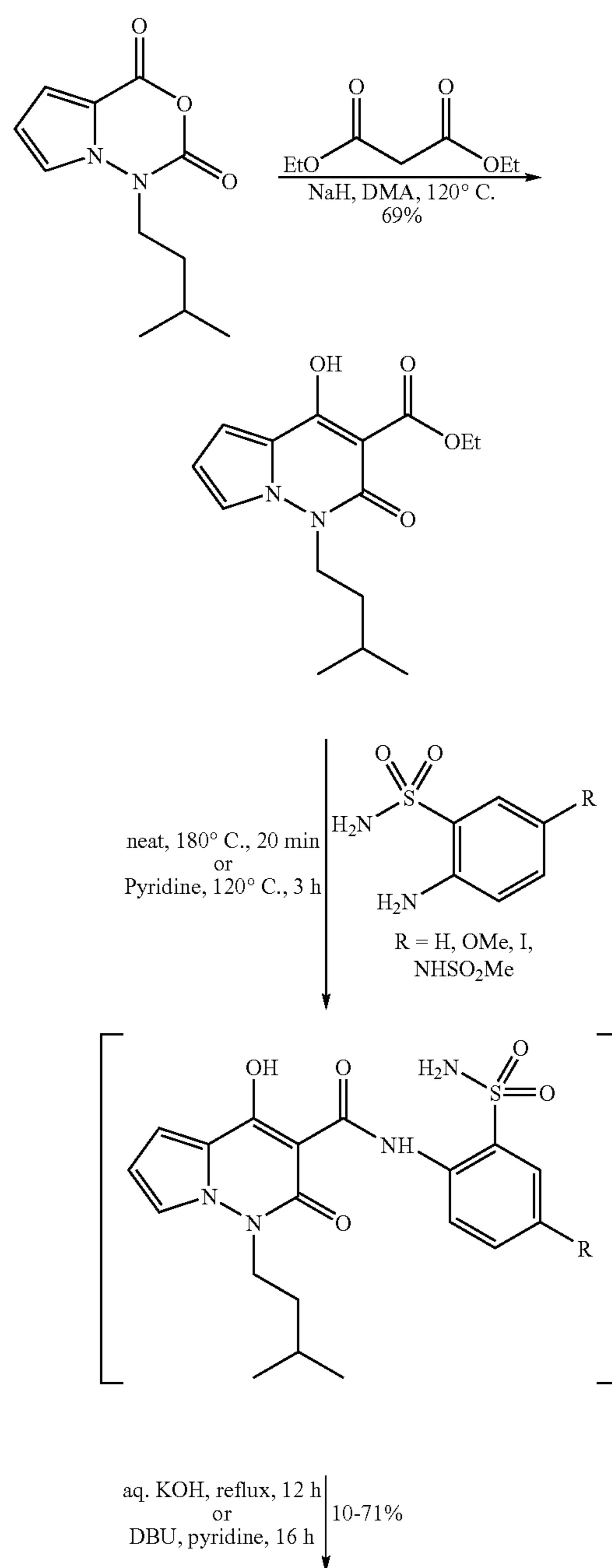
Scheme 1
