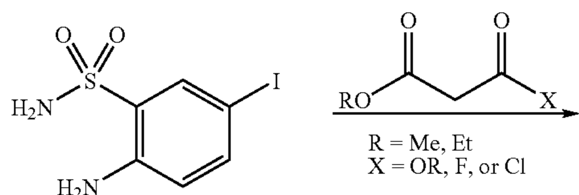
Scheme 17
