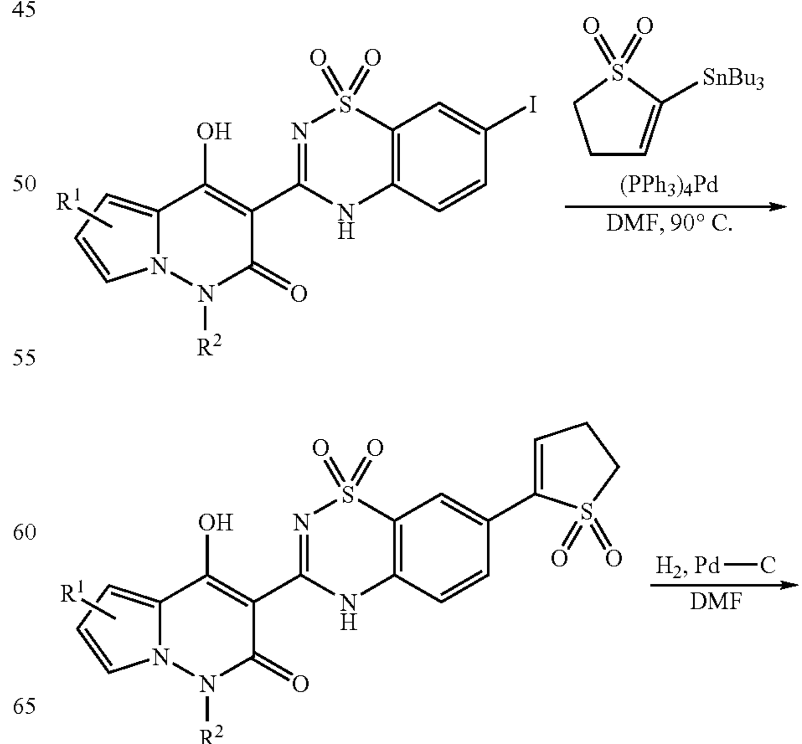
Scheme 19
