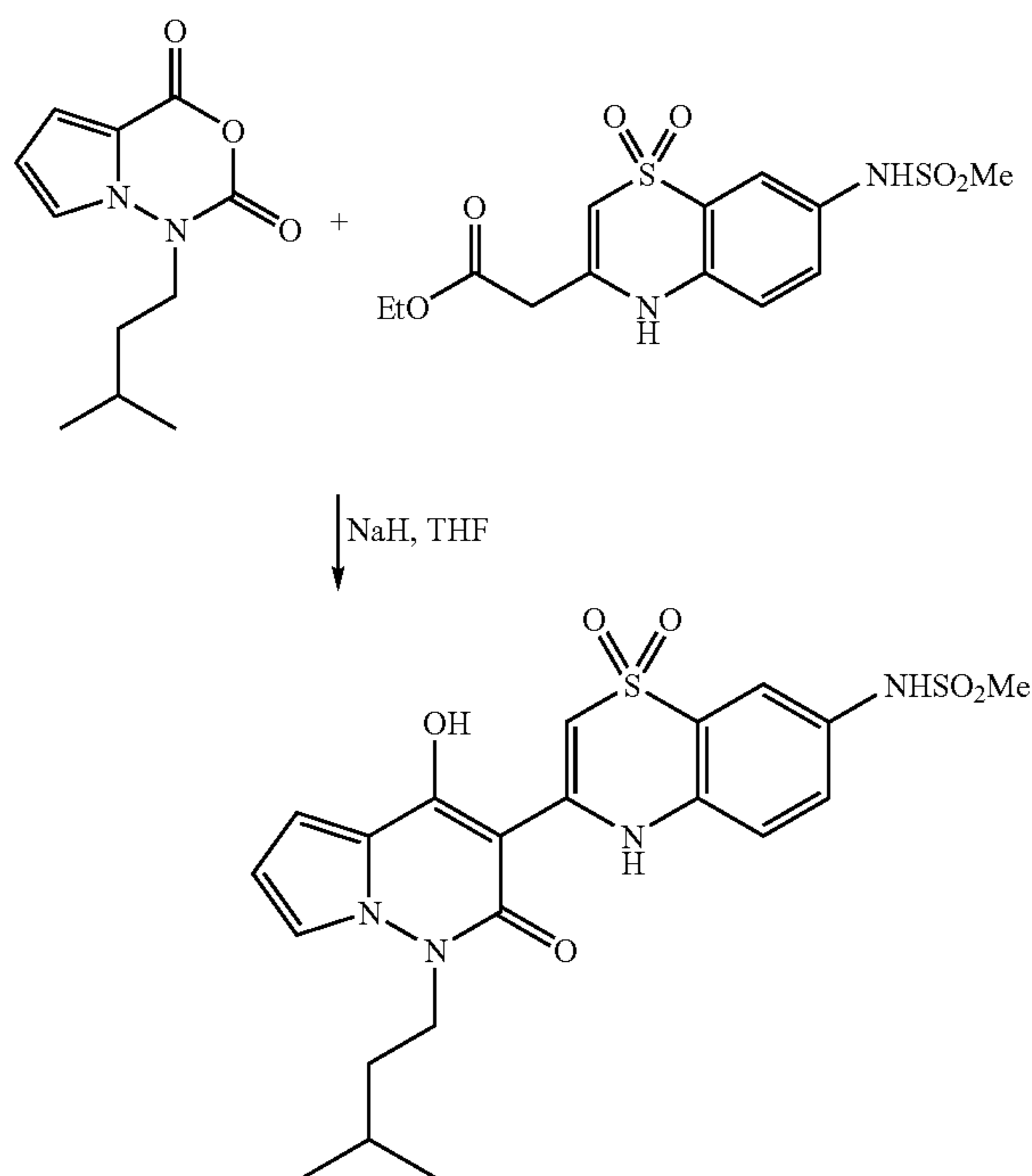
Scheme 20
