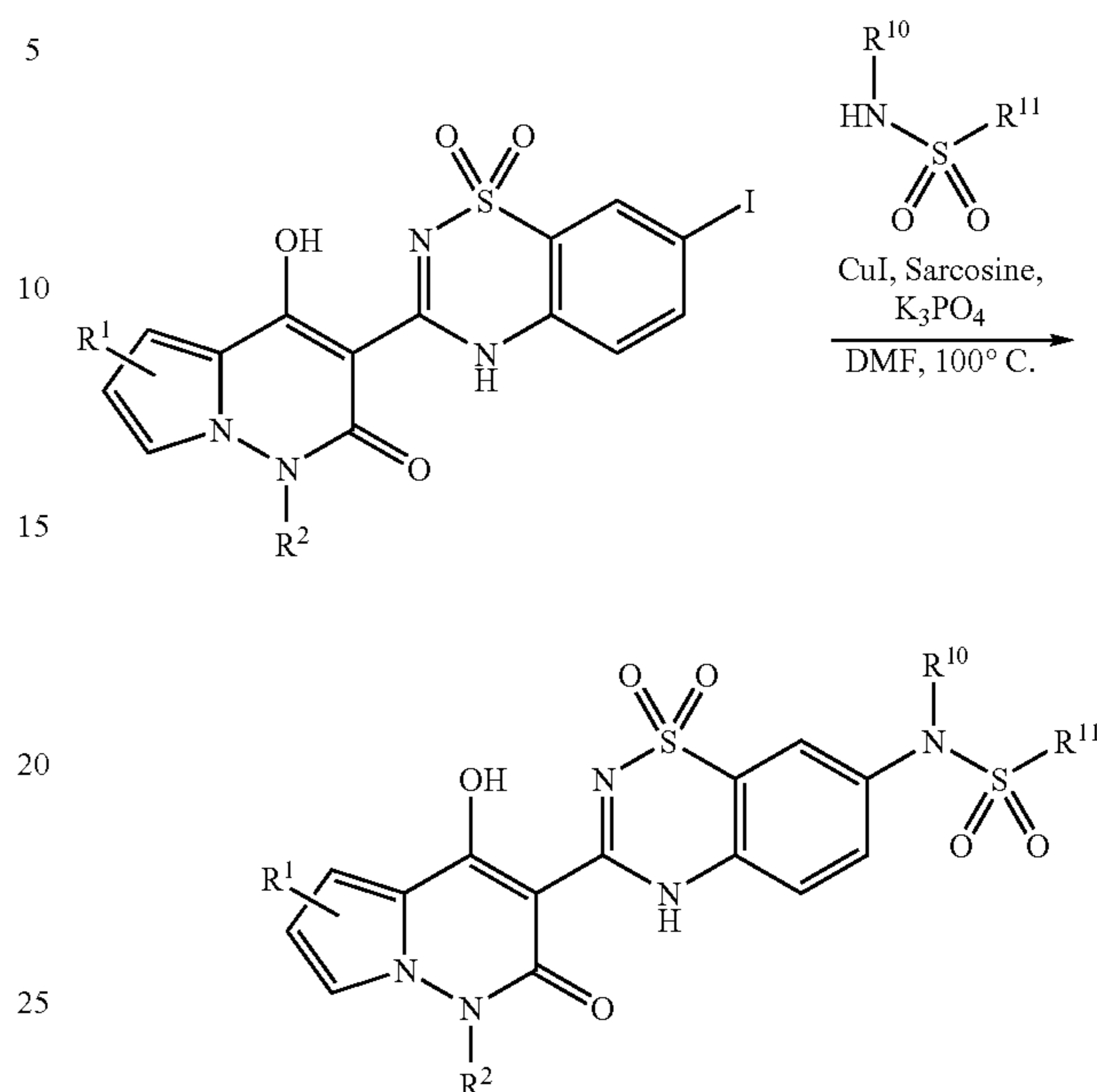
Scheme 18
