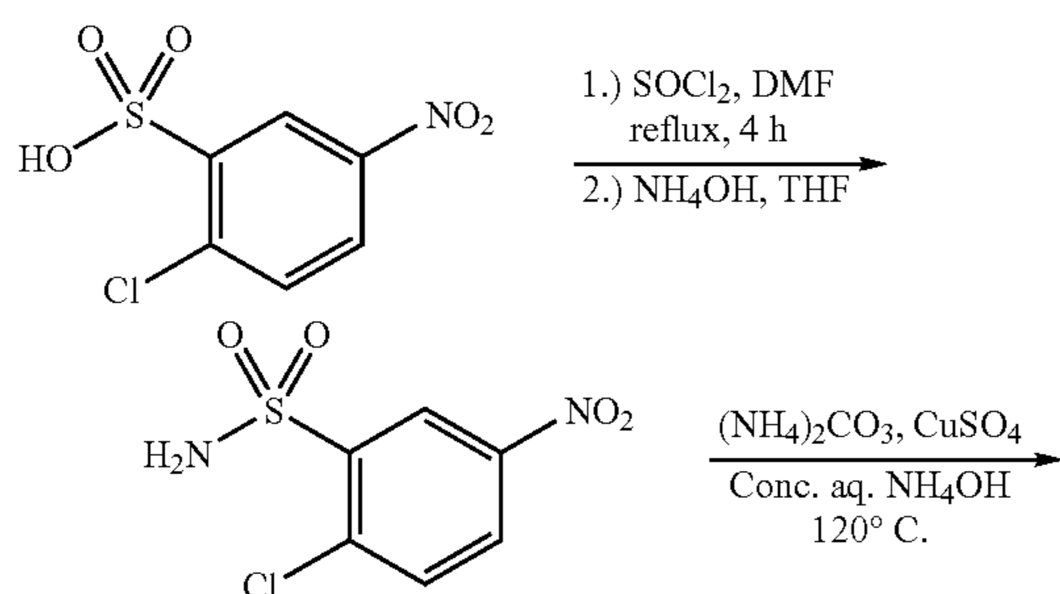
Scheme 11
