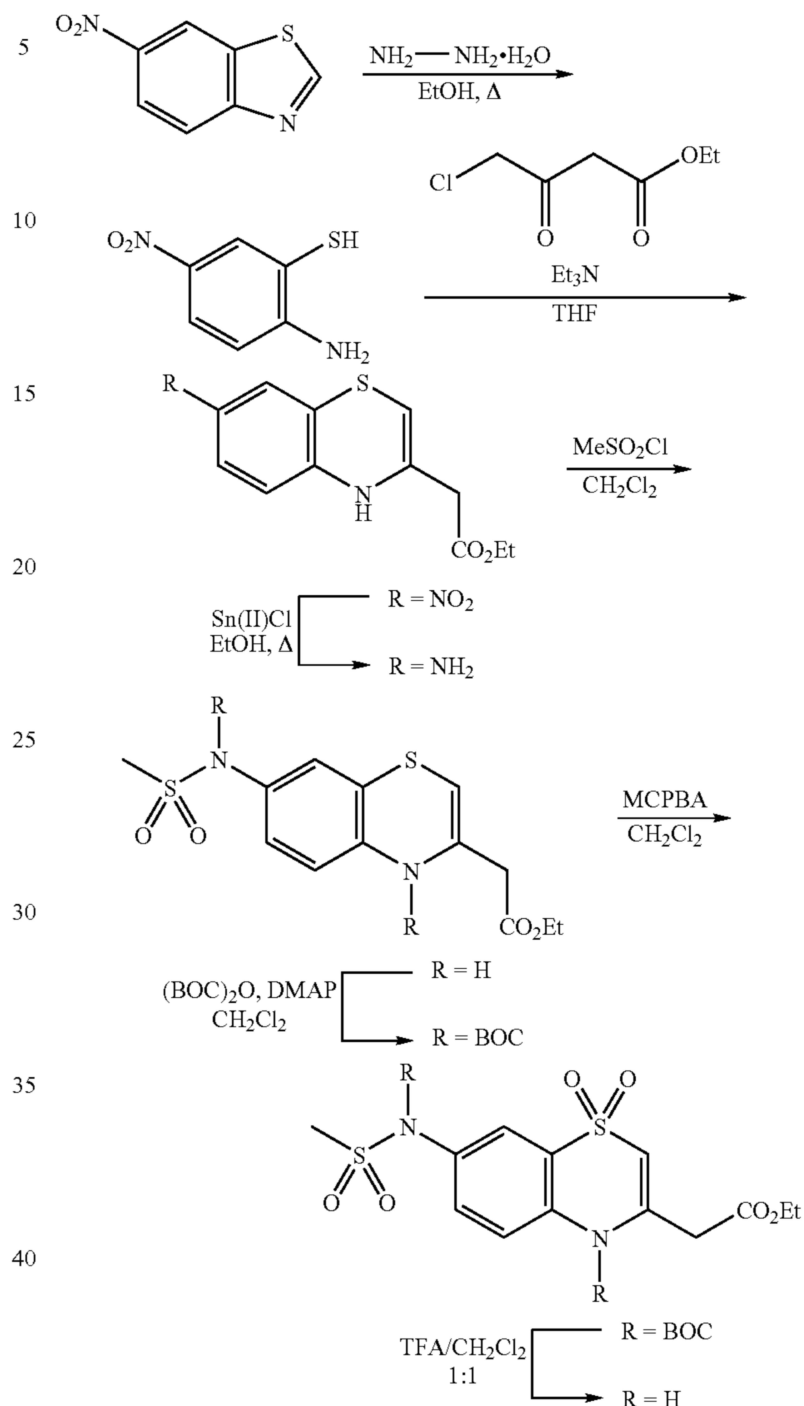
Scheme 21
