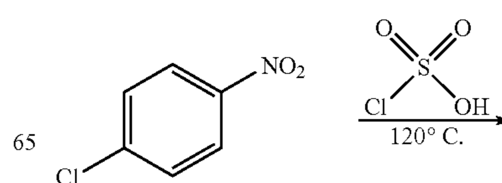
Scheme 12
