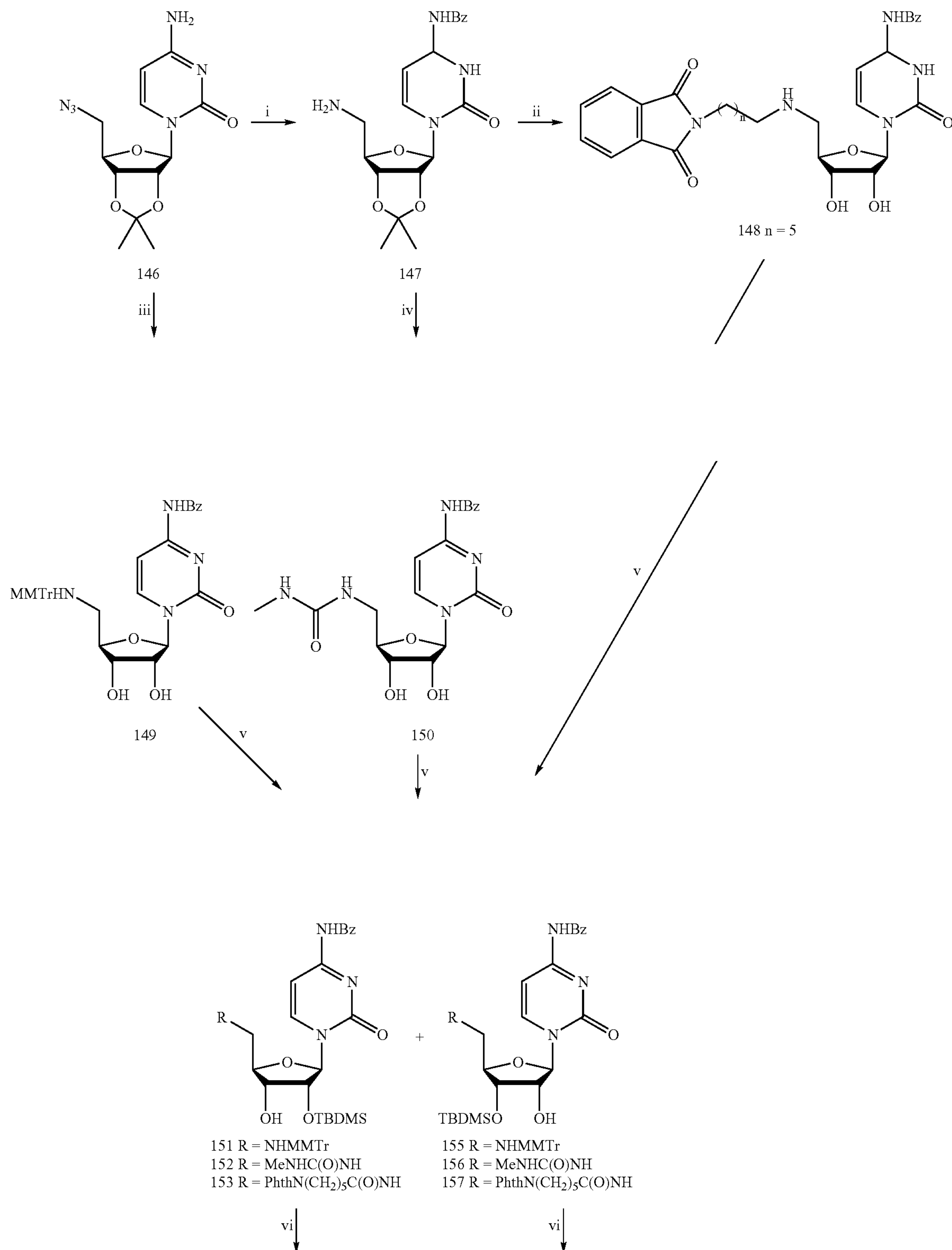
Scheme 7 a
