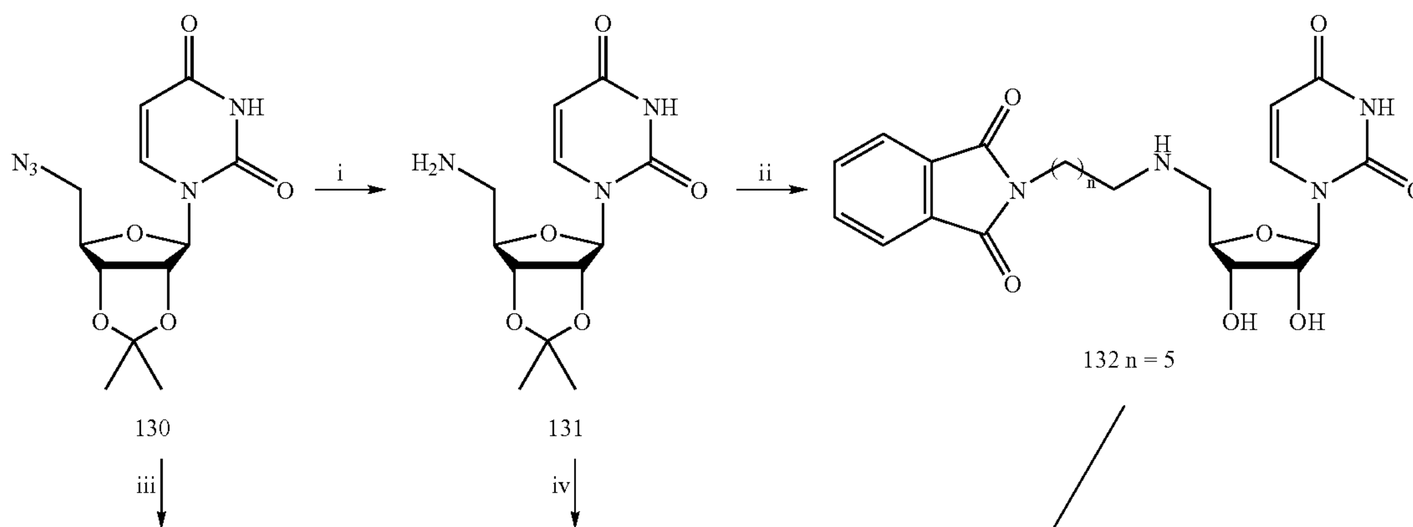
Scheme 6 a
