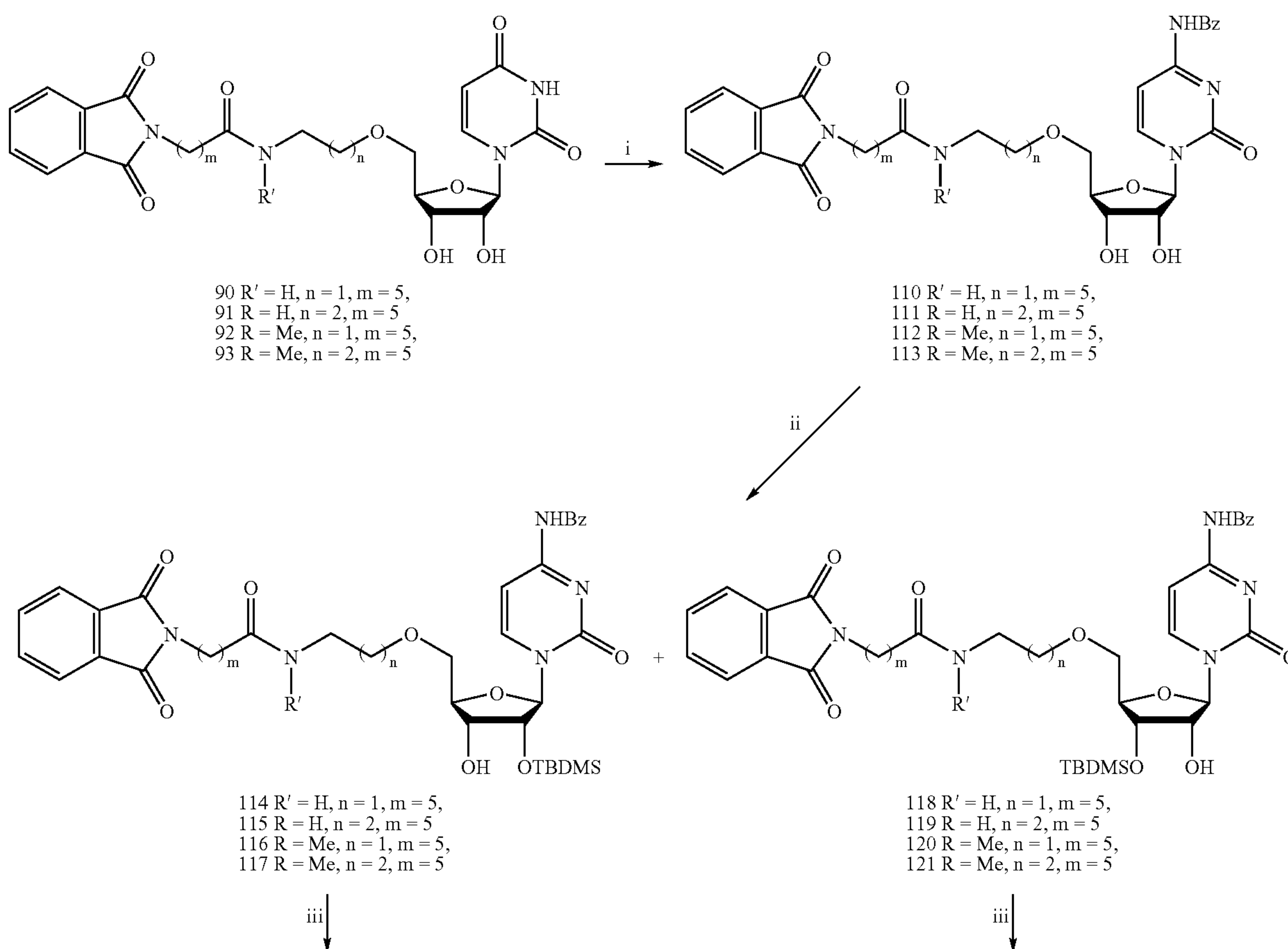
Scheme 5 a
