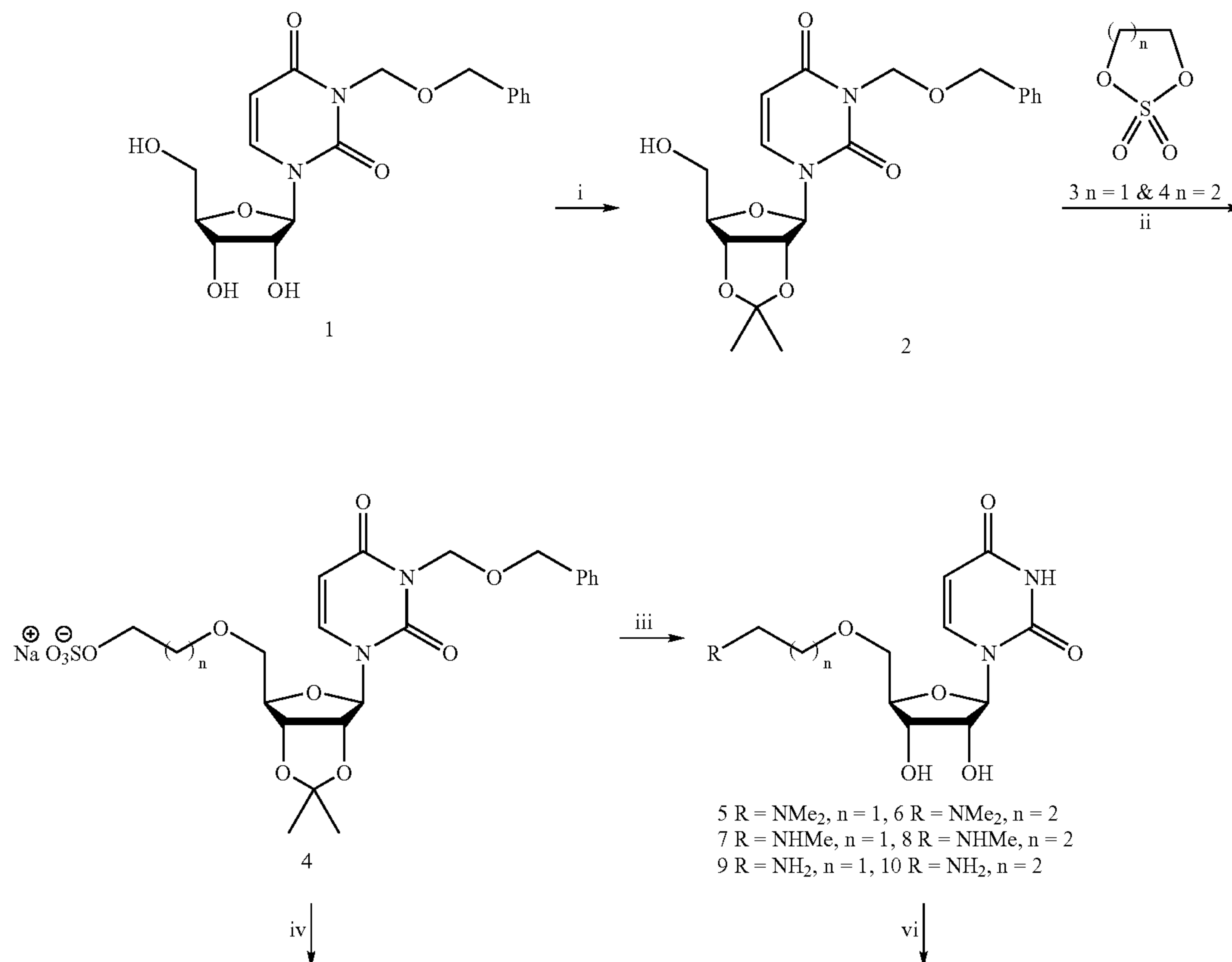
Scheme 1 a
