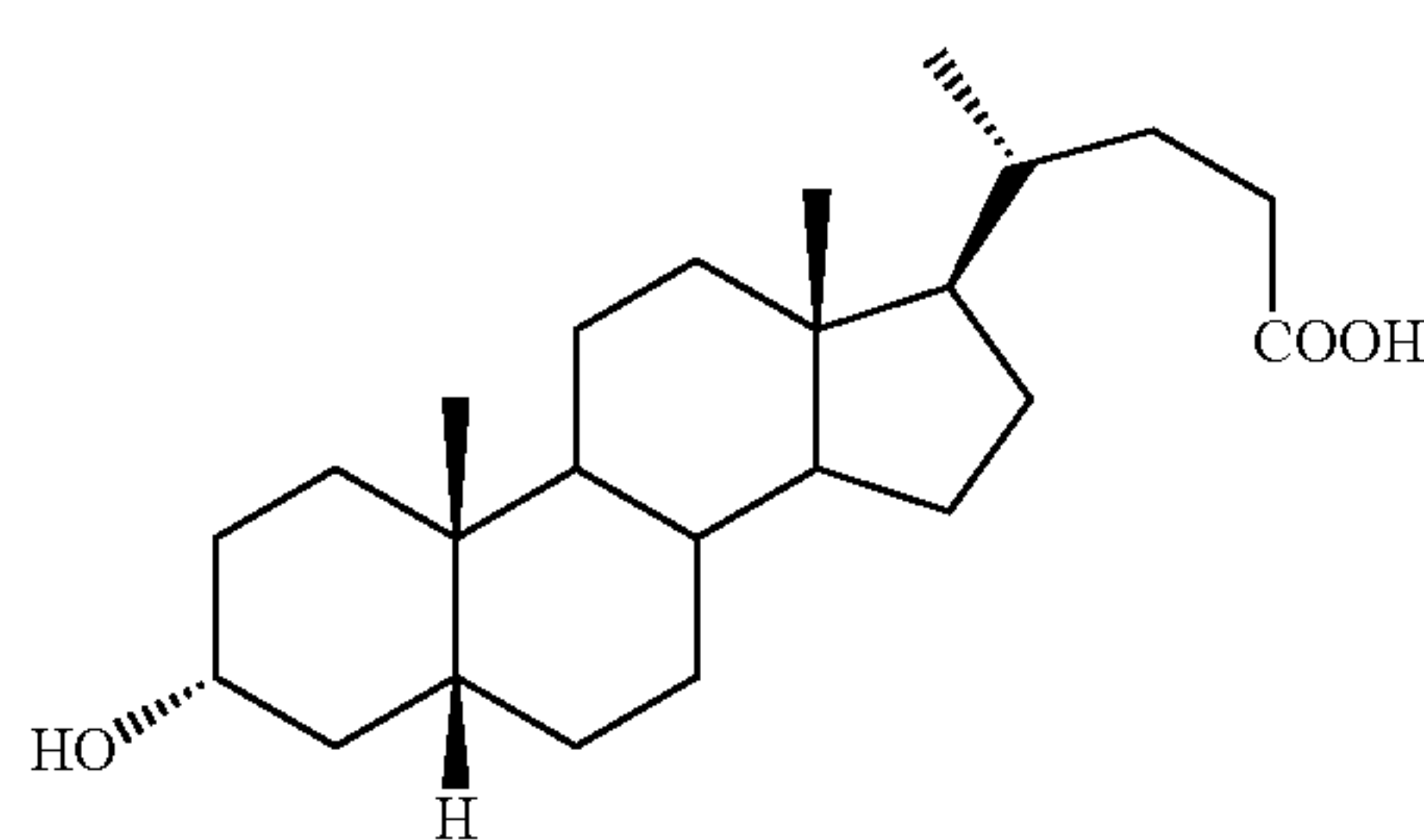
Lithocholic acid
