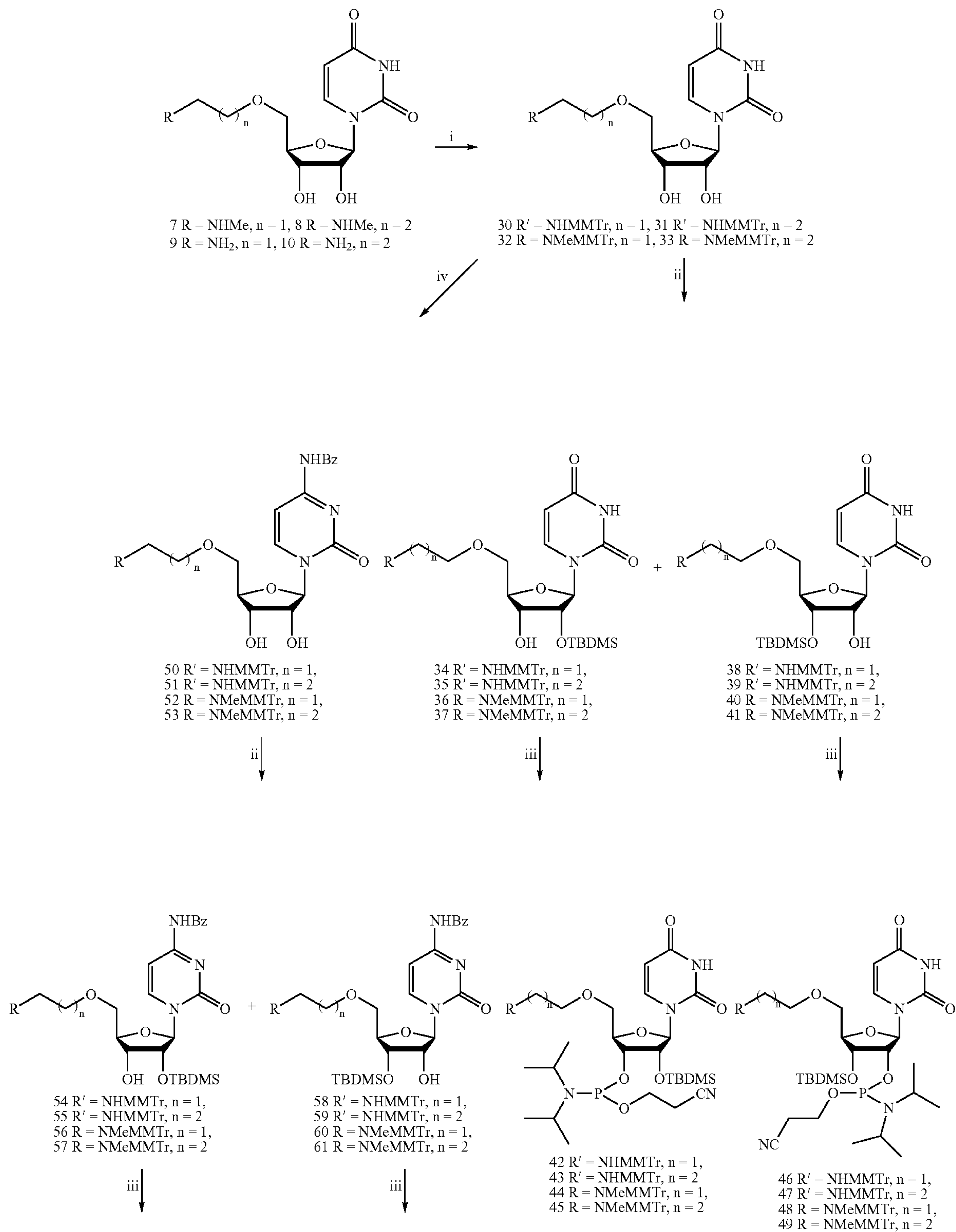
Scheme 2 a
