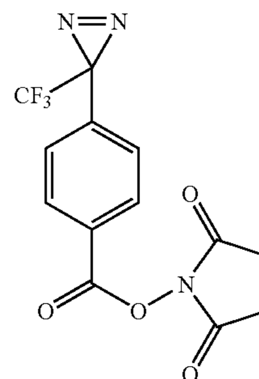
diazirine compound D
