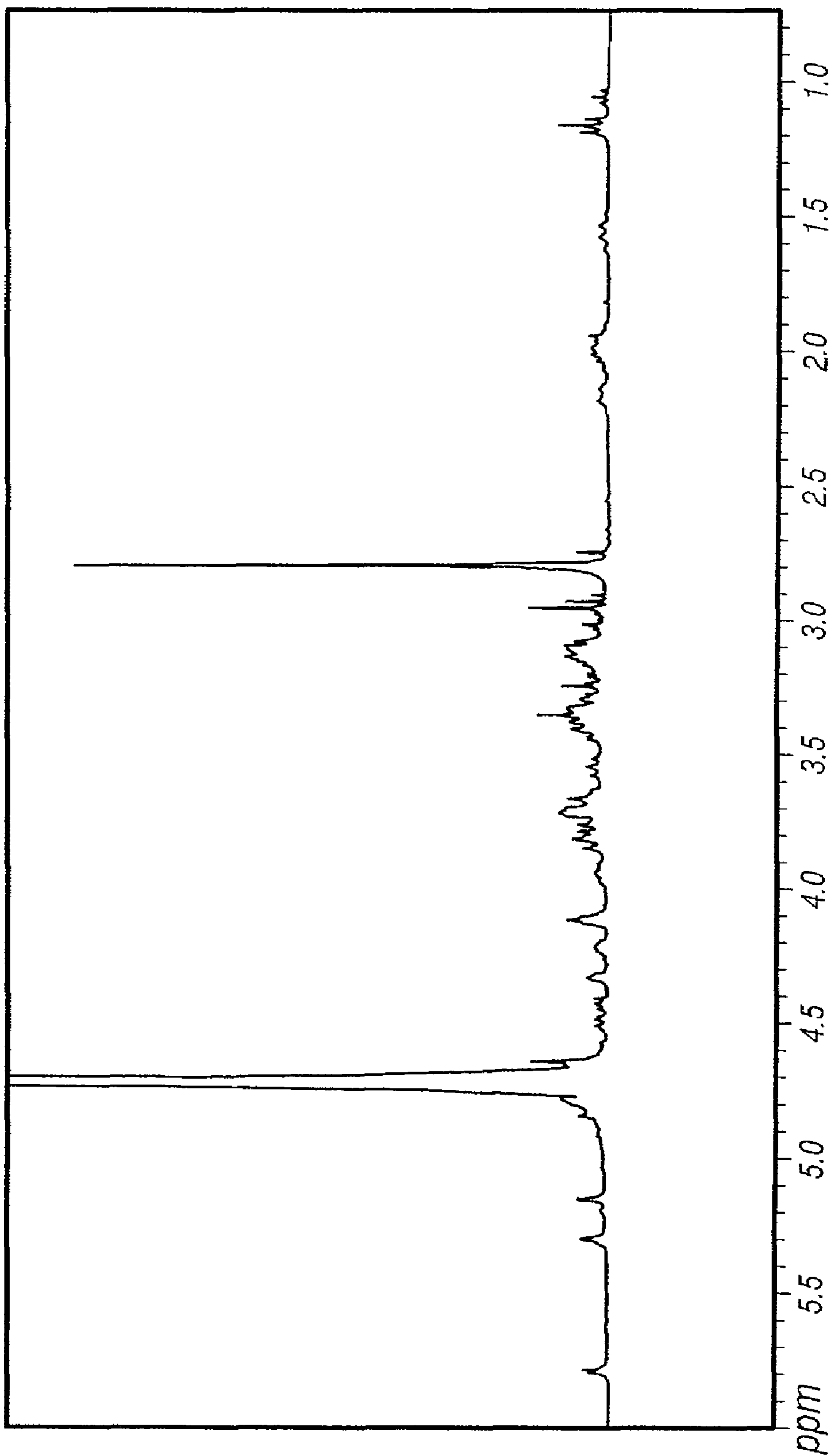
1 H-NMR of EC-neomycin
