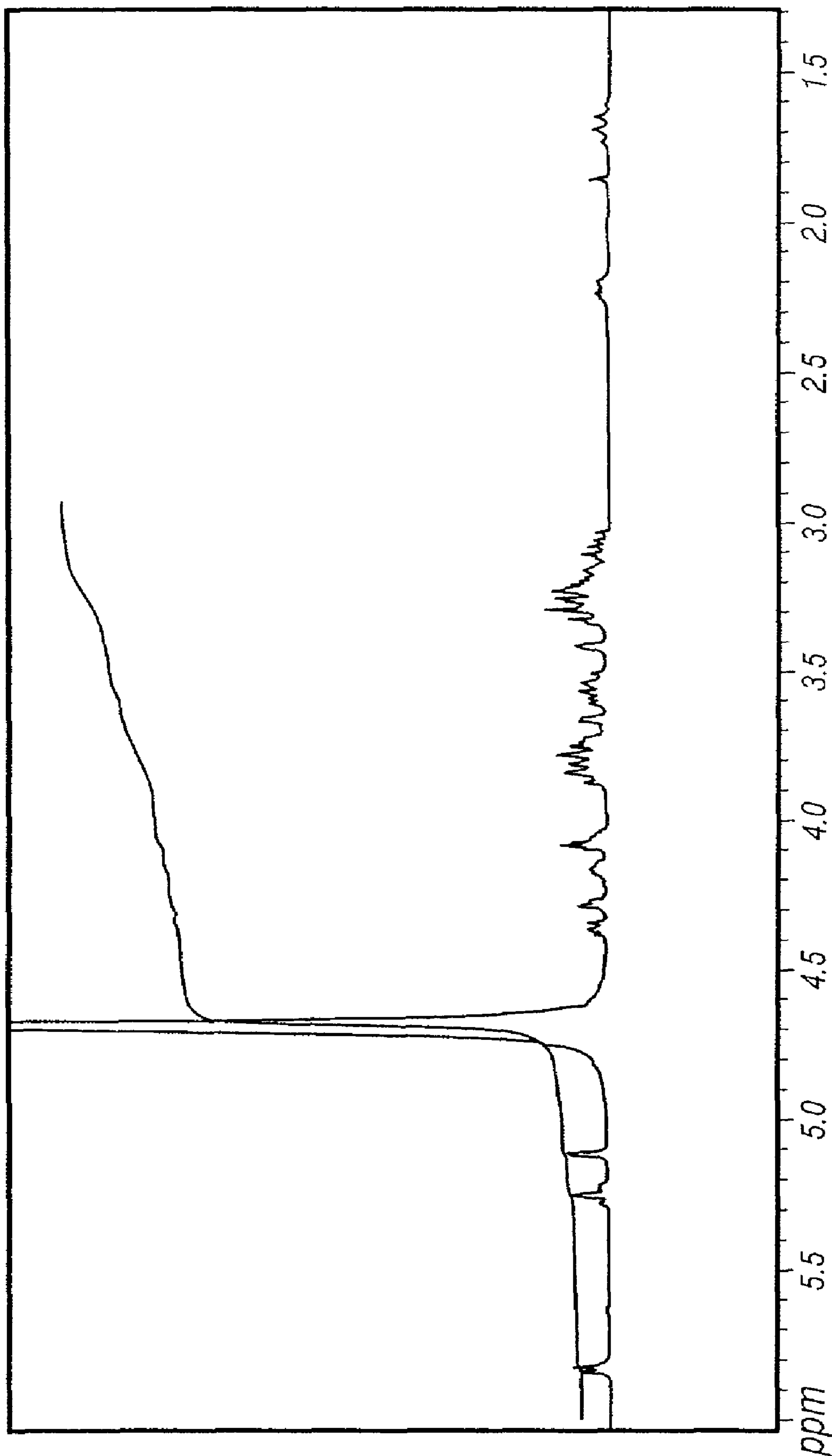
1 H-NMR of neomycin
