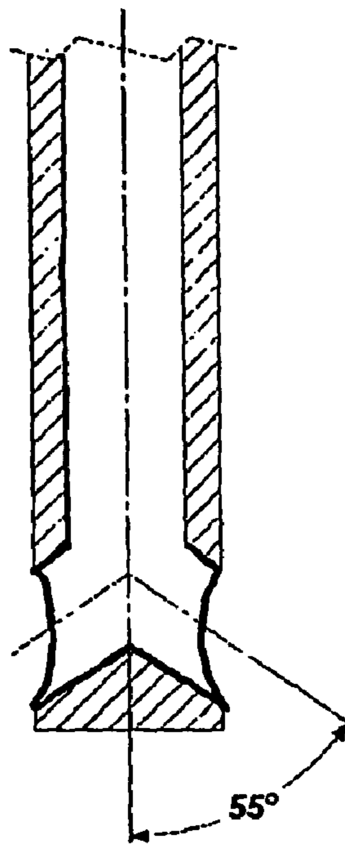
Fig. 3 PRIOR ART
