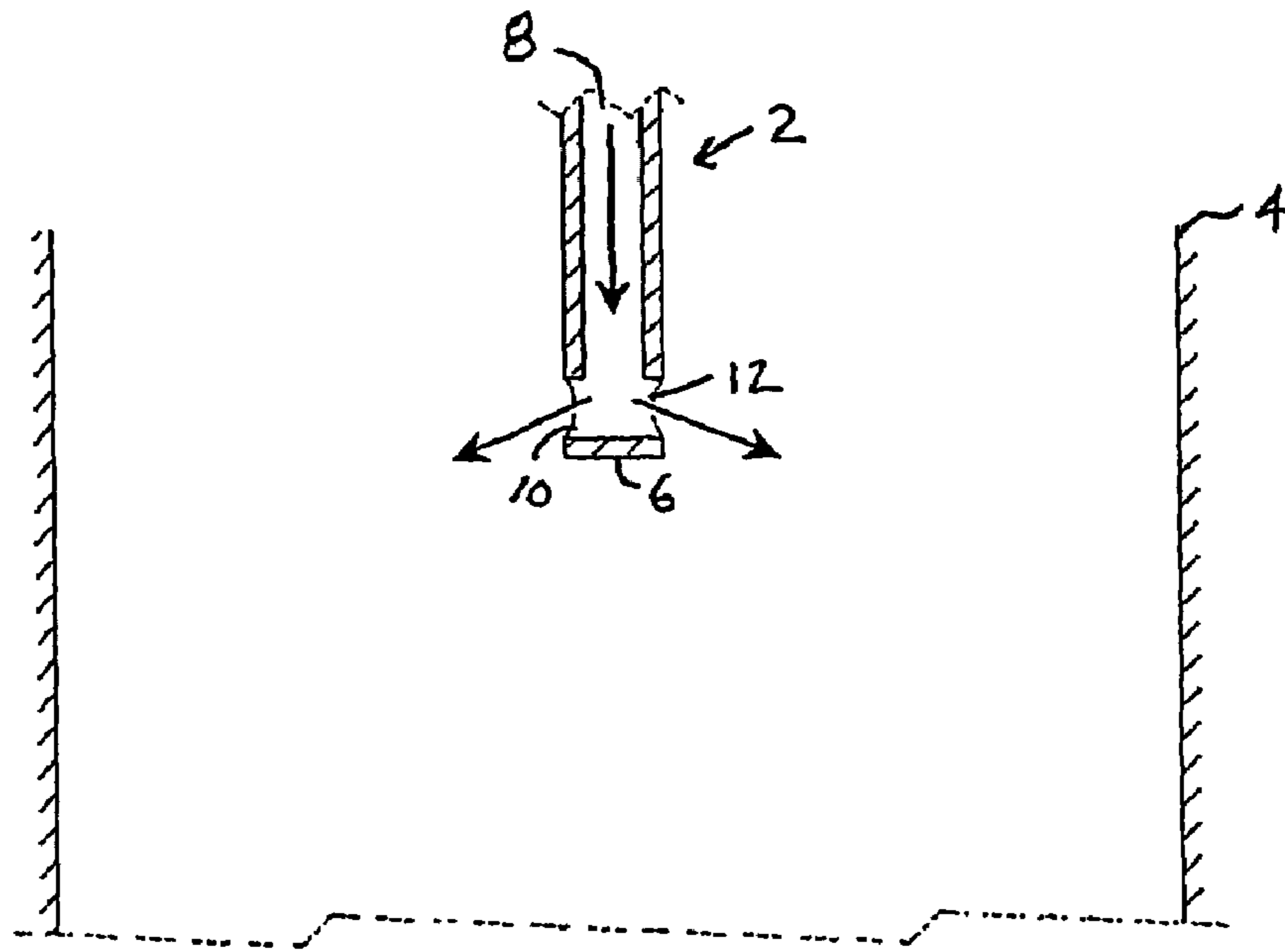
Fig. 1 PRIOR ART
