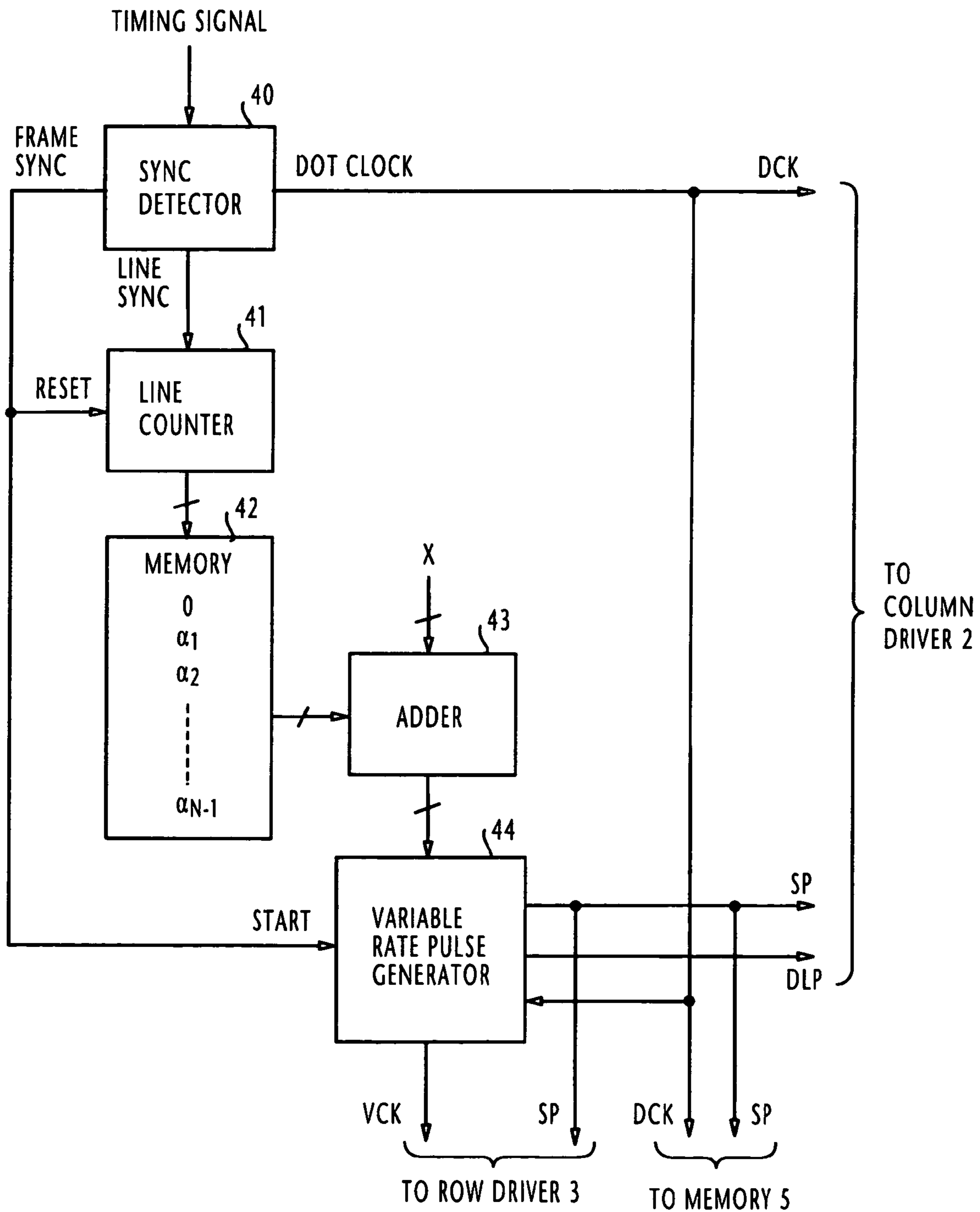
TIMING CONTROLLER
