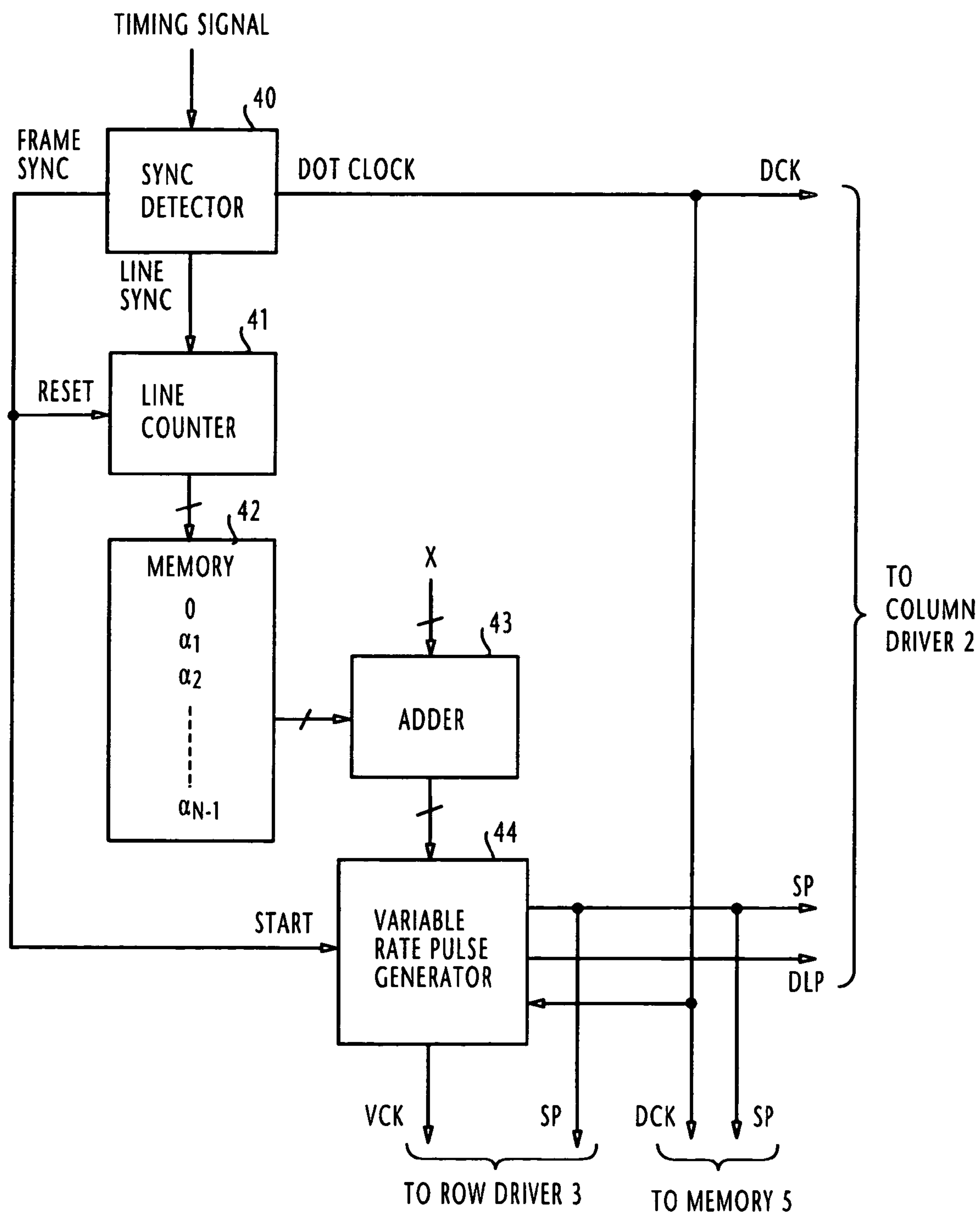
TIMING CONTROLLER
