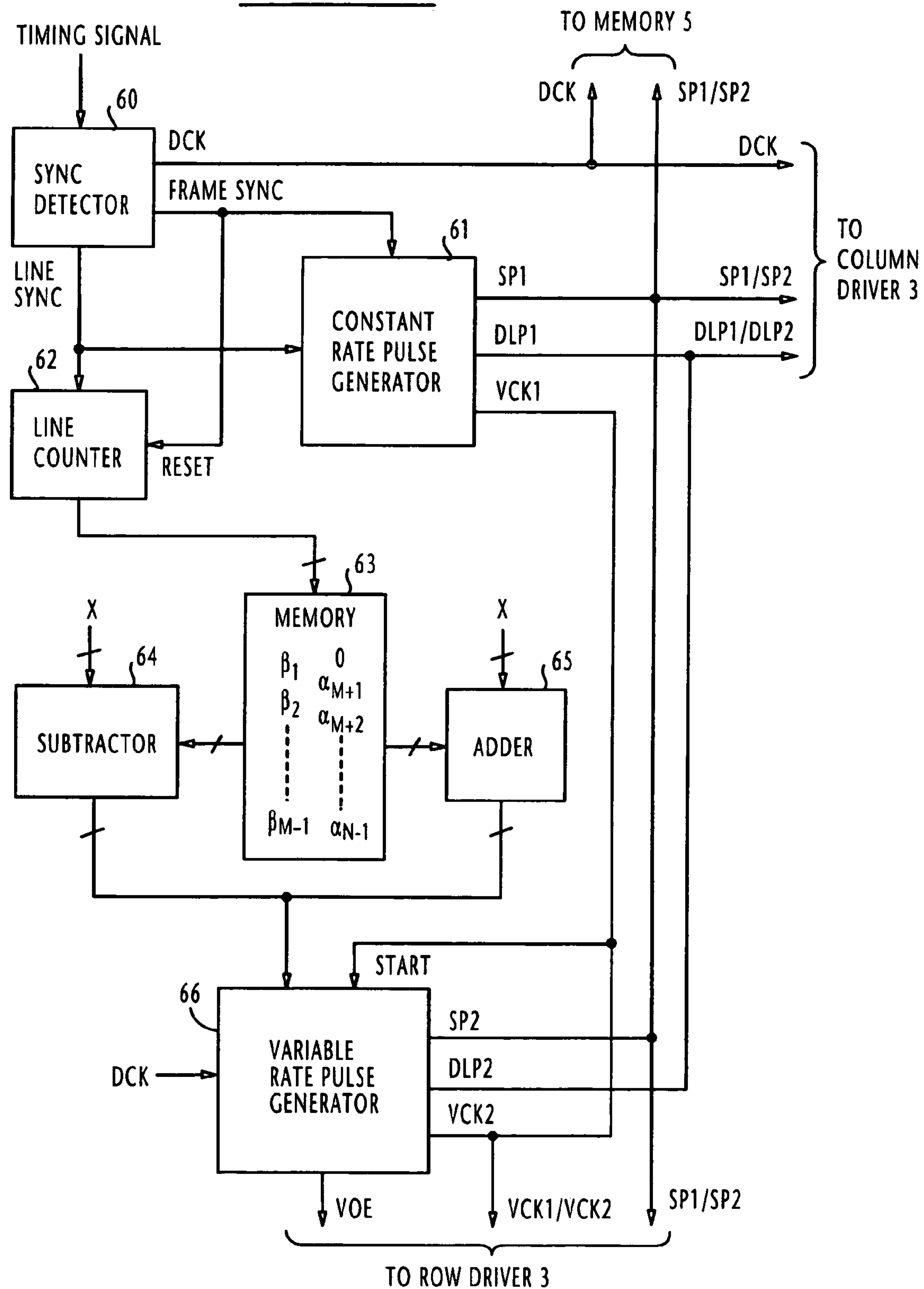
TIMING CONTROLLER
